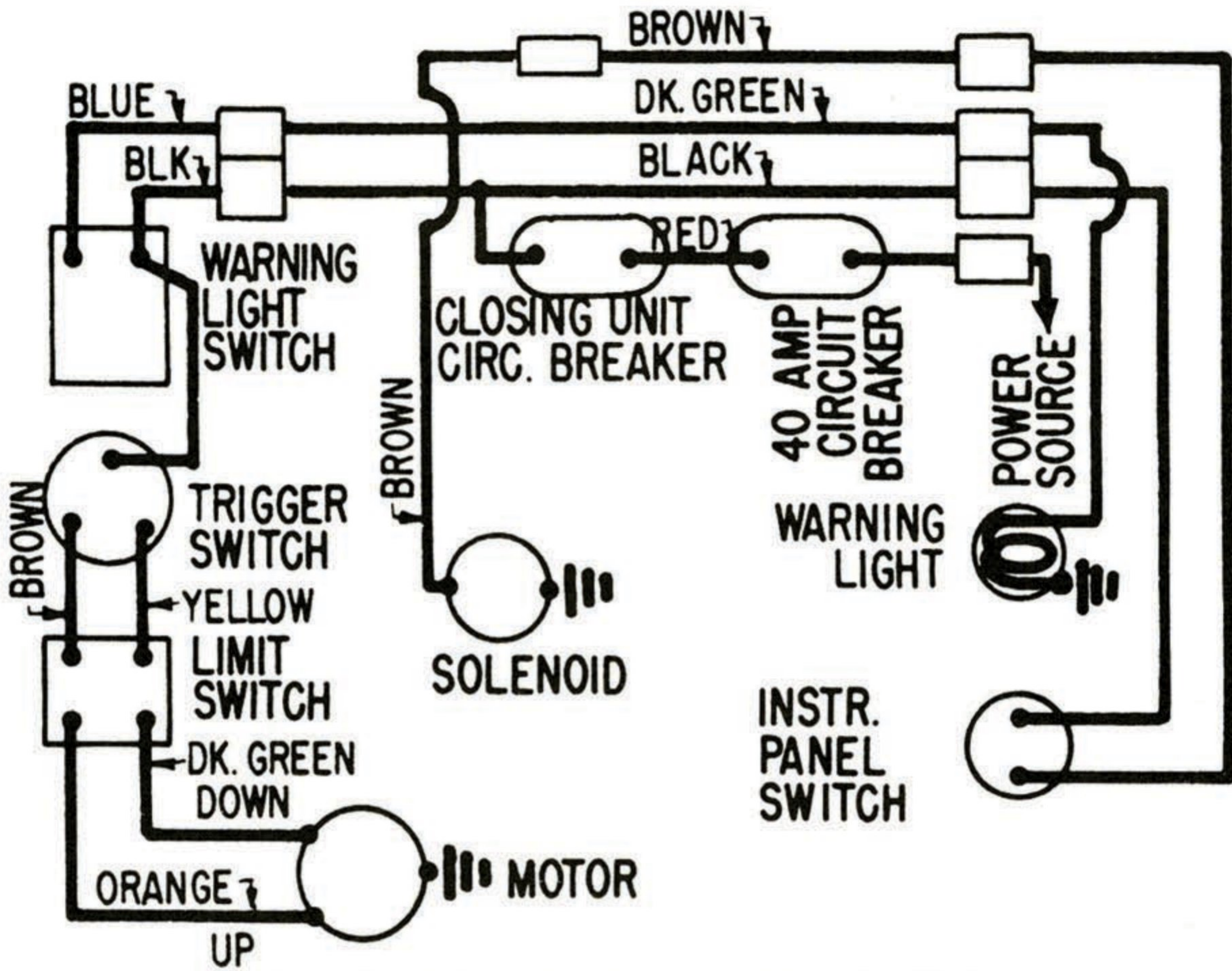
CADILLAC TRUNK LOCK DIAGRAM
