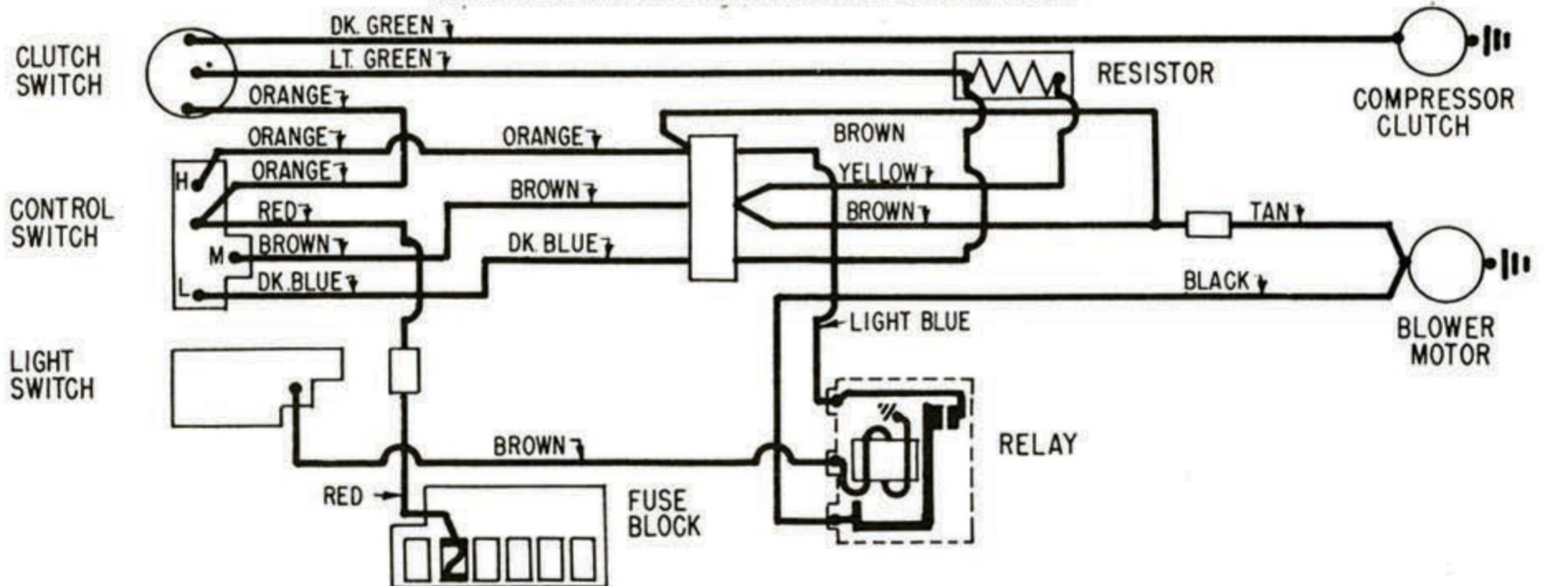
CHEVROLET AIR CONDITIONING CONTROL DIAGRAM
