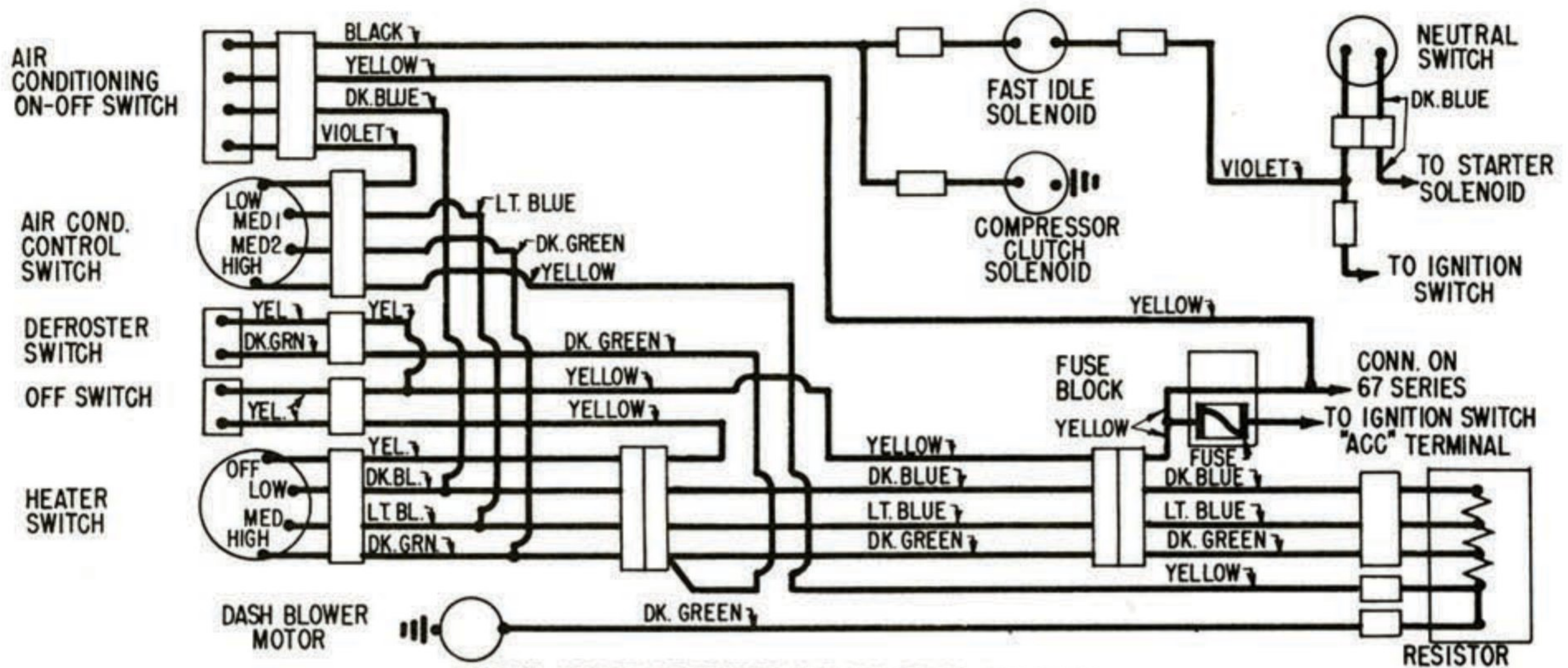
CADILLAC AIR CONDITIONING CONTROL DIAGRAM
