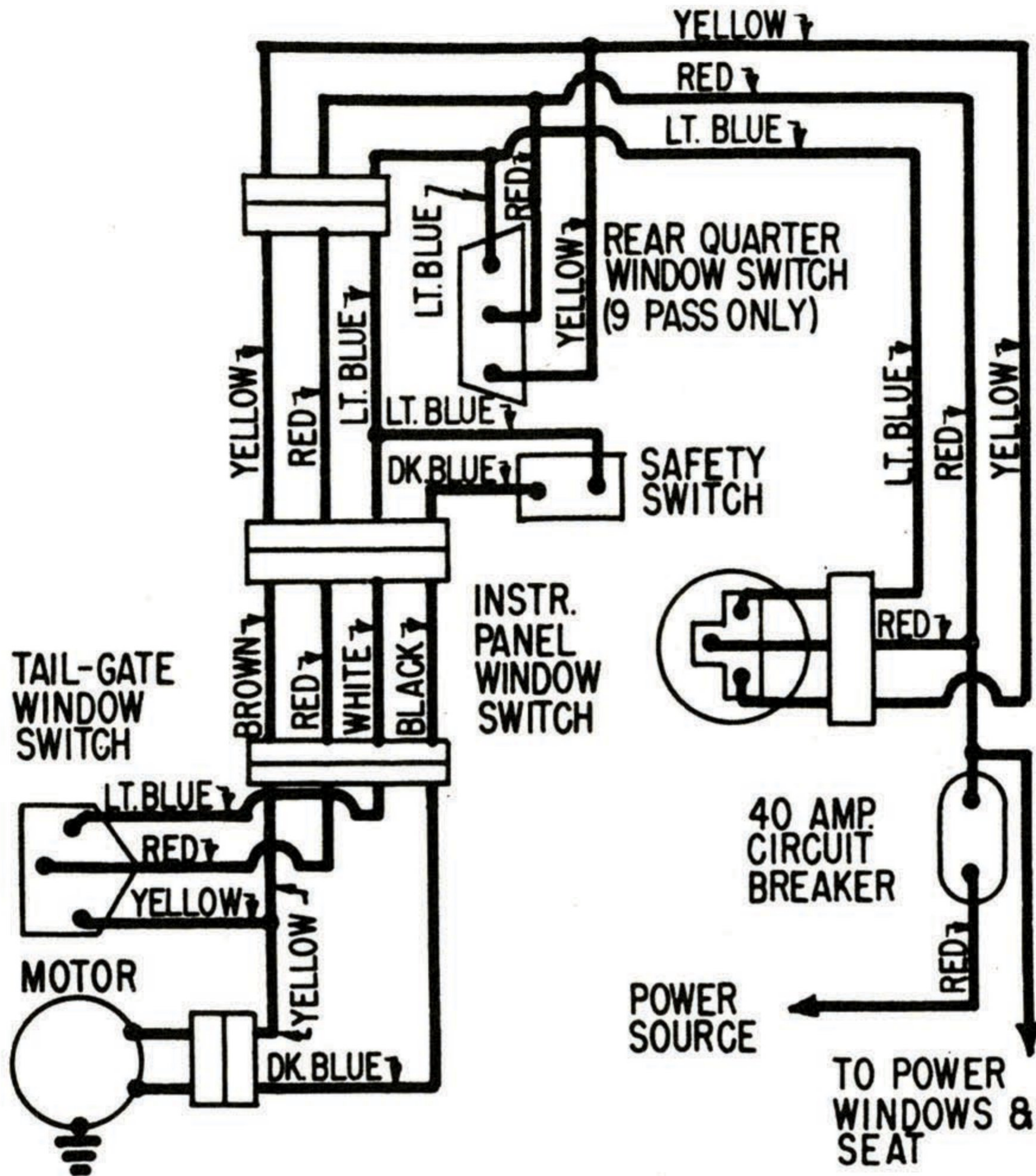
CHEVROLET REAR WINDOW CONTROL
