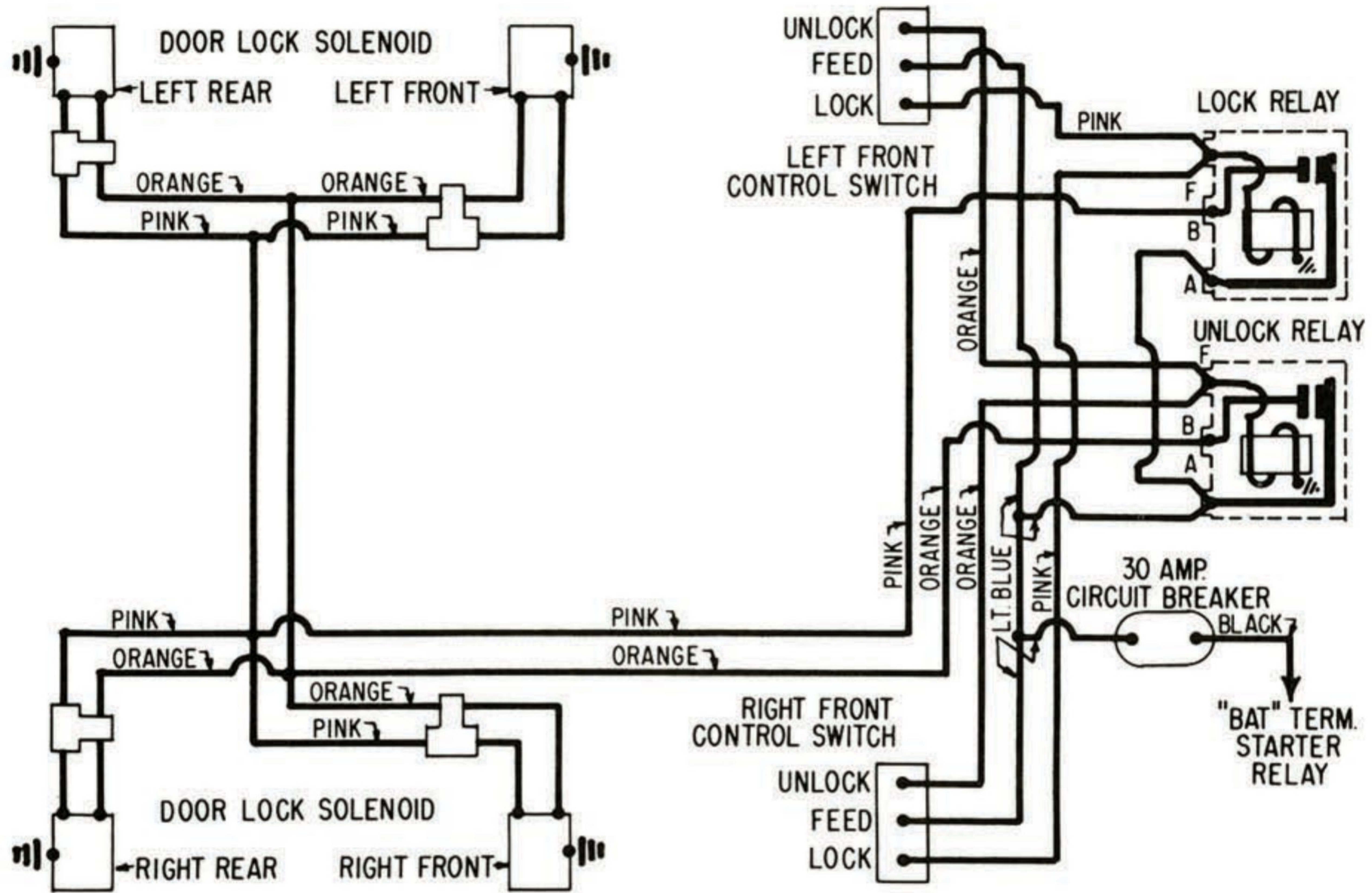
CHRYSLER IMPERIAL DOOR LOCK DIAGRAM
