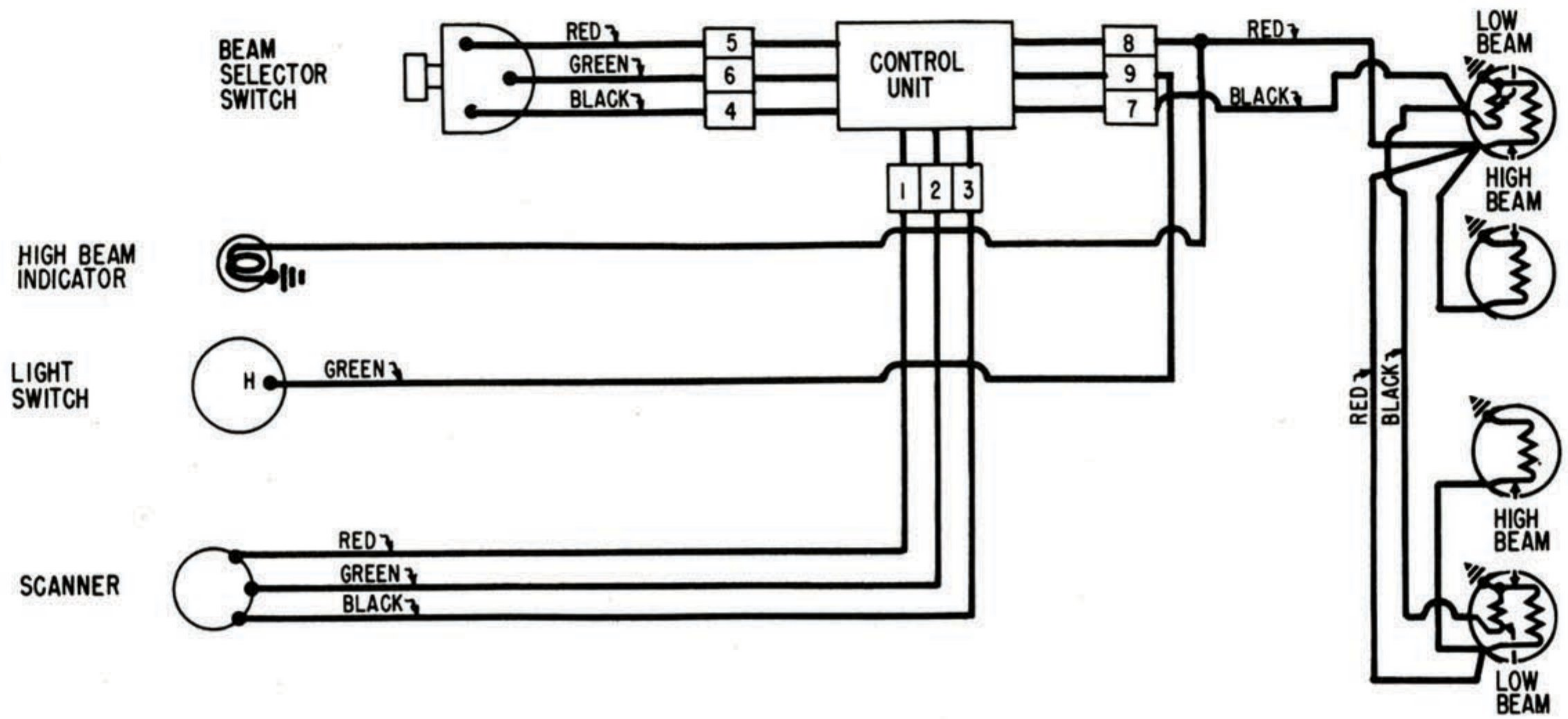
AUTOMATIC DIMMER WIRING DIAGRAM
