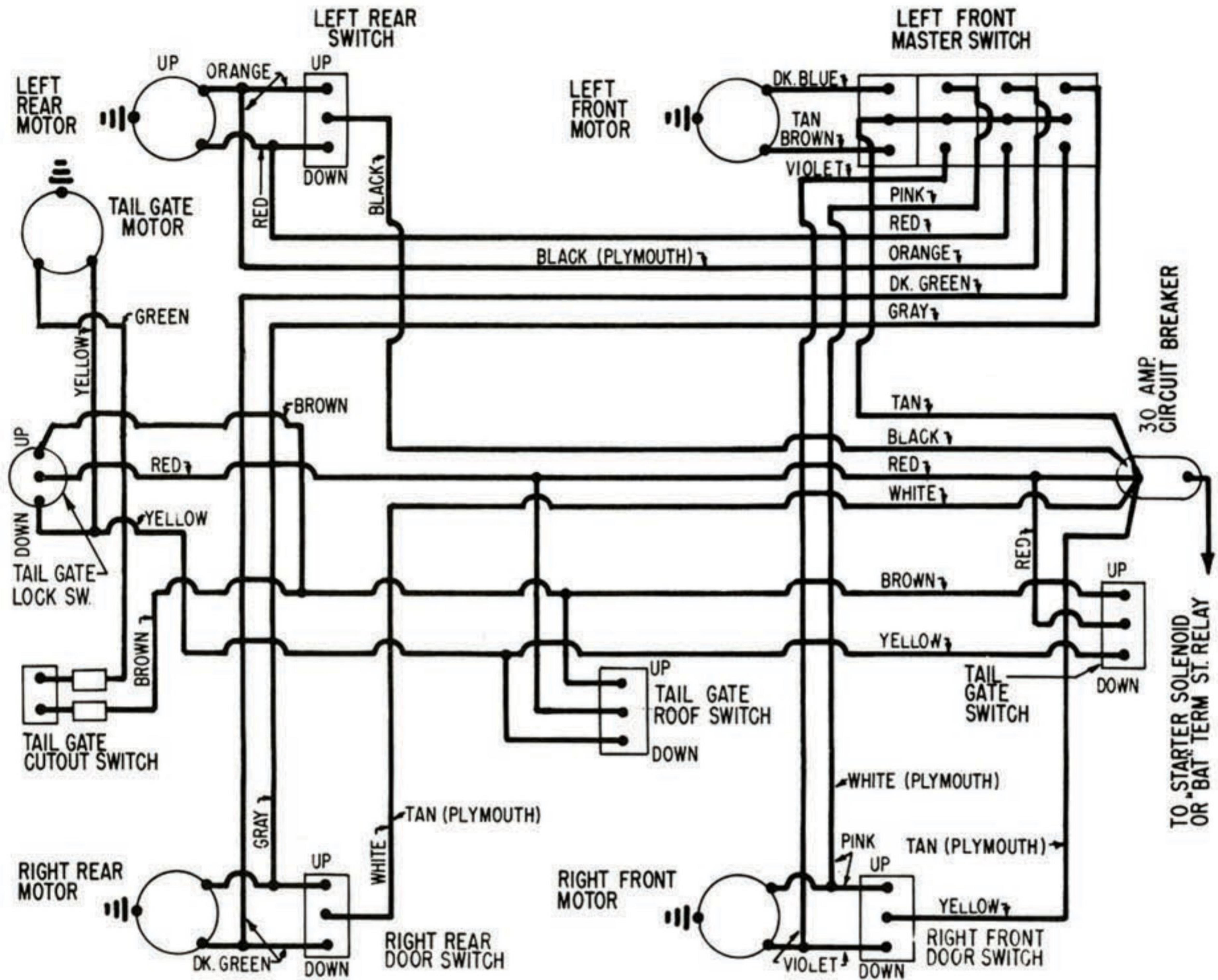
CHRYSLER, DE SOTO, DODGE, PLYMOUTH WINDOW CONTROL WIRING DIAGRAM
