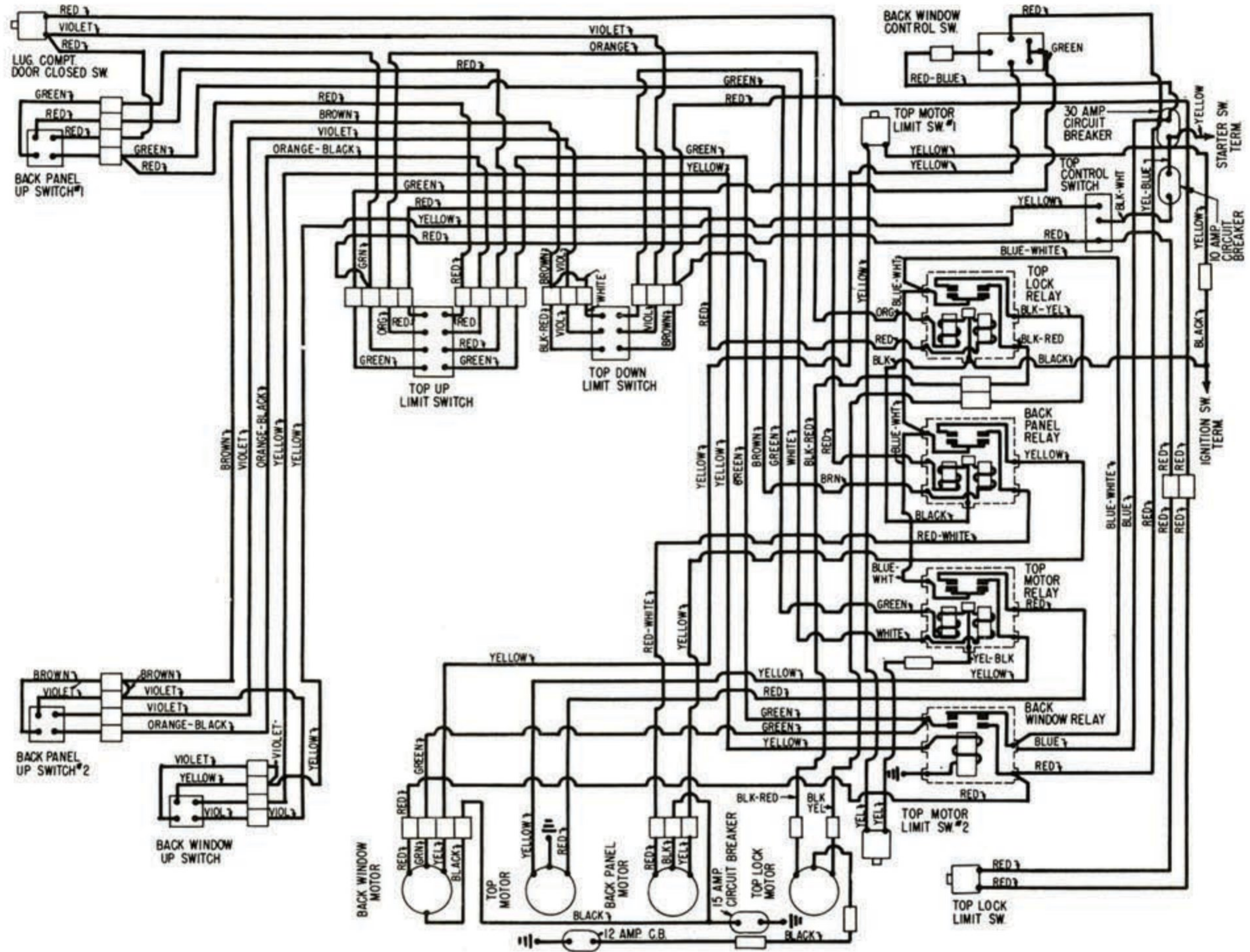
CONTINENTAL CONVERTIBLE TOP CONTROL WIRING DIAGRAM
