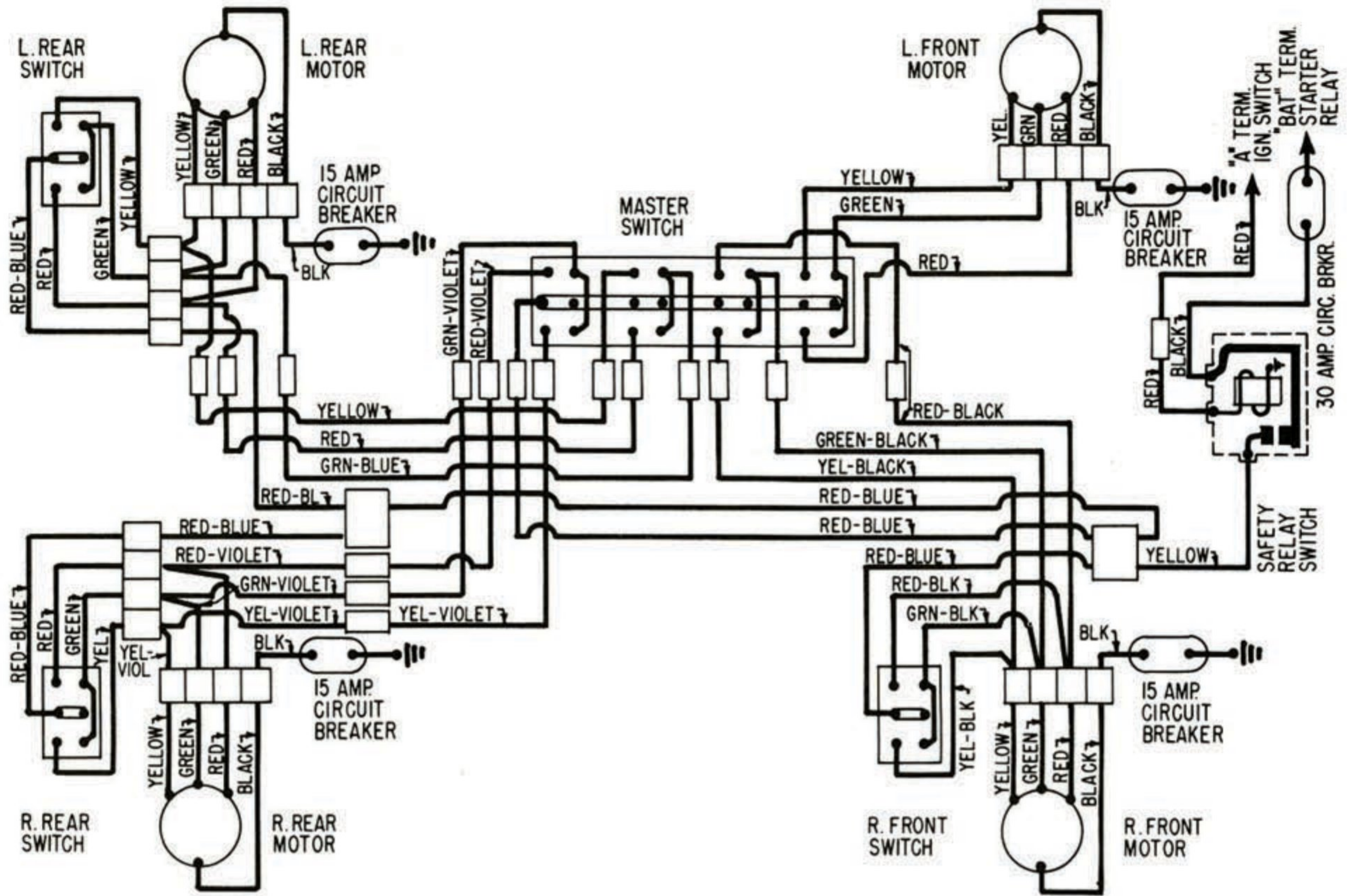
FORD & EDESEL WINDOW CONTROL WIRING DIAGRAM
