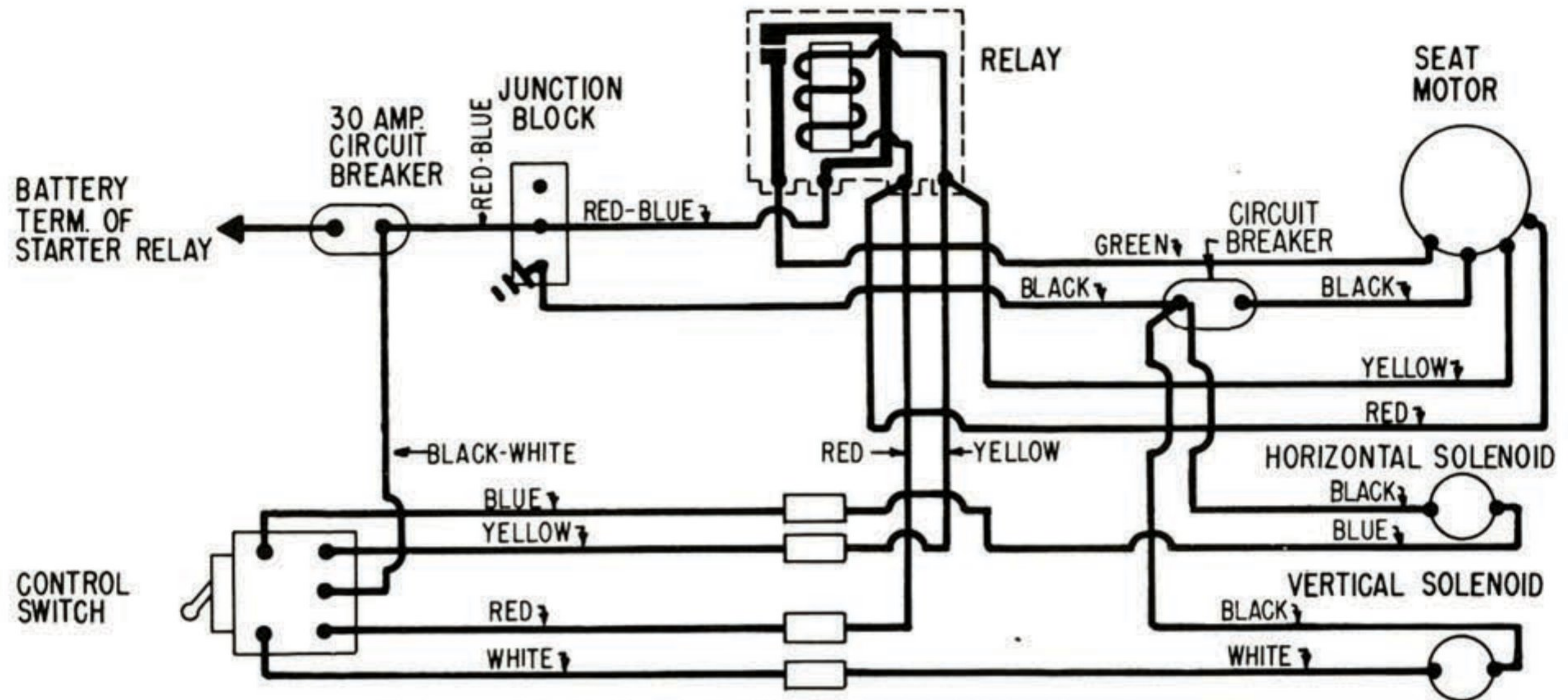
EDSEL, FORD & MERCURY FOUR-WAY SEAT CONTROL WIRING DIAGRAM
