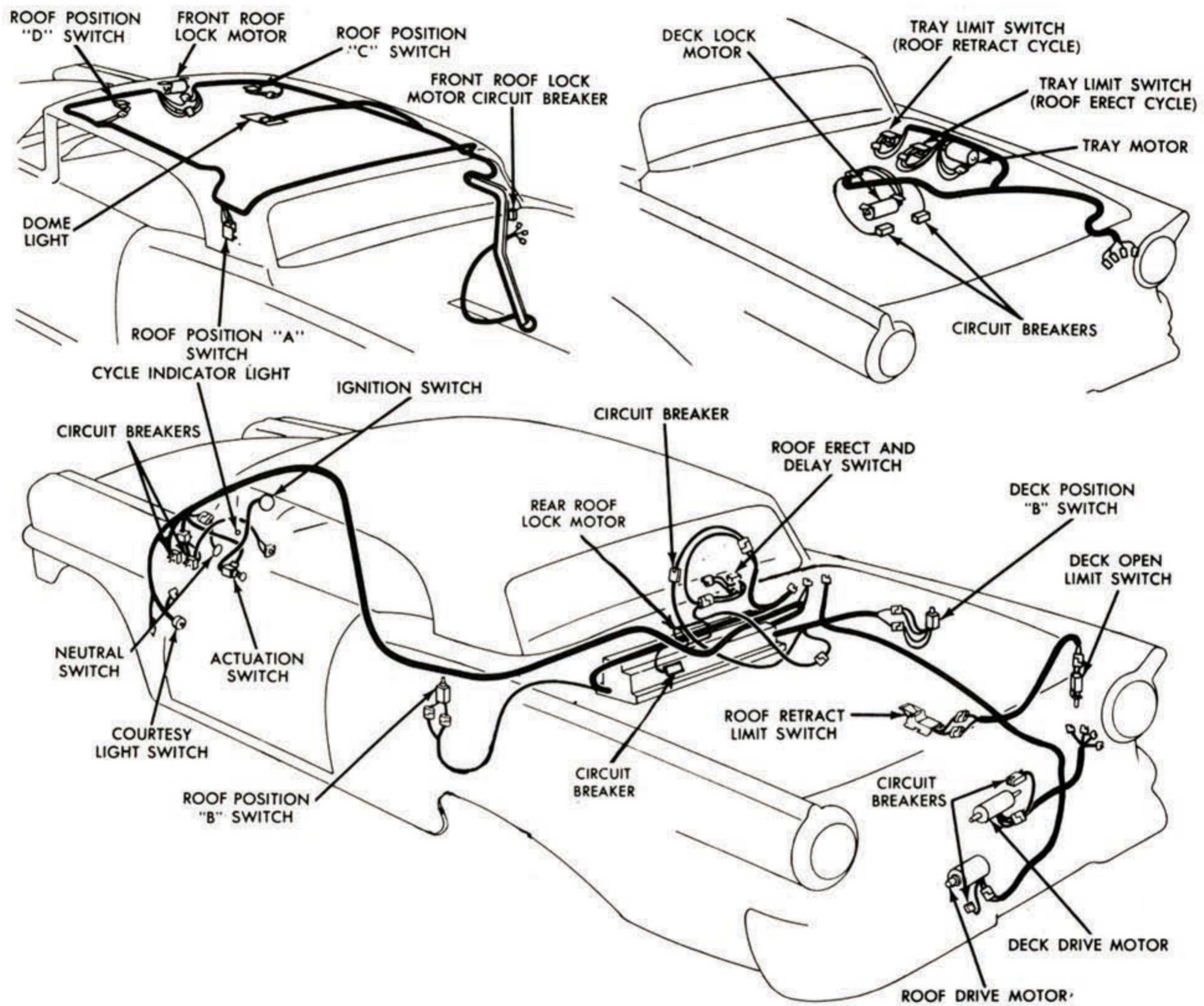
FORD HARDTOP MOTOR & SWITCH LOCATIONS
