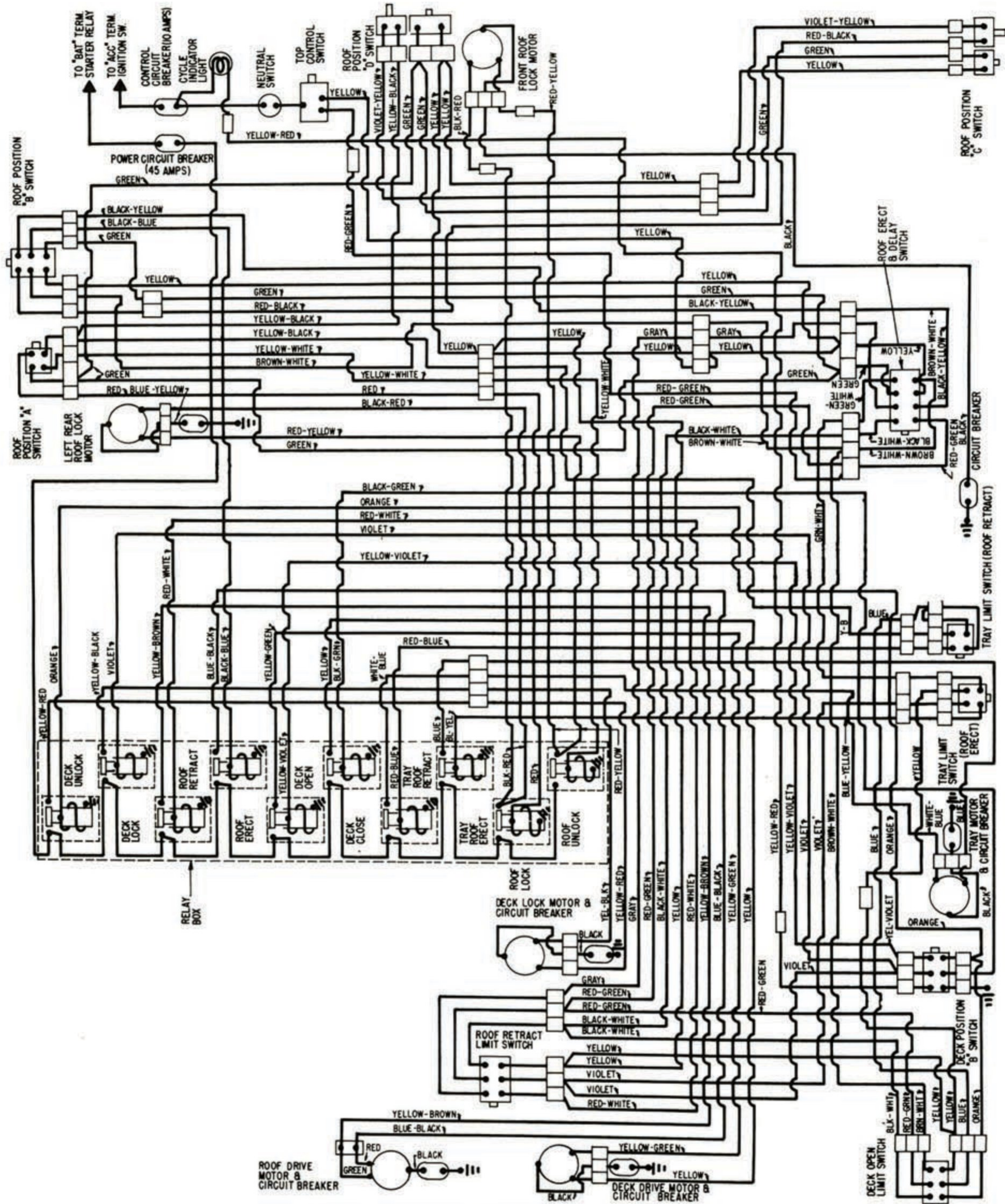
FORD RETRACTABLE HARDTOP WIRING DIAGRAM
