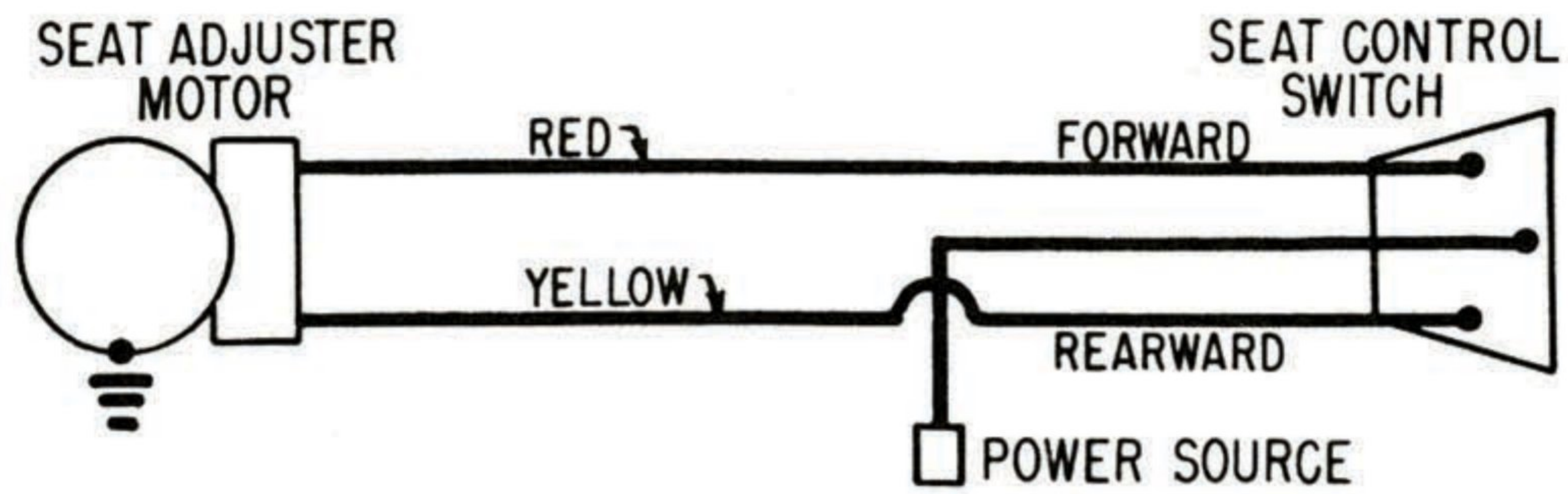
G.M. 2-WAY SEAT WIRING DIAGRAM
