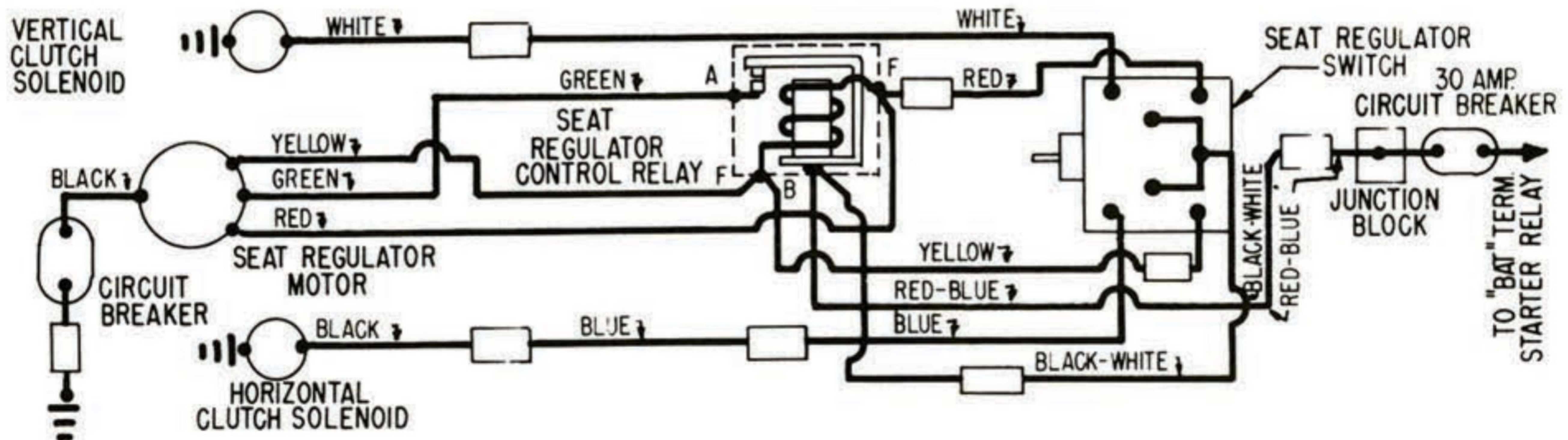
LINCOLN FOUR-WAY SEAT CONTROL WIRING DIAGRAM
