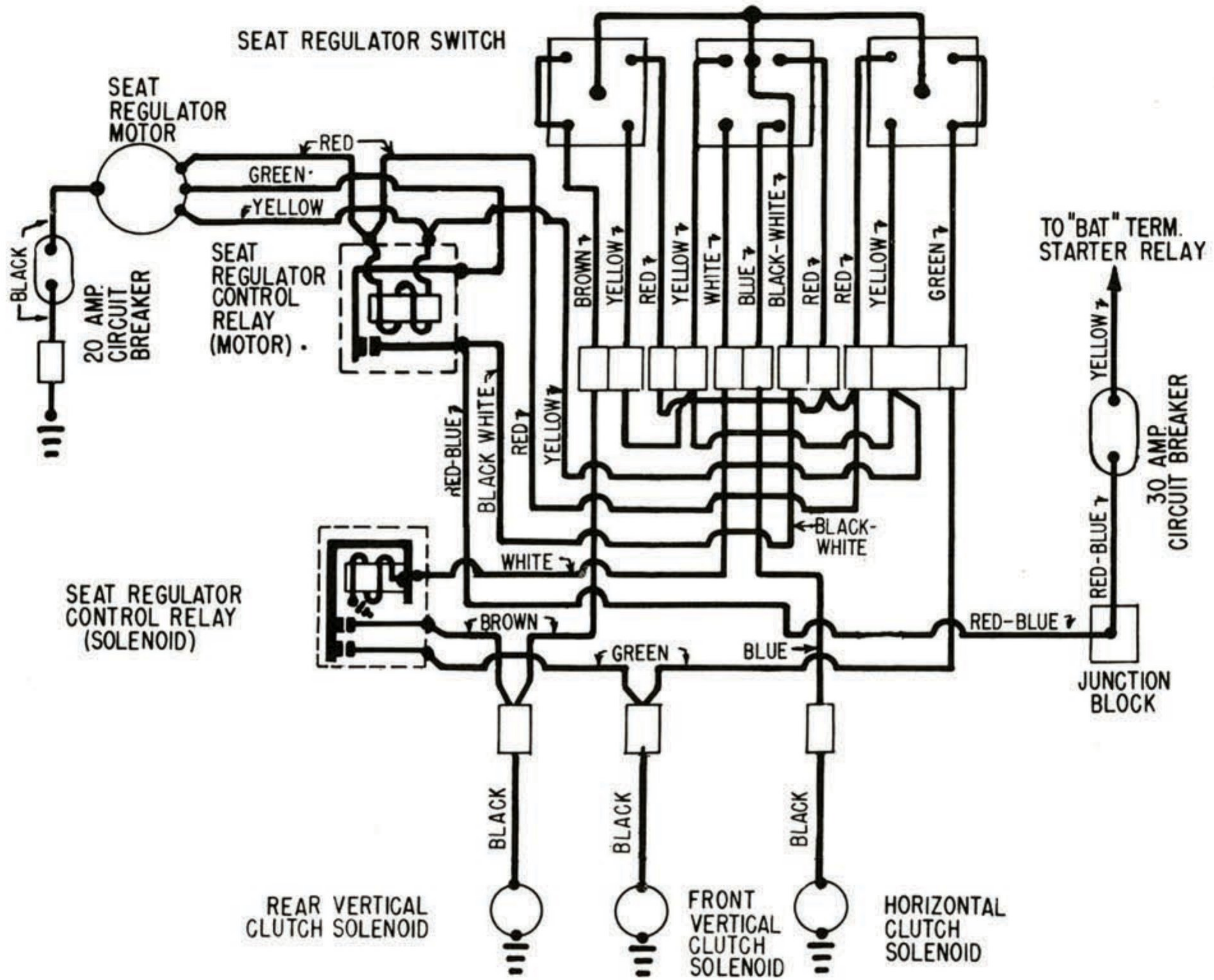
LINCOLN SIX-WAY SEAT CONTROL WIRING DIAGRAM
