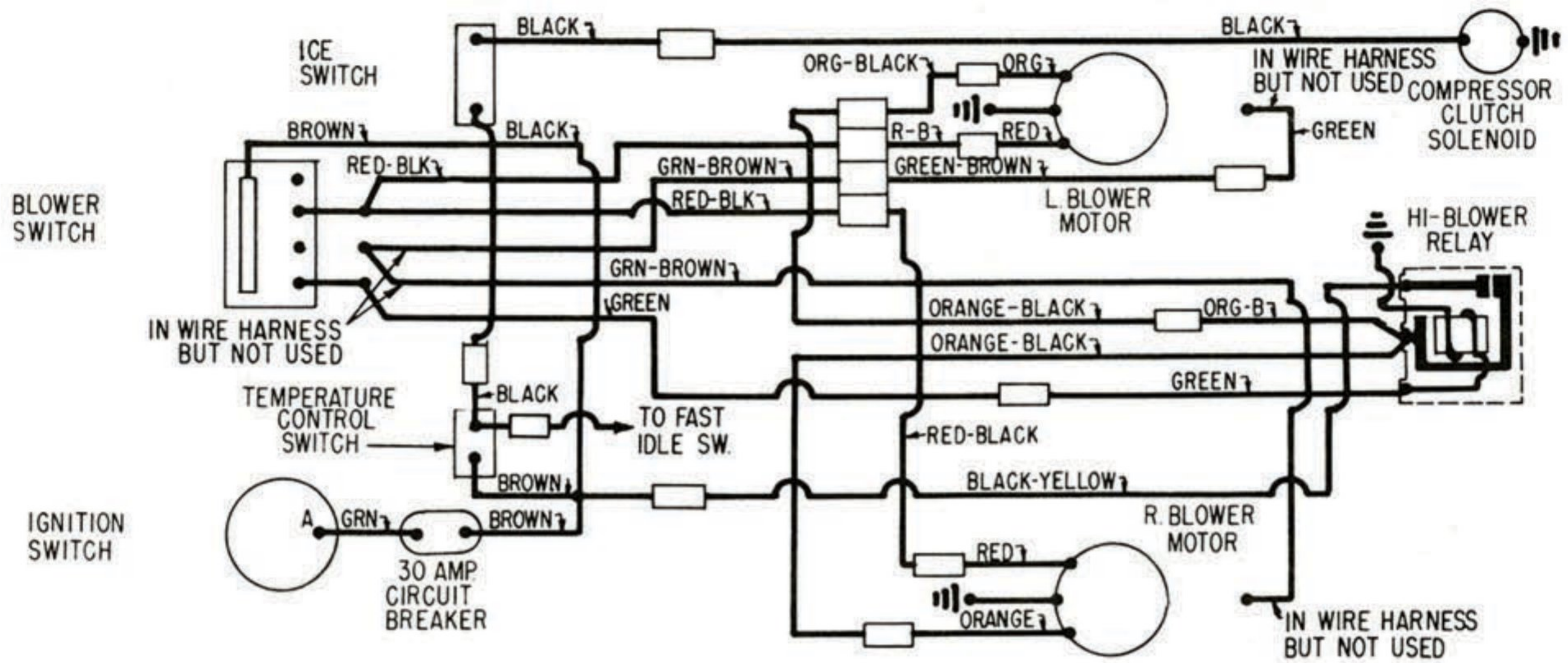
LINCOLN AIR CONDITIONING CONTROL DIAGRAM
