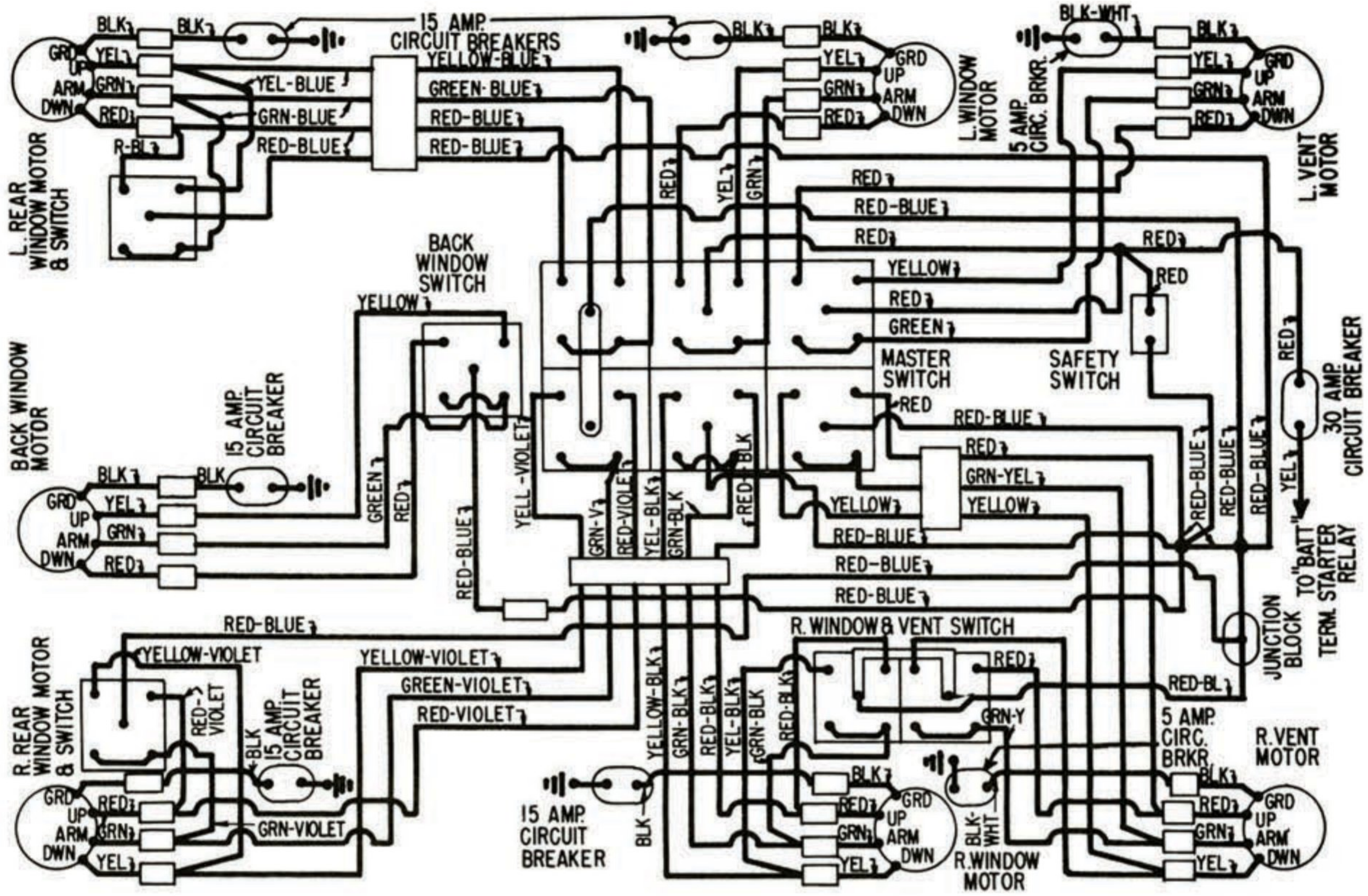
LINCOLN WINDOW CONTROL WIRING DIAGRAM
