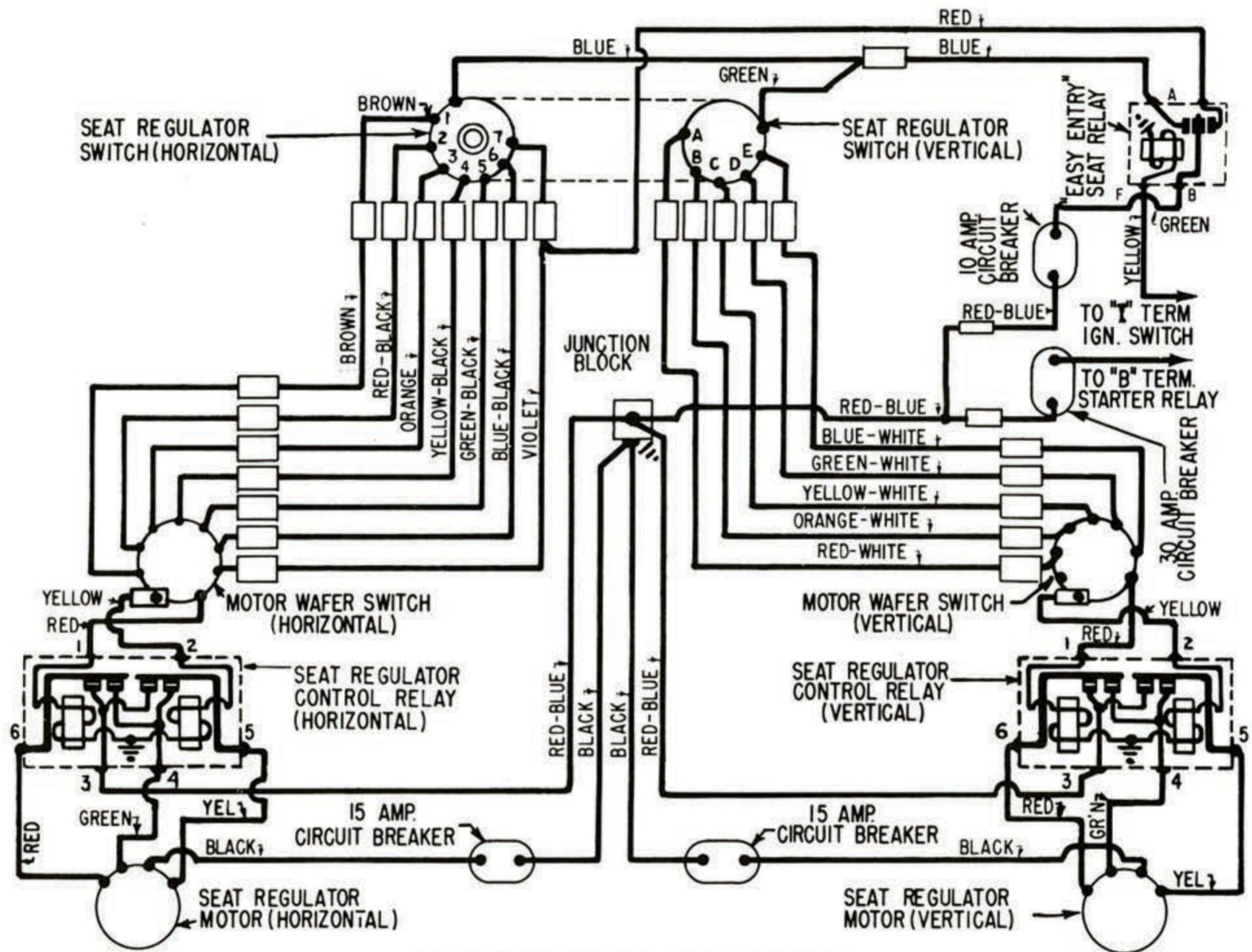
MERCURY SEAT-O-MATIC WIRING DIAGRAM
