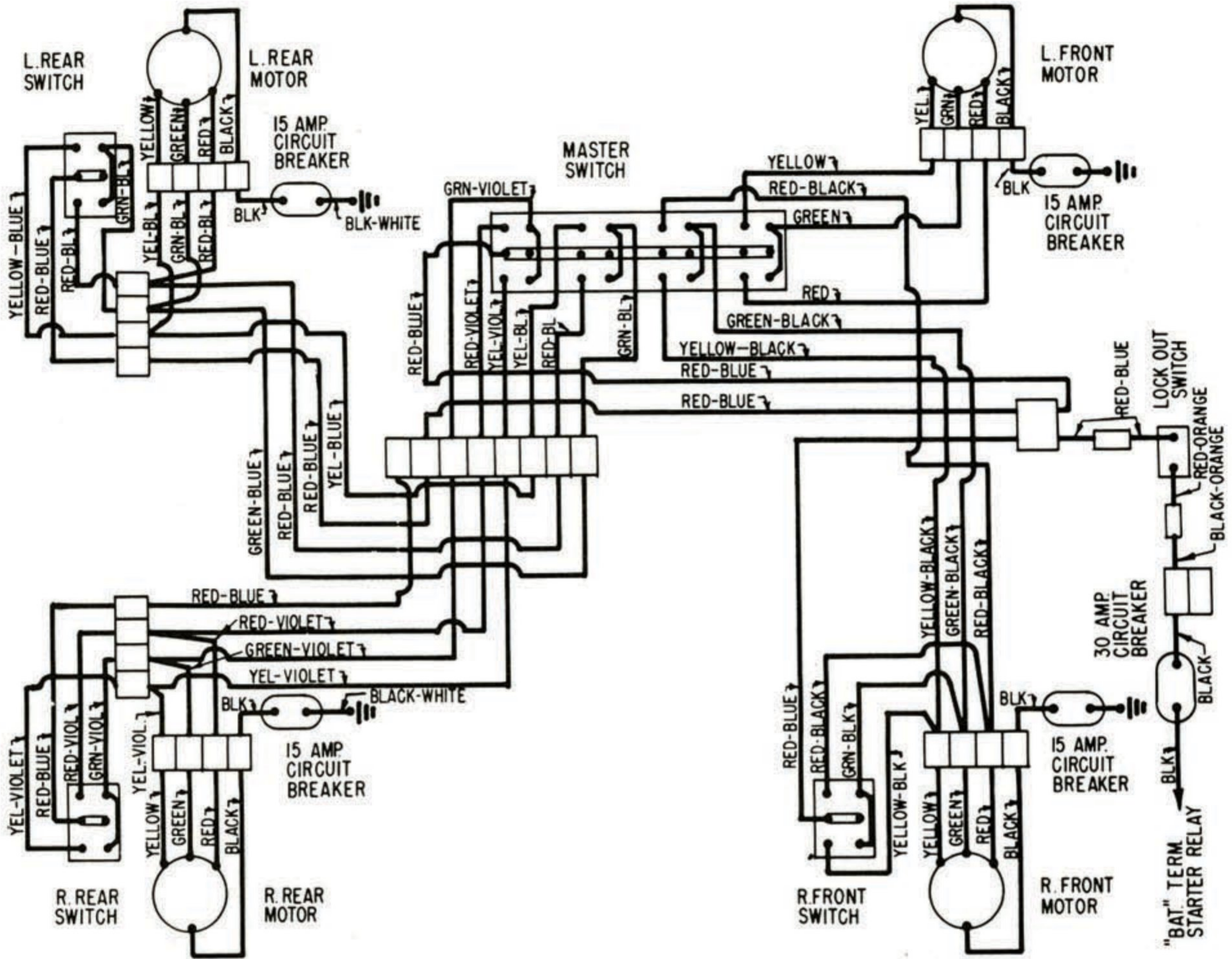
MERCURY WINDOW CONTROL WIRING DIAGRAM
