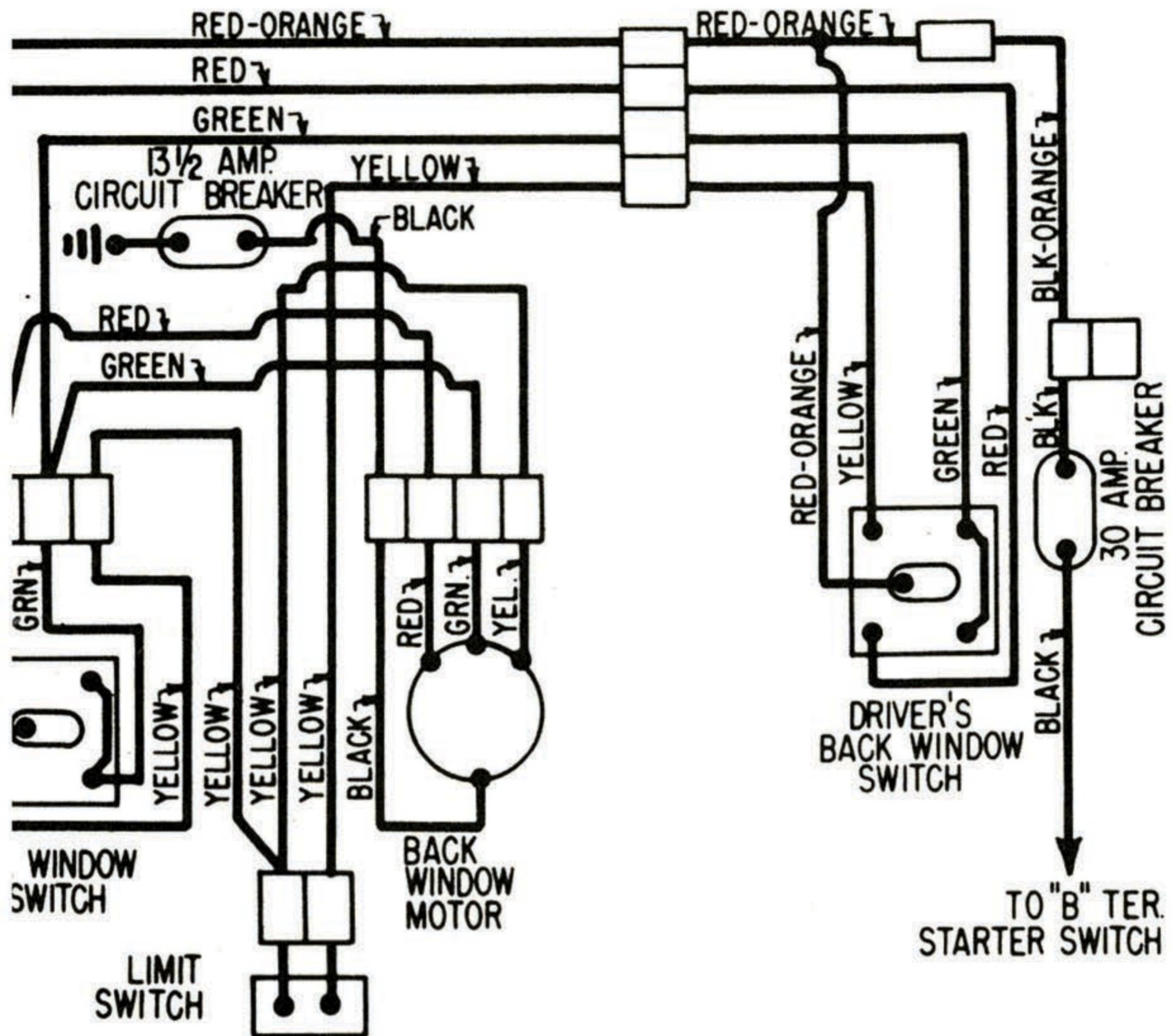
MERCURY TAIL GATE WINDOW CONTROL WIRING DIAGRAM
