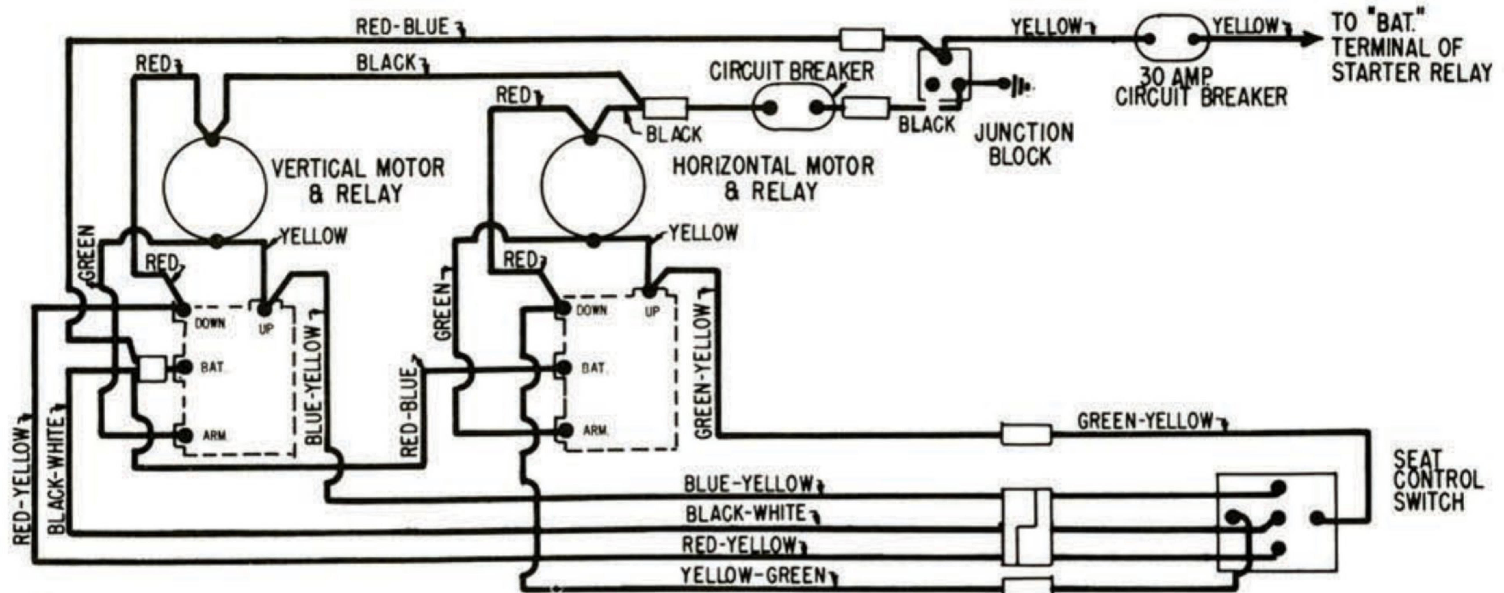
FORD THUNDERBIRD SEAT CONTROL WIRING DIAGRAM (ONE SEAT SHOWN)
