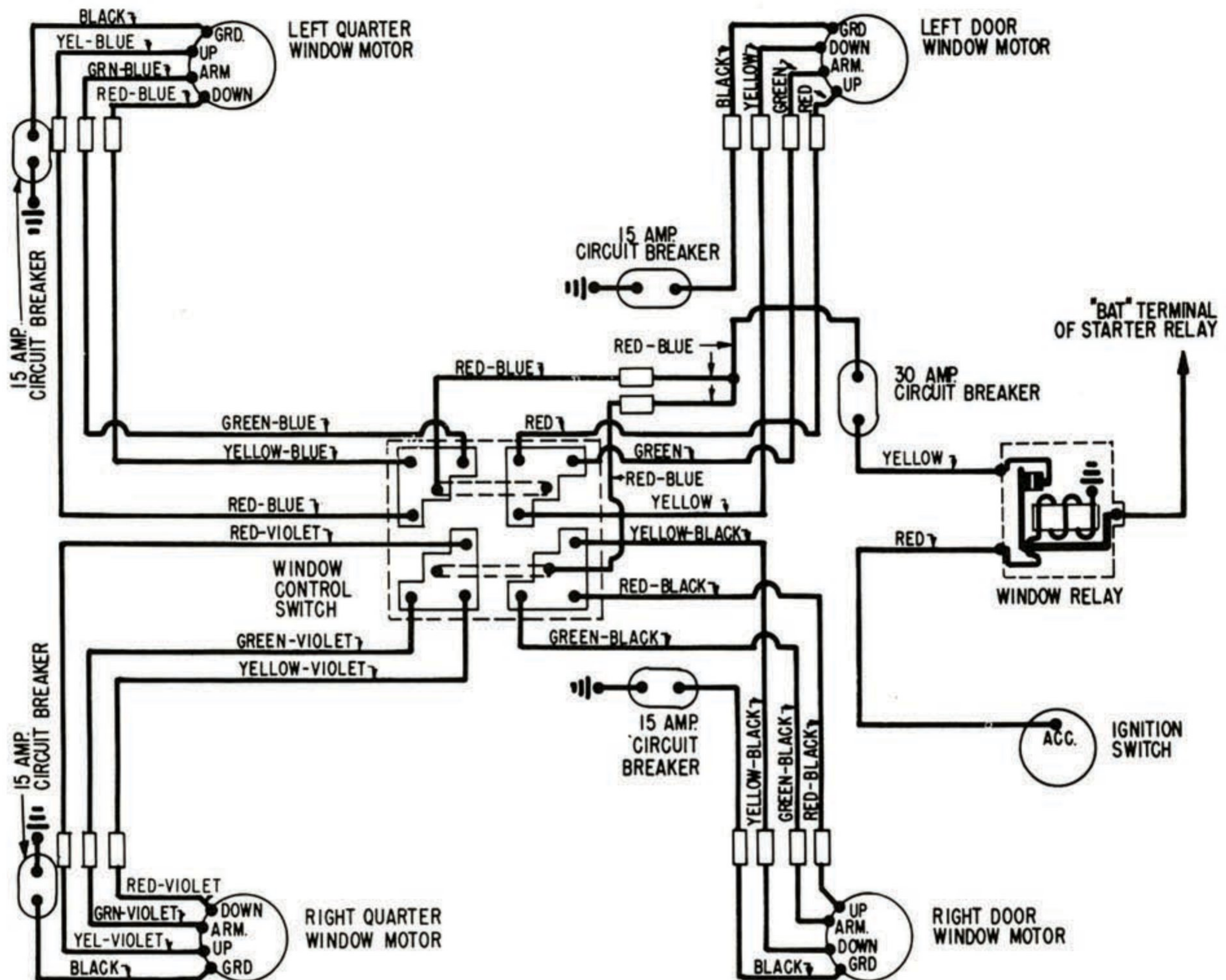
FORD THUNDERBIRD WINDOW CONTROL WIRING DIAGRAM
