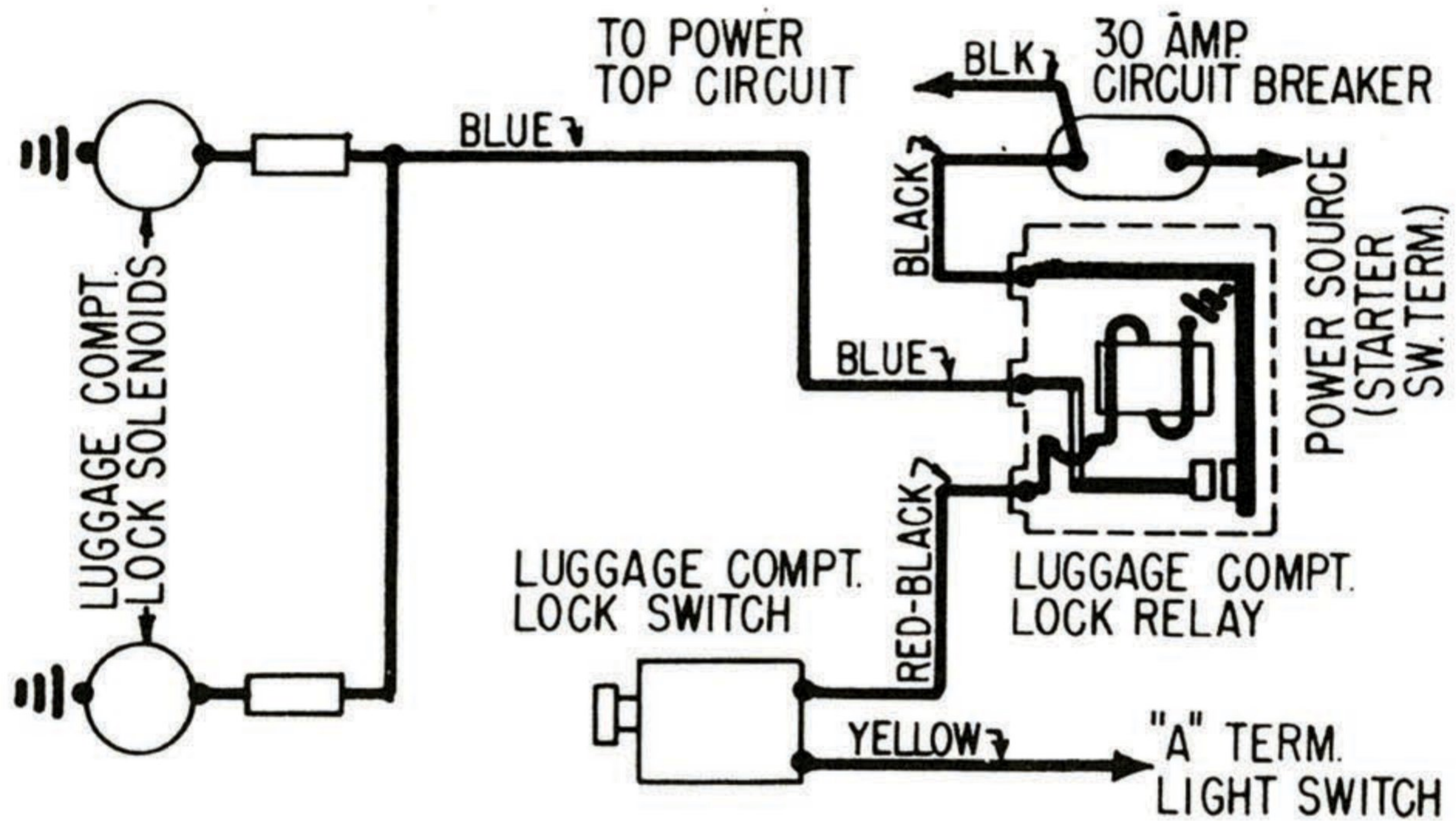
THUNDERBIRD TRUNK LOCK DIAGRAM
