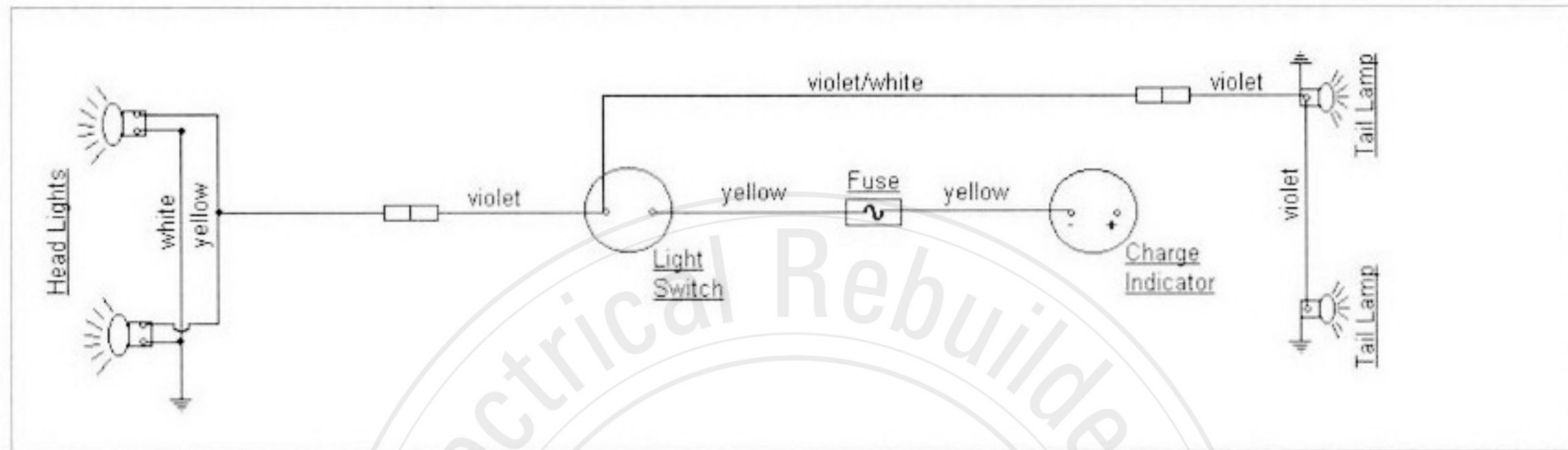
Electric Lighting Wiring Diagram.
