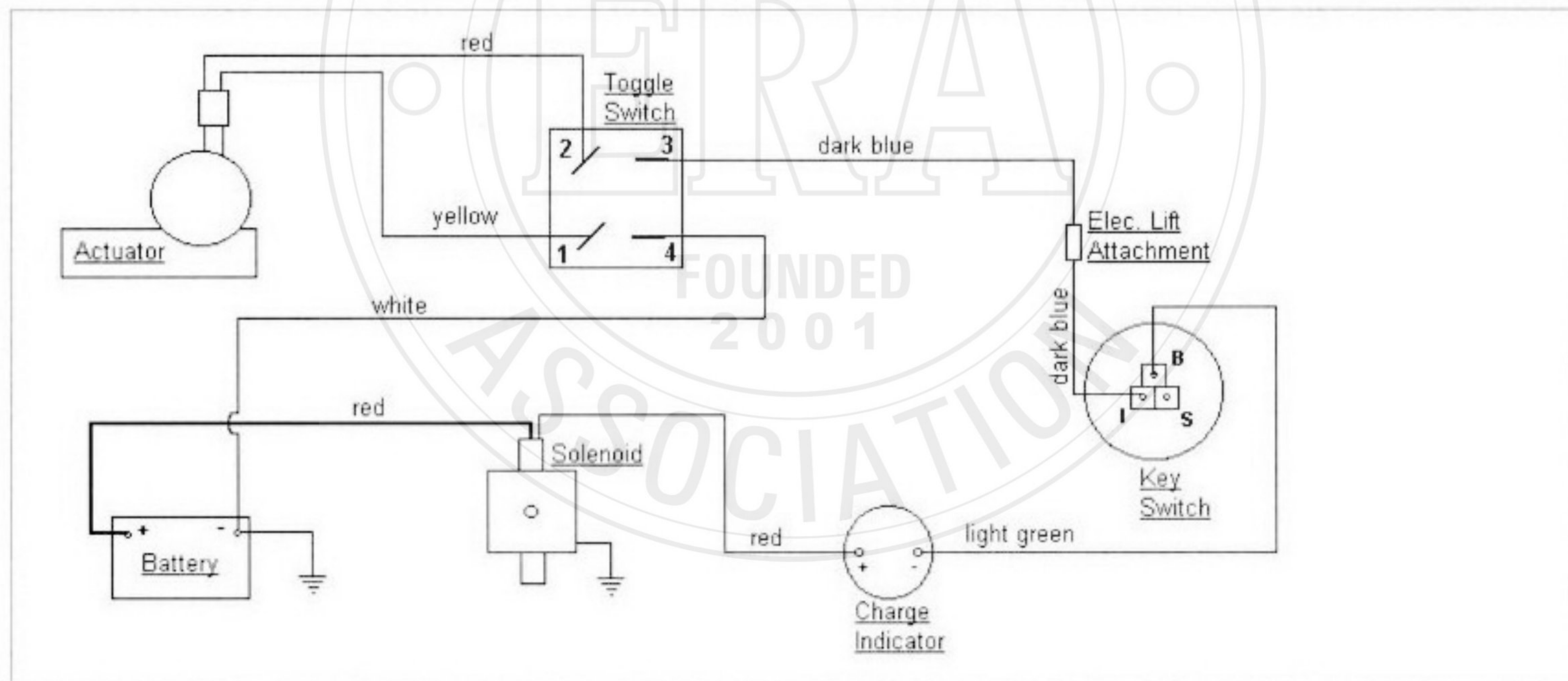
Electric Lift Wiring Diagram.
