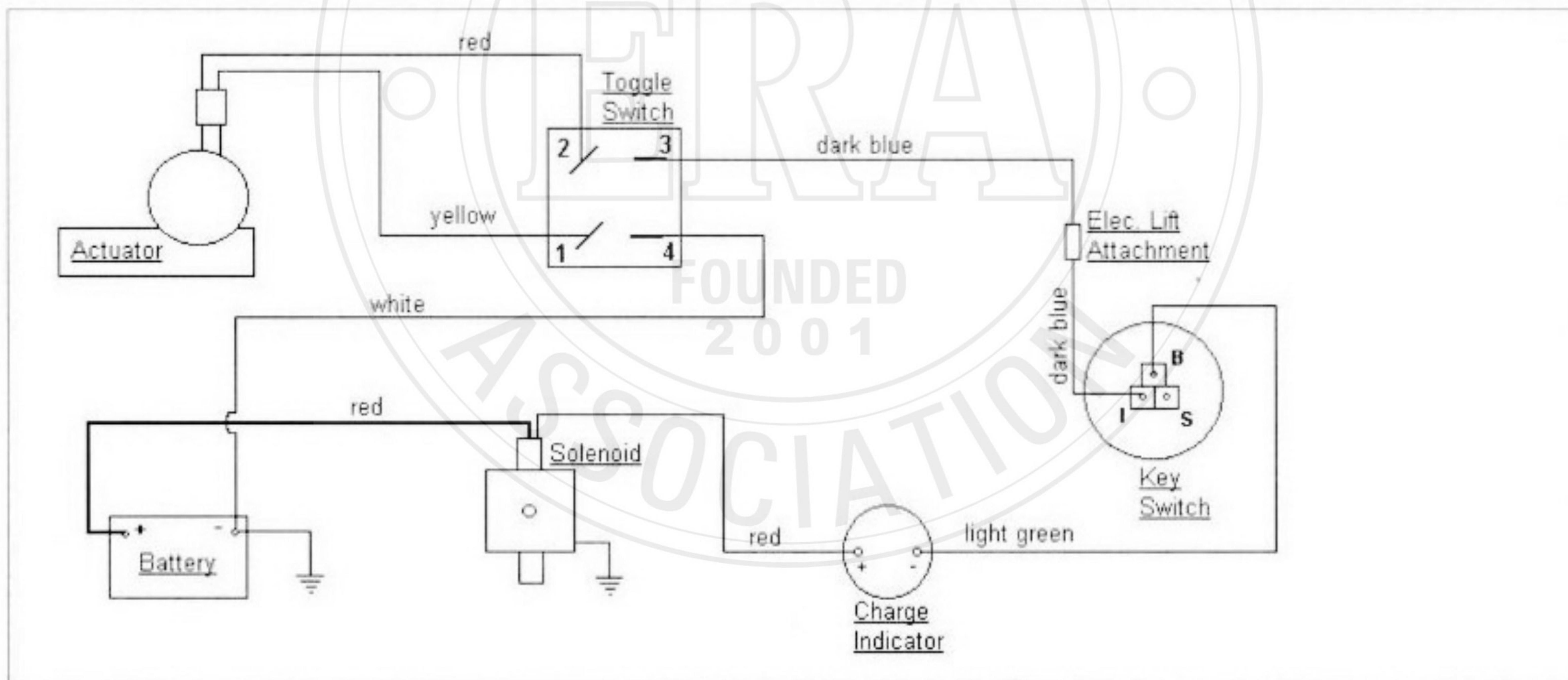
Electric Lift Wiring Diagram.
