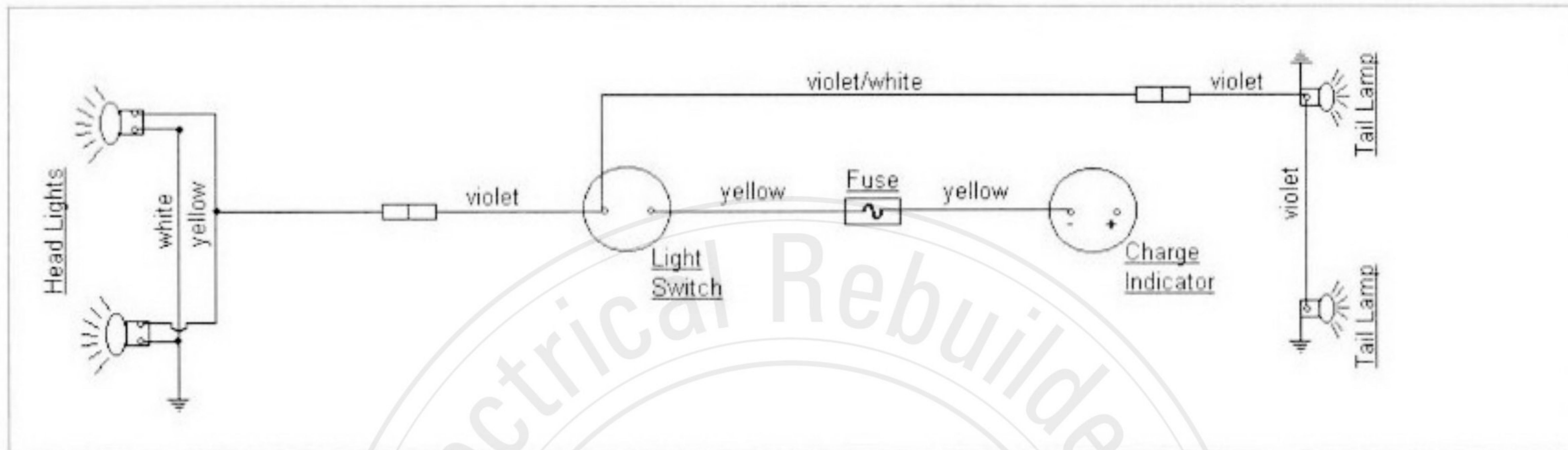
Electric Lighting Wiring Diagram.
