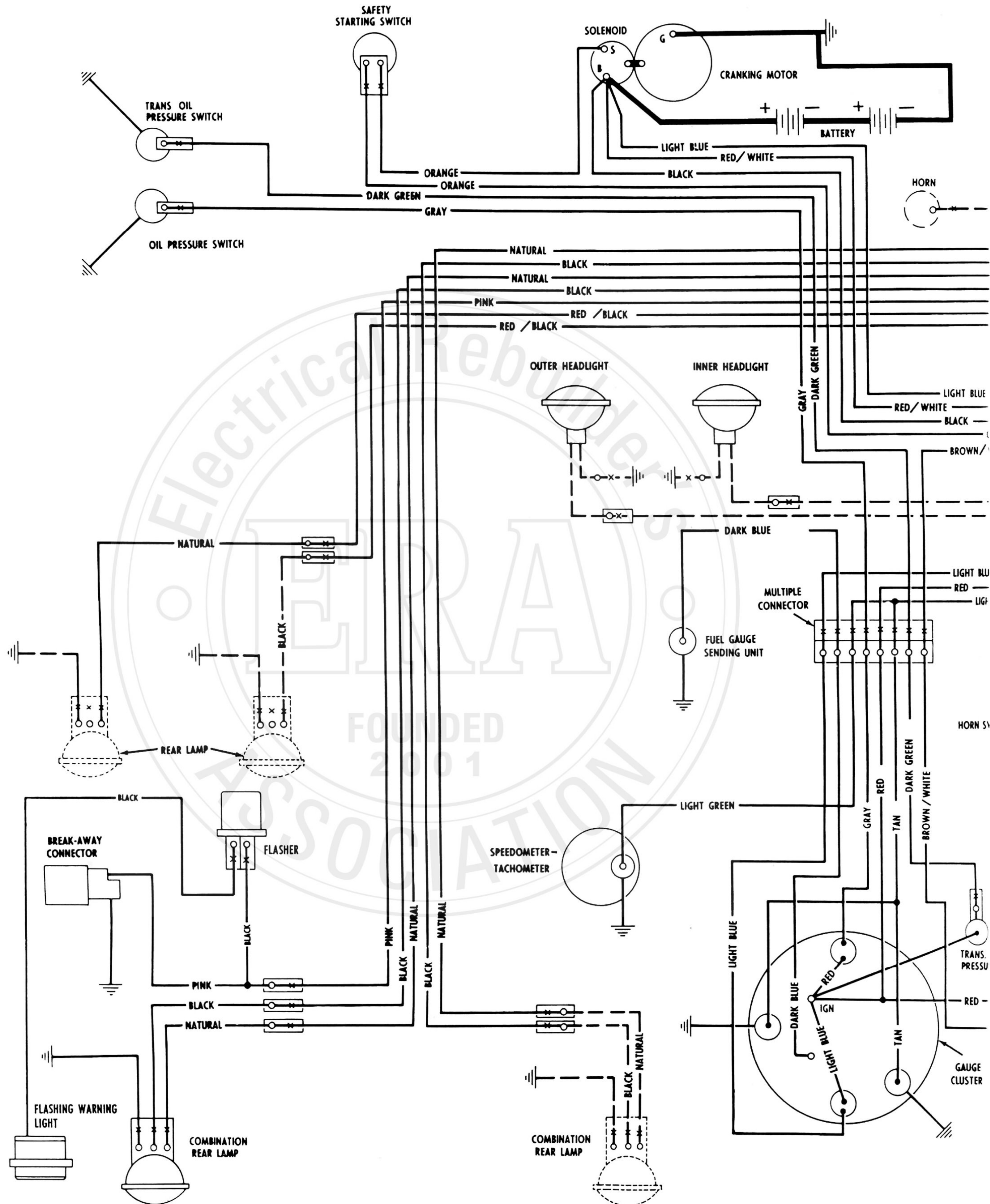
Schematic wiring diagram (4100 and 4156).
