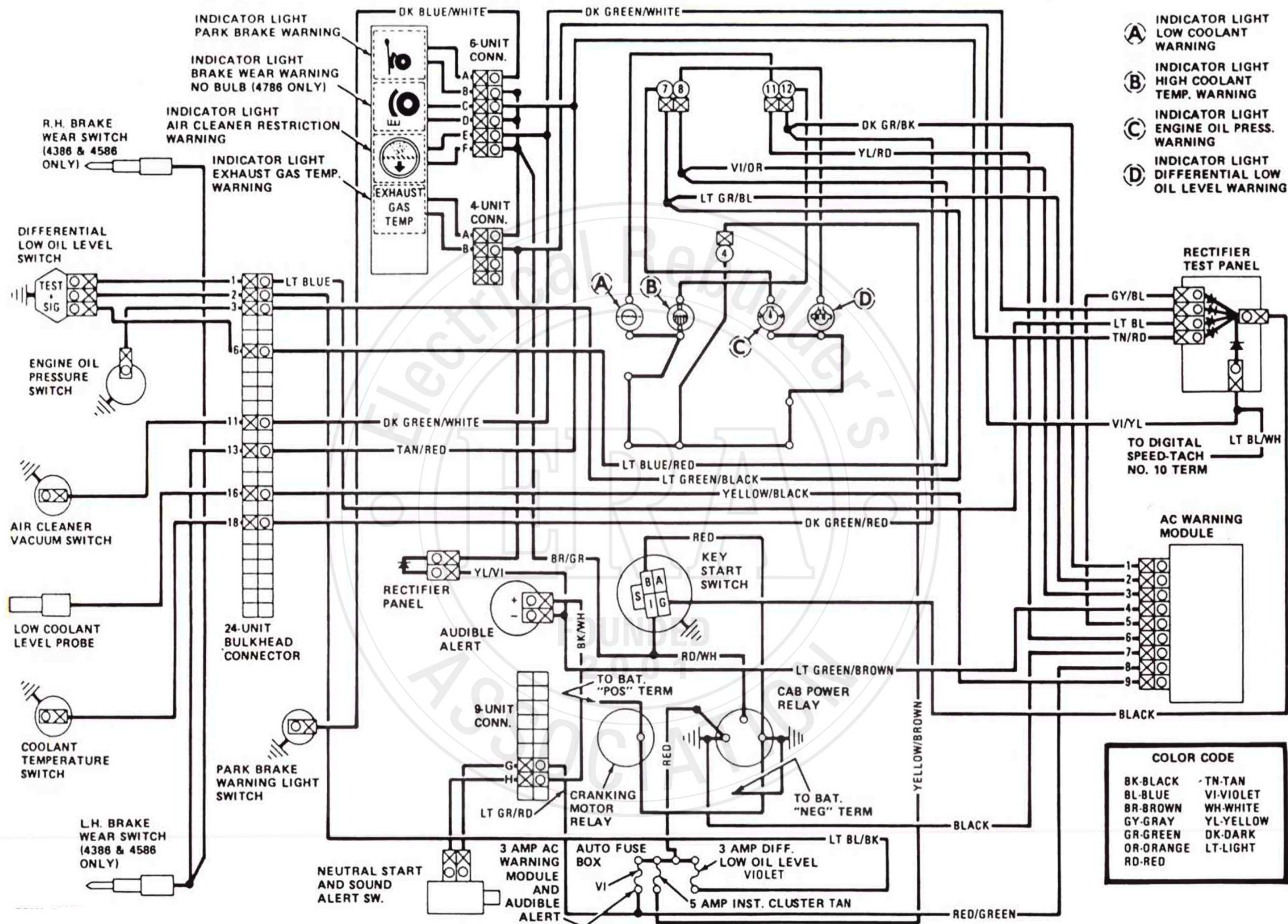
EARLY WARNING SYSTEM — 4386, 4586 Serial Number 1501 and Above and 4786 Tractor 501 and Above
