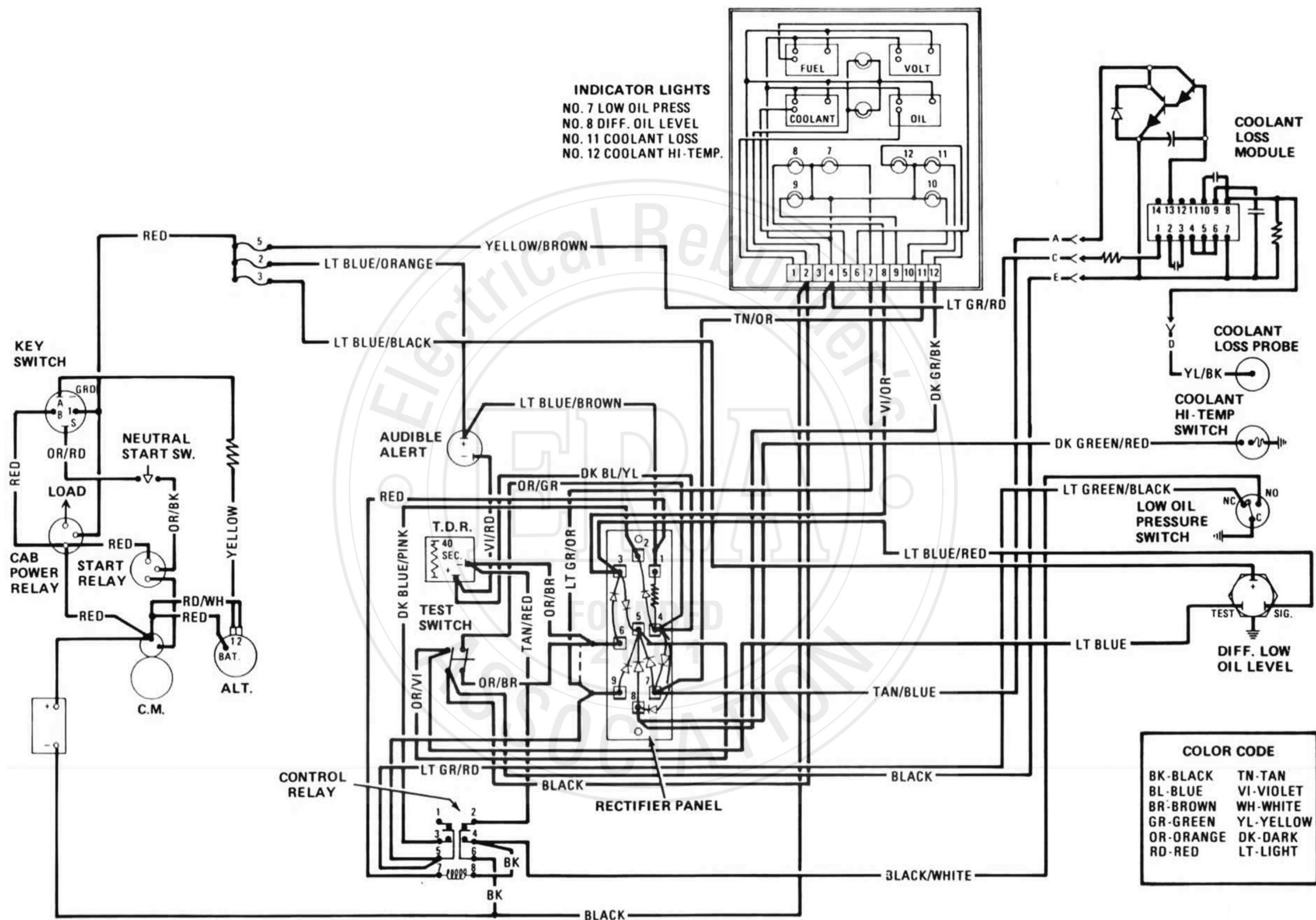
EARLY WARNING SYSTEM – 4386, 4586 Serial Number 1500 and Below
