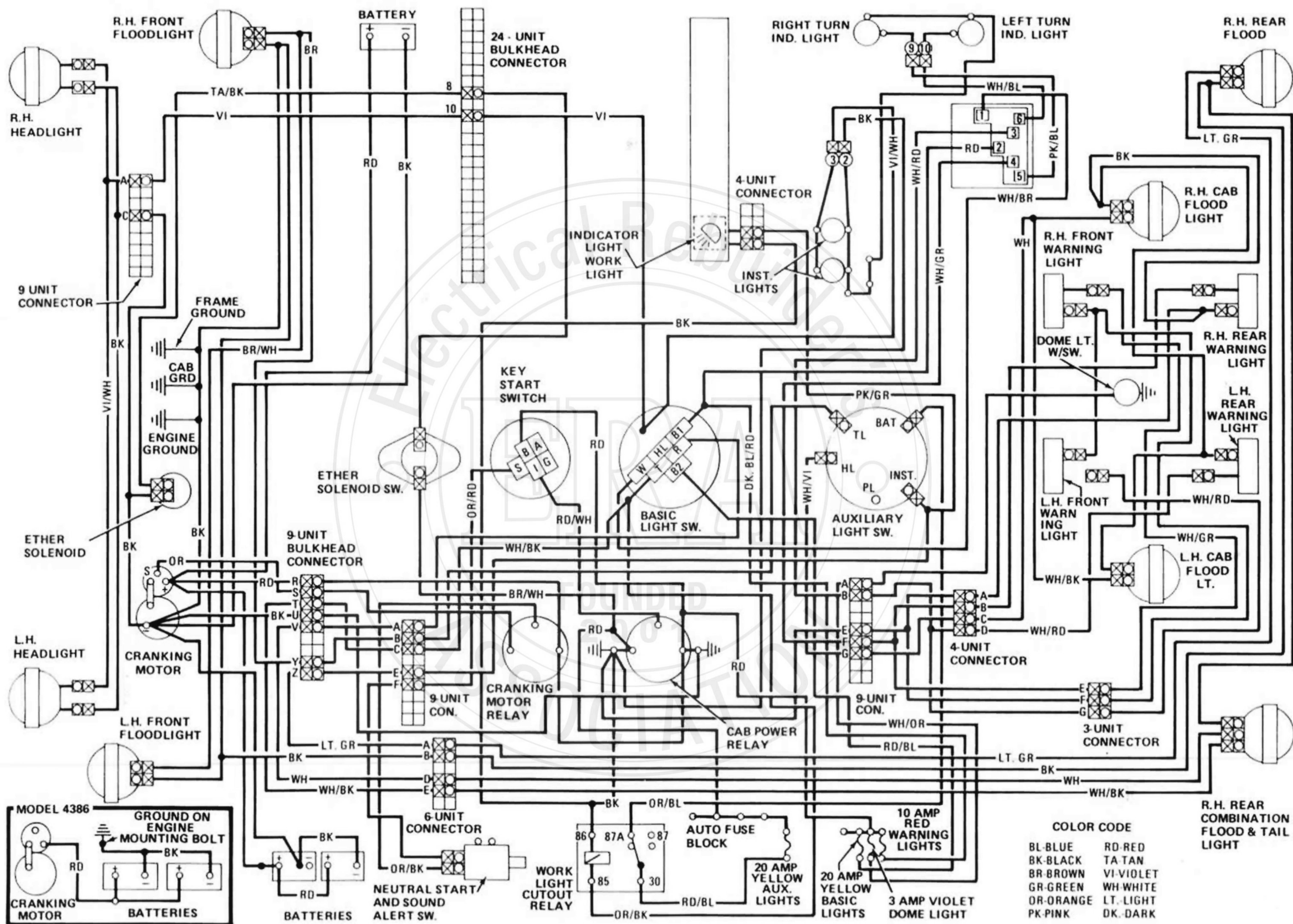
Starting and Lighting Wiring — 4386, 4586 and 4786 Tractors
