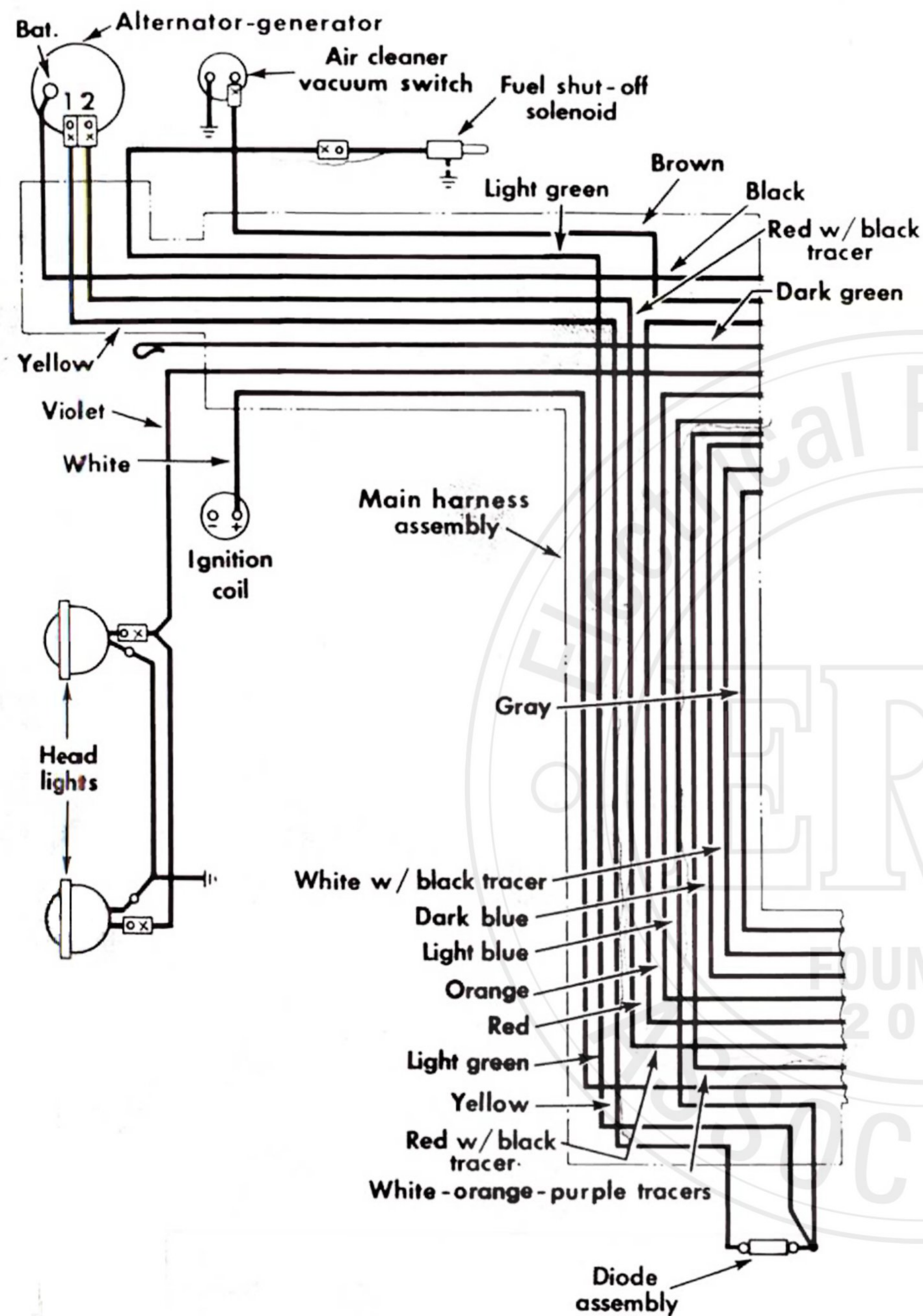
Alternator-generator with integral voltage regulator (766 gas tractor).
