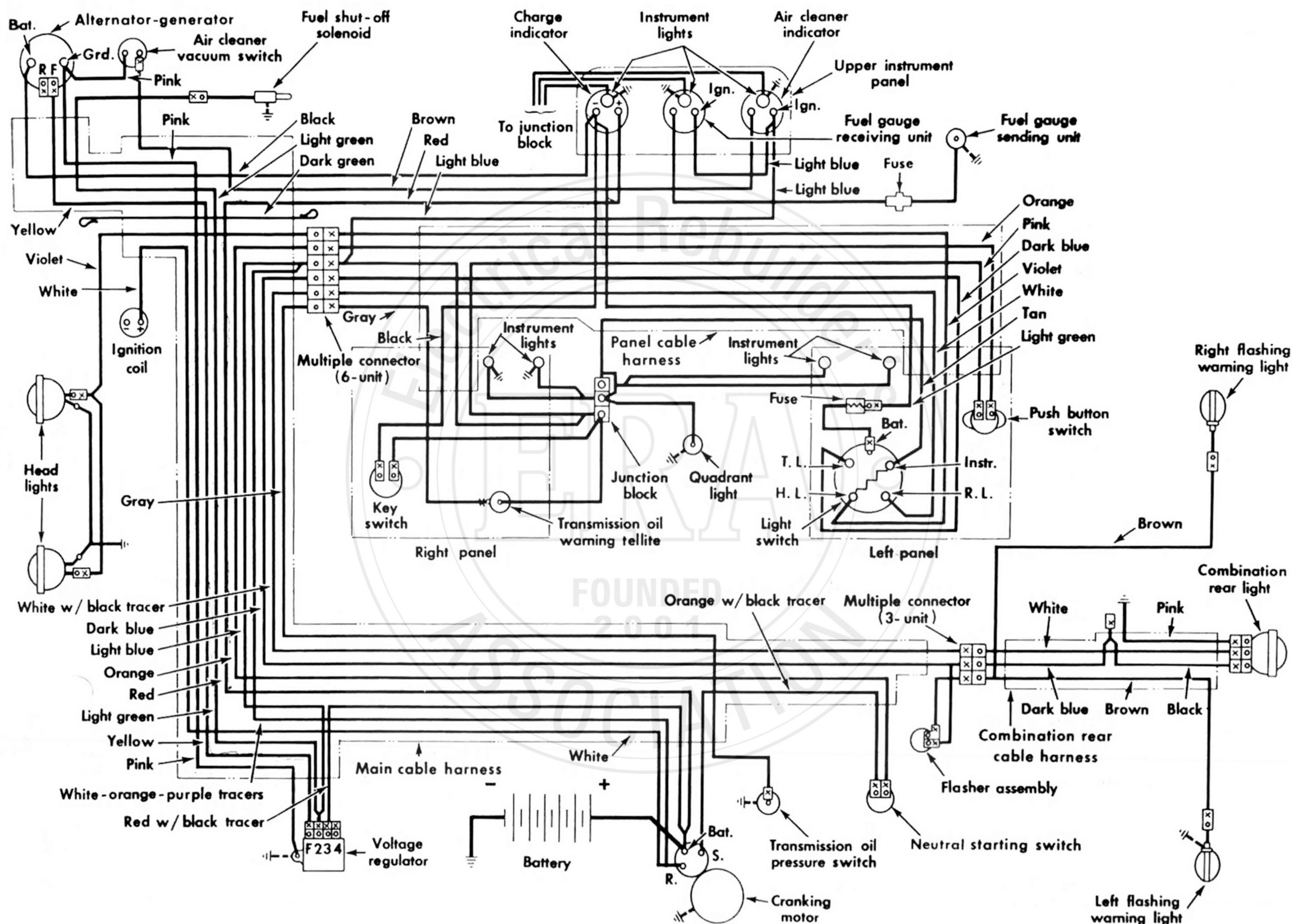
Wiring diagram (766 gas tractor).
