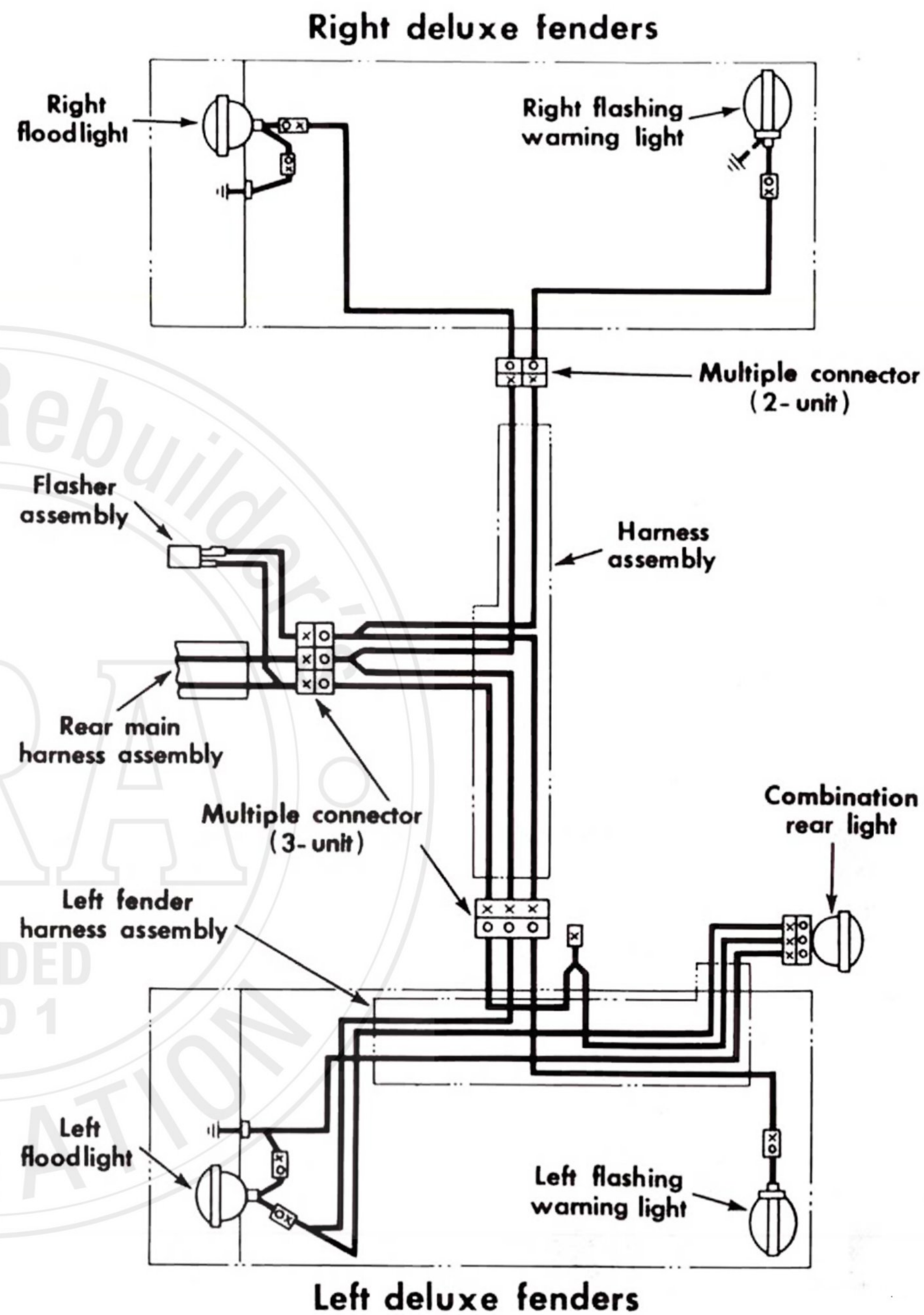
Schematic wiring diagram for deluxe fenders.
