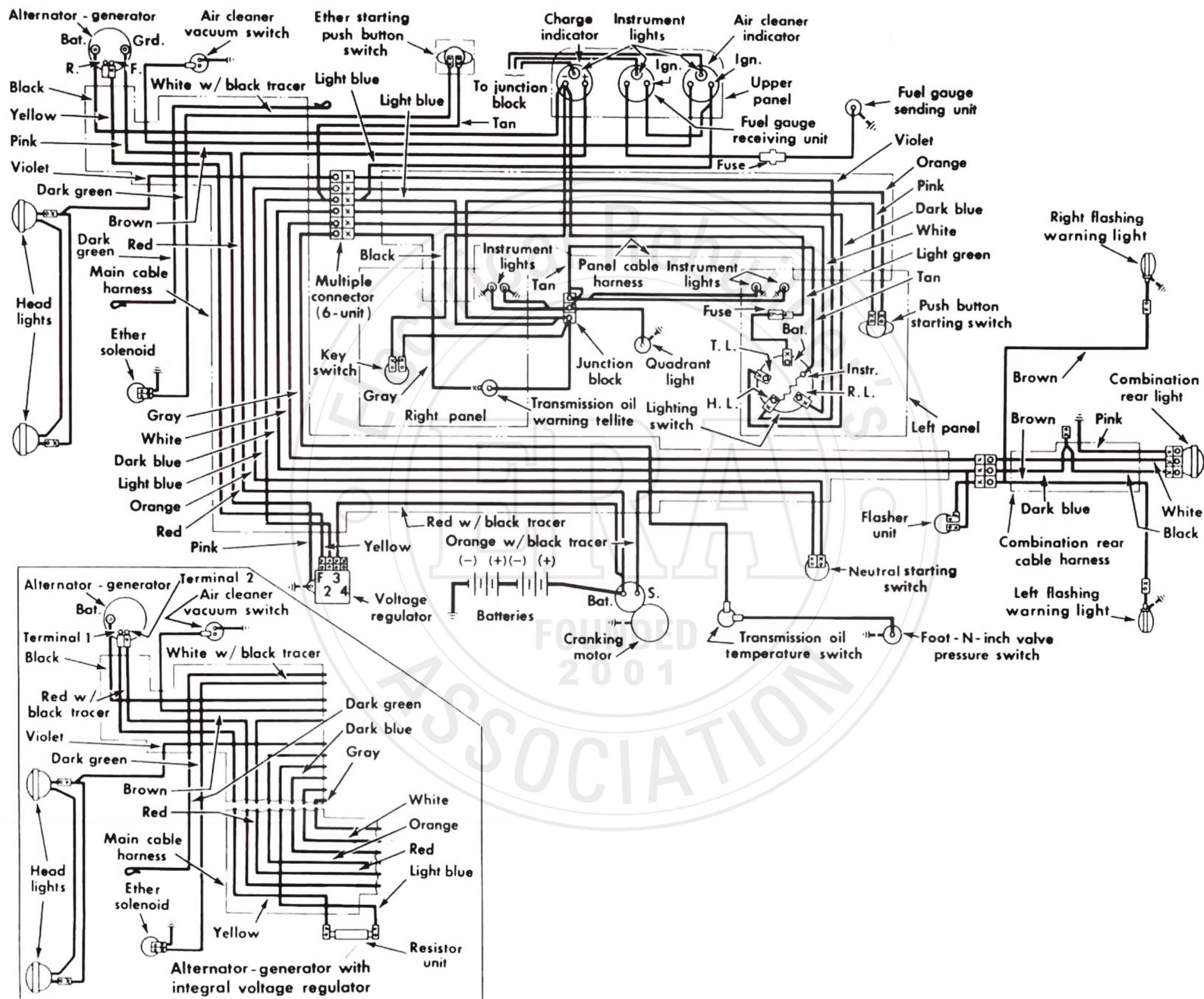
Hydrostatic Drive Tractors (966 and 1066) Schematic Wiring Diagram.
