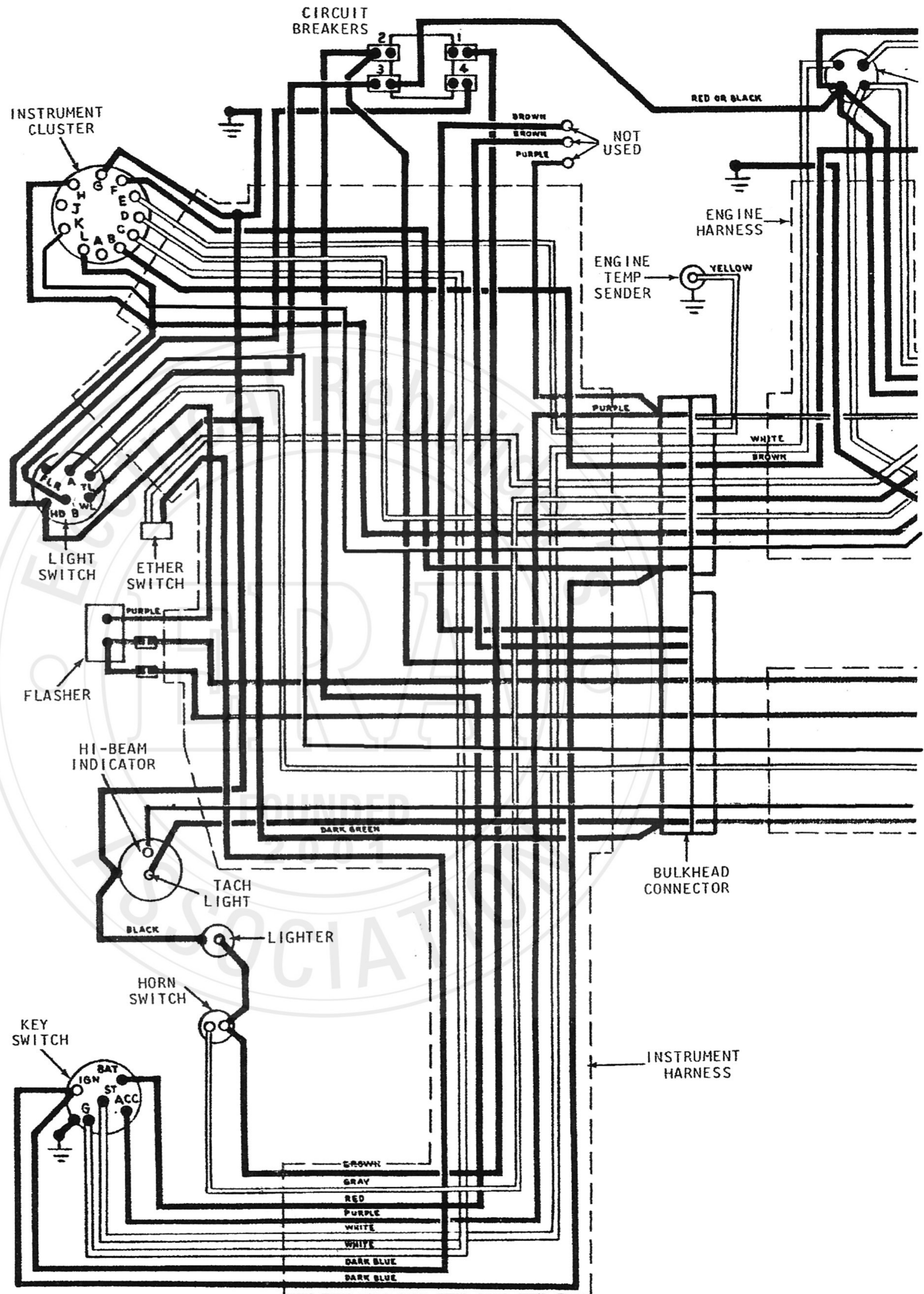
Wiring for Tractor without Four-Post Roll Gard or Sound-Gard Body
