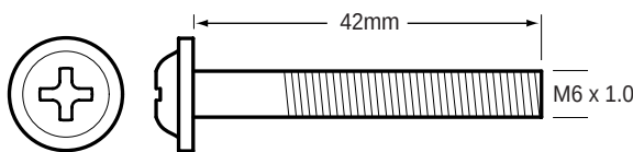
85-1336 Screw
