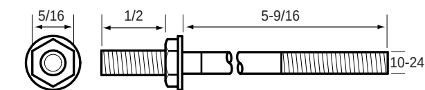
84-1349 Thru Bolt w/ Extension
