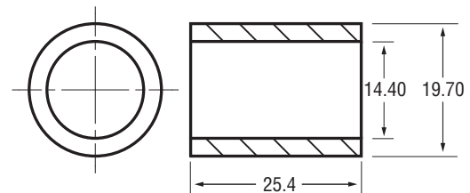
62-1506 Bushing - C.E.
