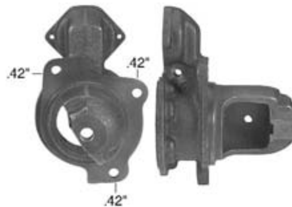
51-114 D.E. Housing Cast Iron, Wet Clutch
