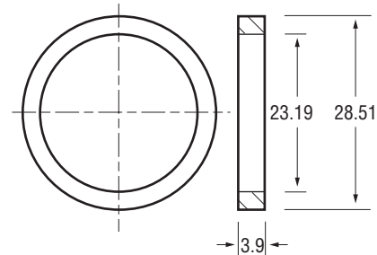
62-82801 Bushing - Starter Drive
