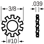
84-4300 External Tooth Lock Washer Dim: #10 ID x 3/8 OD x .039 T Features: • Zinc-plated
