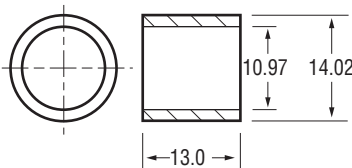
62-83403 Bushing - D.E., C.S.
