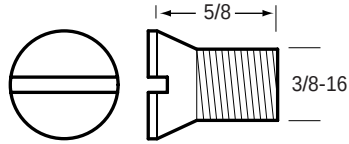
84-1500 Screw
