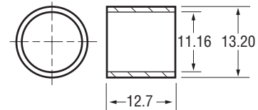
62-1407 Conversion Bushing - D.E.
