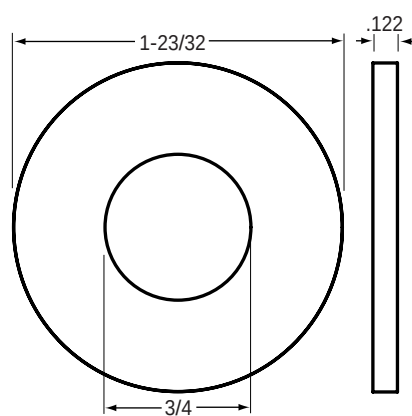
84-4710 Flat Washer
