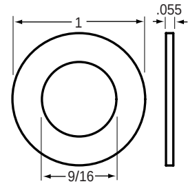
84-4610 Flat Washer
