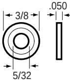
84-4102 Flat Washer Dim: 5/32 ID x 3/8 OD x .050 T Features: • Concave surface • Plain finish
