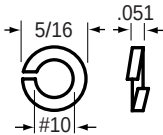
84-4309 Split Lock Washer Dim: #10 ID x 5/16 OD x .051 T Features: • Zinc-plated
