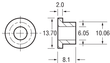
62-94200 Bushing - C.E. (Fld. Case)
