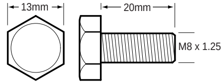
85-1402 Bolt
