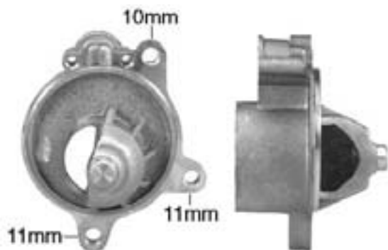
51-243 D.E. Housing Aluminum
