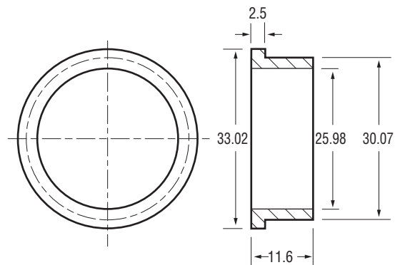
62-91901 Bushing - D.E.
