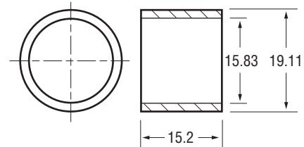
62-2600-2 Bushing - C.E. .0050" (2X) Undersize
