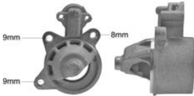
51-259 D.E. Housing Aluminum
