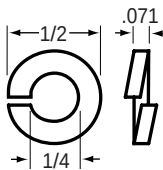
84-4401 Split Lock Washer Dim: 1/4 ID x 1/2 OD x .071 T Features: • Zinc-plated
