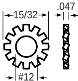
84-4303 External Tooth Lock Washer Dim: #12 ID x 15/32 OD x .047 T Features: • Zinc-plated
