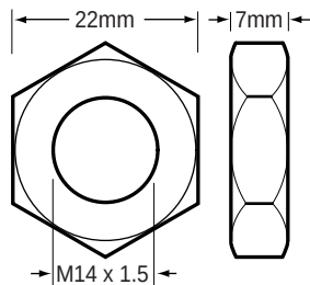
85-2601 Hex Nut
