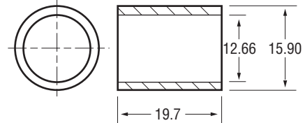
62-1406-1 Bushing - D.E. .0025" (1X) Undersize
