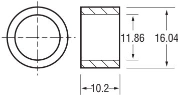
62-2403-2 Bushing - D.E. .0050" (2X) Undersize
