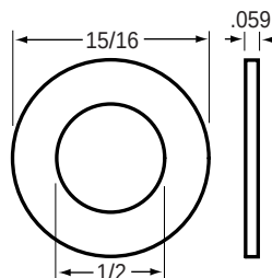
84-4617 Flat Washer
