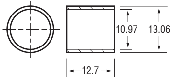
62-83400 Bushing - D.E.
