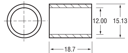
62-2400 Bushing - D.E.
