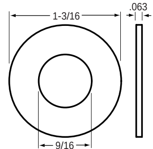
84-4613 Flat Washer
