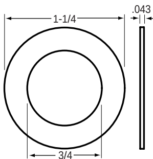
84-4709 Flat Washer
