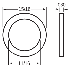
84-4619 Flat Washer
