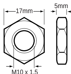
85-2503 Hex Nut
