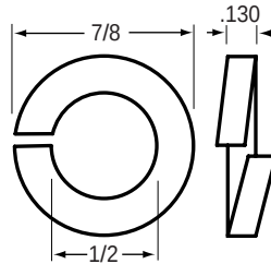
84-4600 Split Lock Washer
