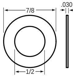
84-4603 Flat Washer
