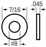
84-4203 Flat Washer Dim: #8 ID x 7/16 OD x .045 T Features: • Zinc-plated
