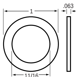
84-4604 Flat Washer
