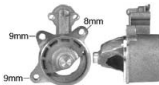
51-249 D.E. Housing Aluminum
