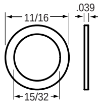
84-4503-1 Flat Washer
