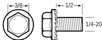
84-1402 Screw
