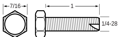
84-1419 Screw
