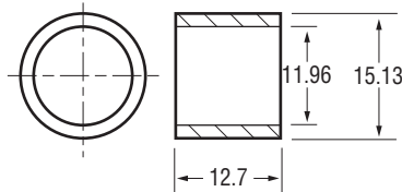
62-1403-1 Bushing - D.E. .0025" (1X) Undersize
