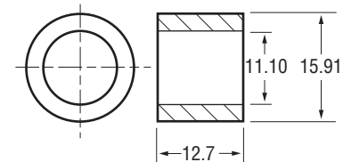
62-1408-1 Conversion Bushing - D.E. .0025" (1X) Undersize
