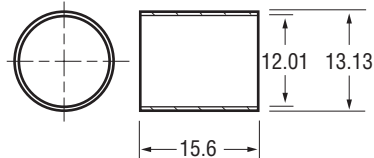
62-2404 Bushing - D.E.
