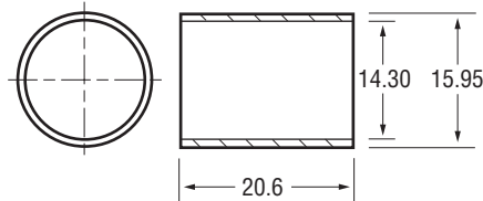
62-1502 Bushing - C.E.
