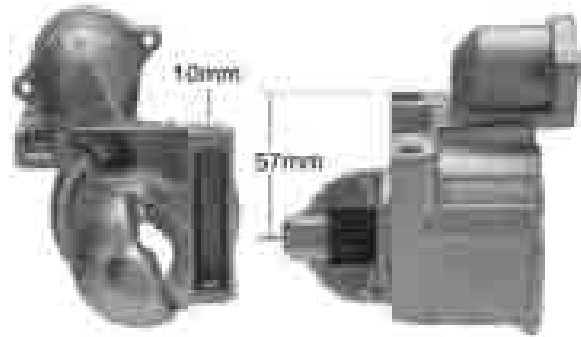
51-105-3 D.E. Housing 'No Shim' Version Aluminum
