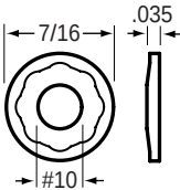
84-4311 Conical Washer Dim: #10 ID x 7/16 OD x .035 T
