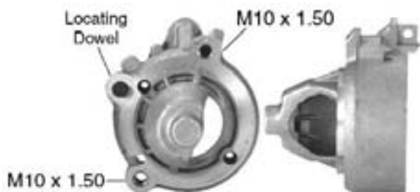
51-230 D.E. Housing Aluminum
