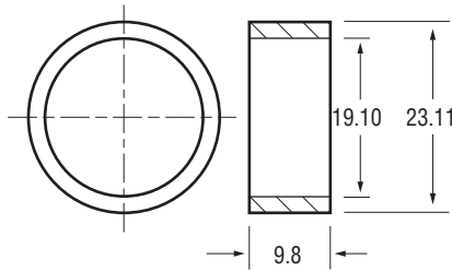
62-91701 Bushing - C.S.
