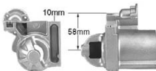
51-1108 D.E. Housing Aluminum
