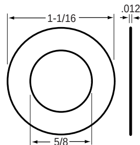
84-4616 Flat Washer
