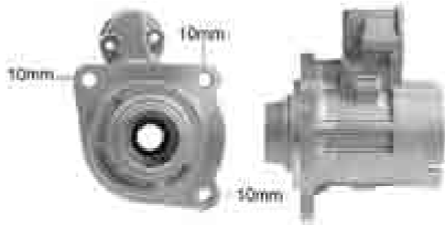
51-8305 D.E. Housing Aluminum
