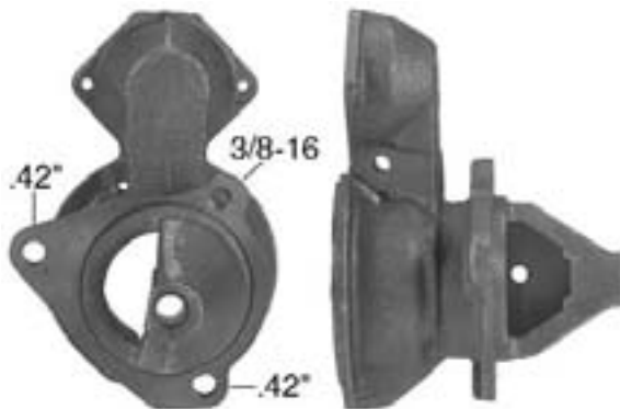
51-130 D.E. Housing Cast Iron
