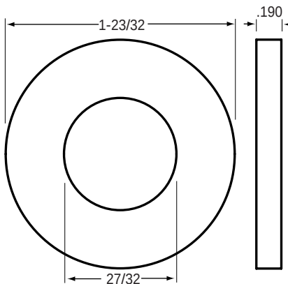
84-4702 Flat Washer
