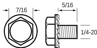
84-1411 Screw
