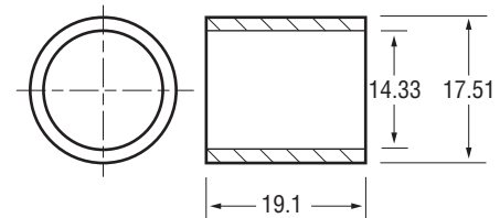
62-1505 Bushing - C.E.
