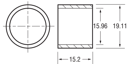
62-2600 Bushing - C.E.
