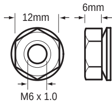
85-2310 Hex Nut
