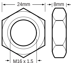
85-2600 Hex Nut
