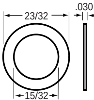
84-4503 Flat Washer
