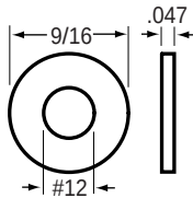
84-4306 Flat Washer Dim: #12 ID x 9/16 OD x .047 T Features: • Zinc-plated
