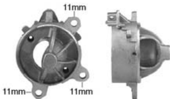
51-209 D.E. Housing Aluminum
