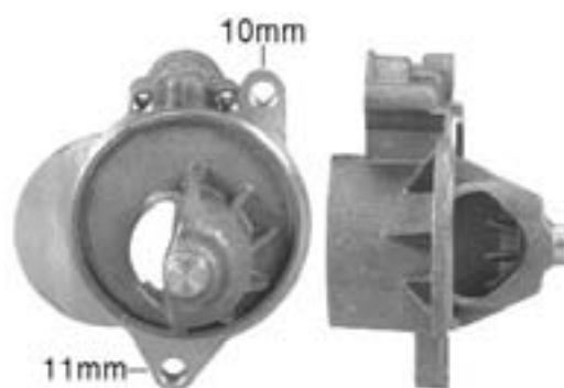
51-257 D.E. Housing Aluminum
