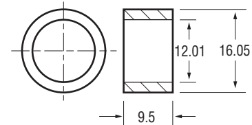
62-83404 Bushing - C.E.
