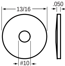
84-4310 Conical Washer Dim: #10 ID x 13/16 OD x .050 T Features: • Zinc-plated
