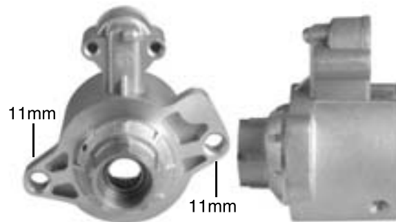
51-263 D.E. Housing Aluminum
