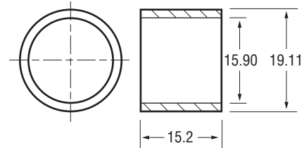
62-2600-1 Bushing - C.E. .0025" (1X) Undersize
