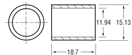
62-2400-1 Bushing - D.E. .0025" (1X) Undersize
