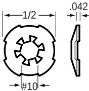
84-4305 Internal Tooth Square Conical Lock Washer Dim: #10 ID x 1/2 OD x .042 T Features: • Black oxide finish
