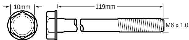
85-1315 Thru Bolt
