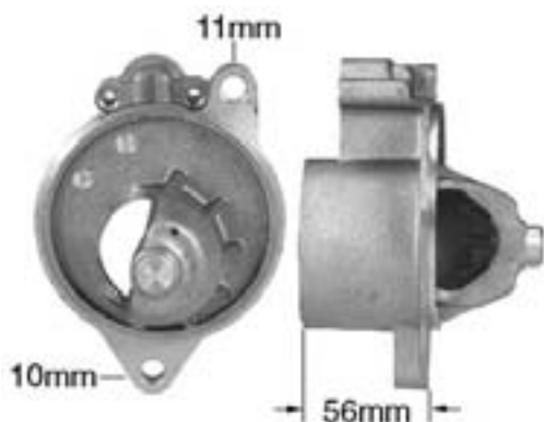
51-247 D.E. Housing Aluminum
