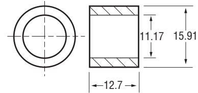
62-1408 Conversion Bushing - D.E.
