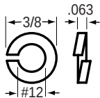
84-4307 Split Lock Washer Dim: #12 ID x 3/8 OD x .063 T Features: • Zinc-plated
