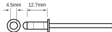
85-3200 Blind Rivet
