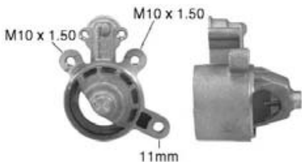
51-253 D.E. Housing Aluminum
