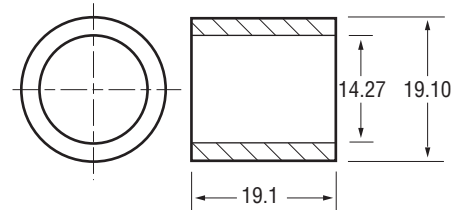
62-1504-1 Bushing - D.E., C.E. .0025" (1X) Undersize
