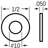
84-4304 Flat Washer Dim: #10 ID x 1/2 OD x .050 T Features: • Zinc-plated
