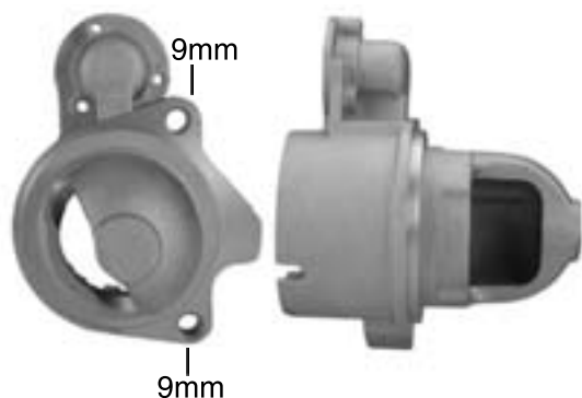
51-1140 D.E. Housing Aluminum
