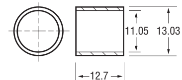
62-83405 Bushing - C.S.
