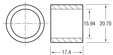
62-2601 Bushing - D.E.
