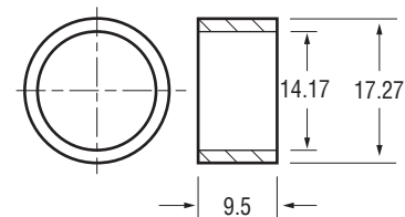
62-83500 Bushing - C.E.
