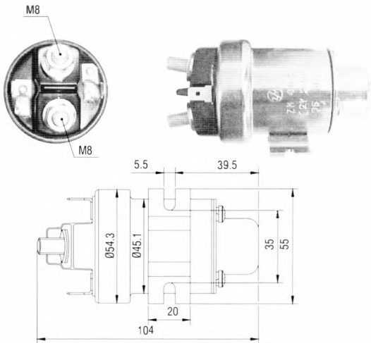
Insulated COIL (Bobina isolada) Permanent current 200 Amp. (Uso continuo 200 Amp.) Short time current 800 Amp(5 Sec.) (Uso max. 5 Seg. 800 Amp.)
