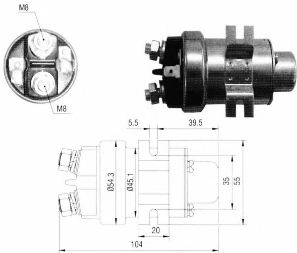
Insulated COIL (Bobina isolada) Permanent current 200 Amp. (Uso continuo 200 Amp.) Short time current 800 Amp(5 Sec.) (Uso max. 5 Seg. 800 Amp.)
