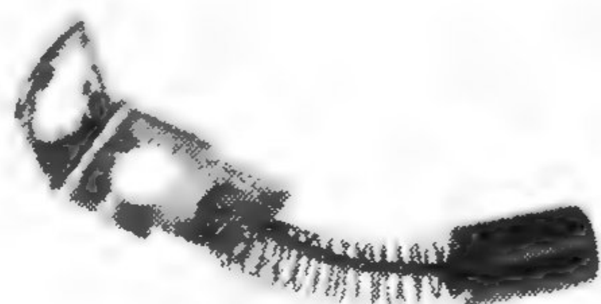
CH-1-R .375 x .250 x .675 Ground REPLACES: 2095039
