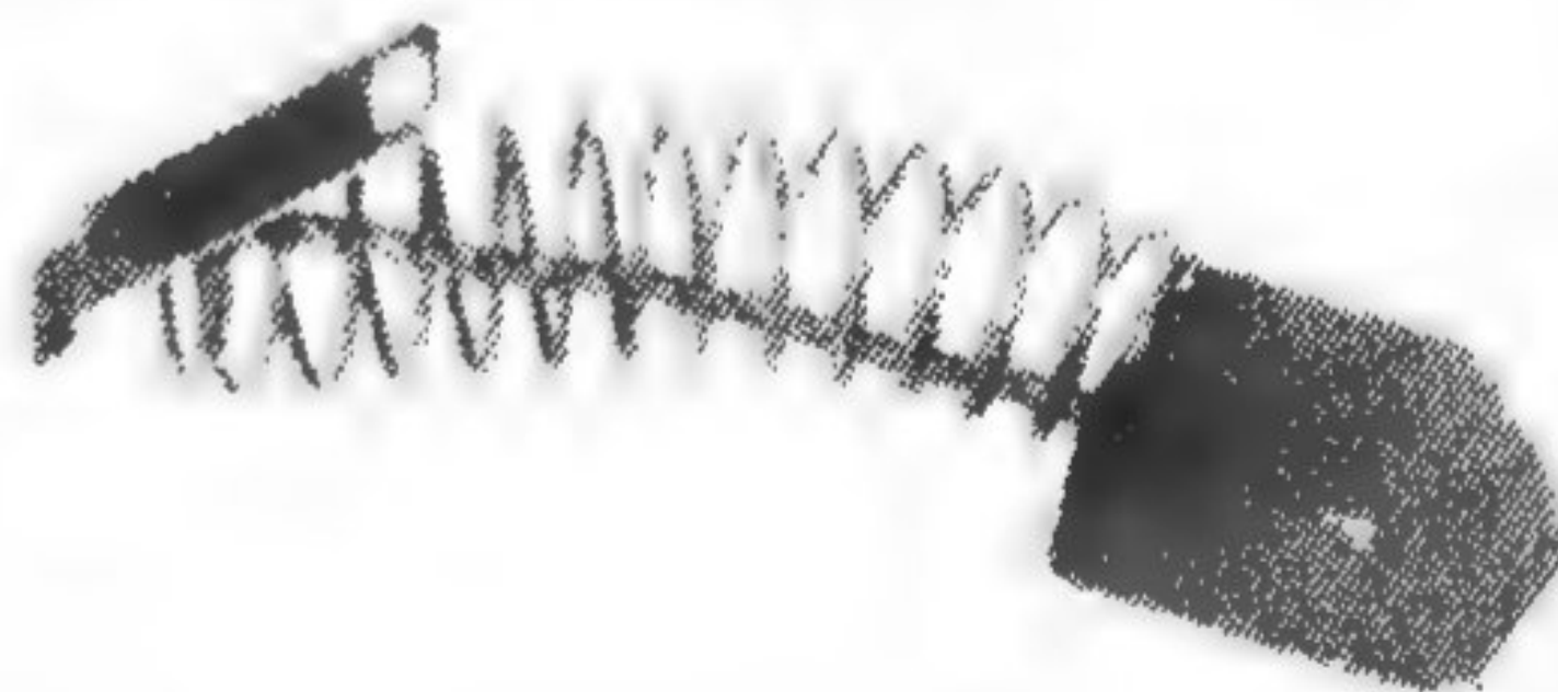
H-4 .812 x .498 x .373 x 1.625 REPLACES: 1669-32A
