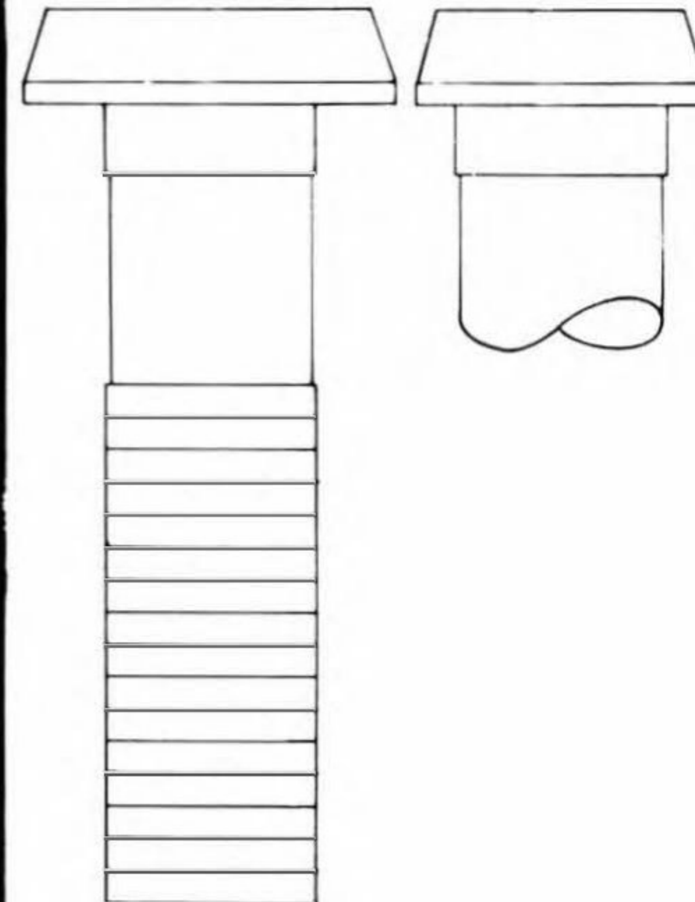
13212 1/2-13 x 1-7/8 Flat Rectangular Head Stepped Shoulder Copper
