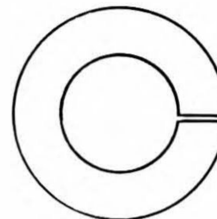
S-264 1/2 I.D. 7/8 O.D. .105 THK. Zinc Plated
