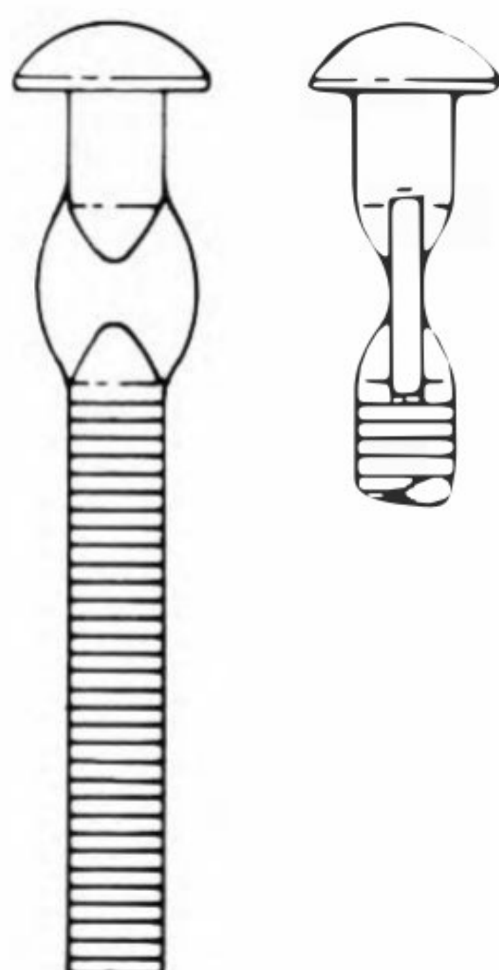
S-1265 10-32 x 1-1/2 Round Head Flange Locking Shoulder Zinc Plated
