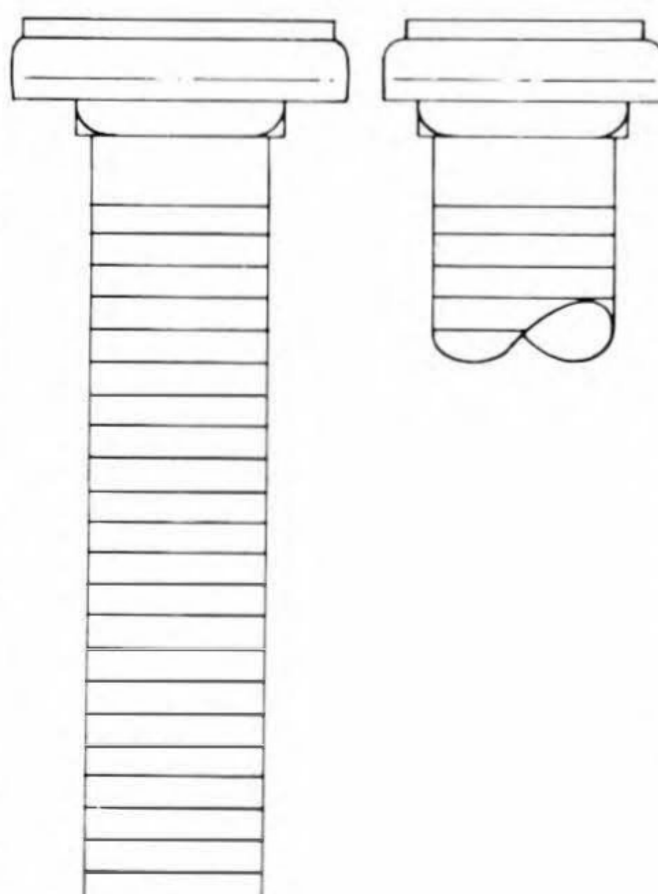
S-1552 1/2-13 x 1-7/8 Flat Rectangular Head Inlaid Silver Alloy Contact Stepped Shoulder (Square) Copper
