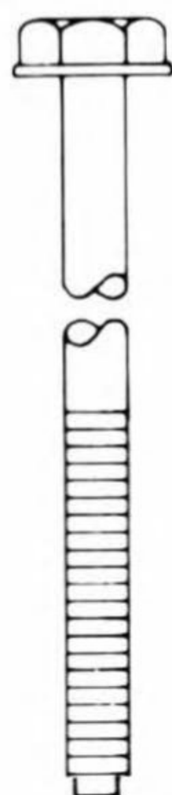
S-1312 10-24 x 2-1/8 Hex Washer Head Dog Point Zinc Plated
