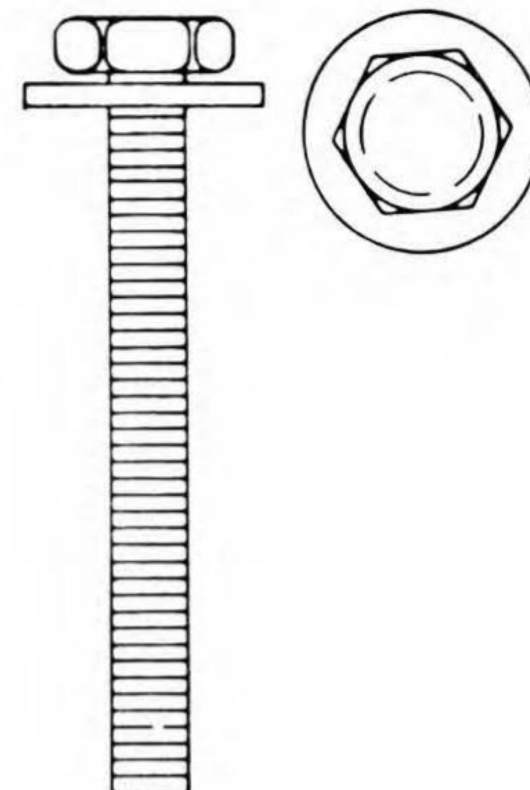
S-3417 10-24 x 1-3/4 Hex Head Attached Lockwasher Zinc Plated
