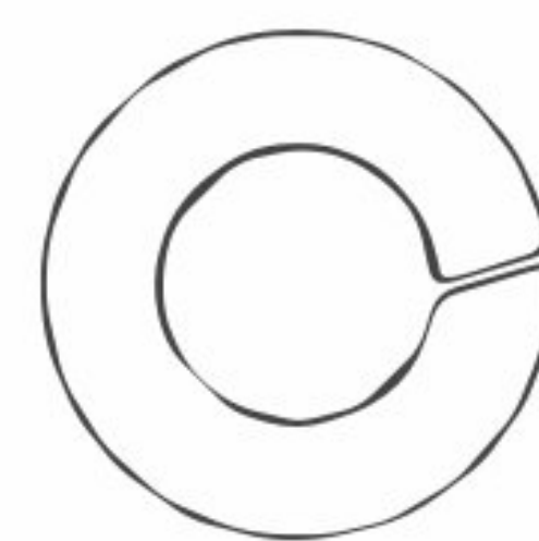
S-258 5/16 I.D. 9/16 O.D. .080 THK. Zinc Plated
