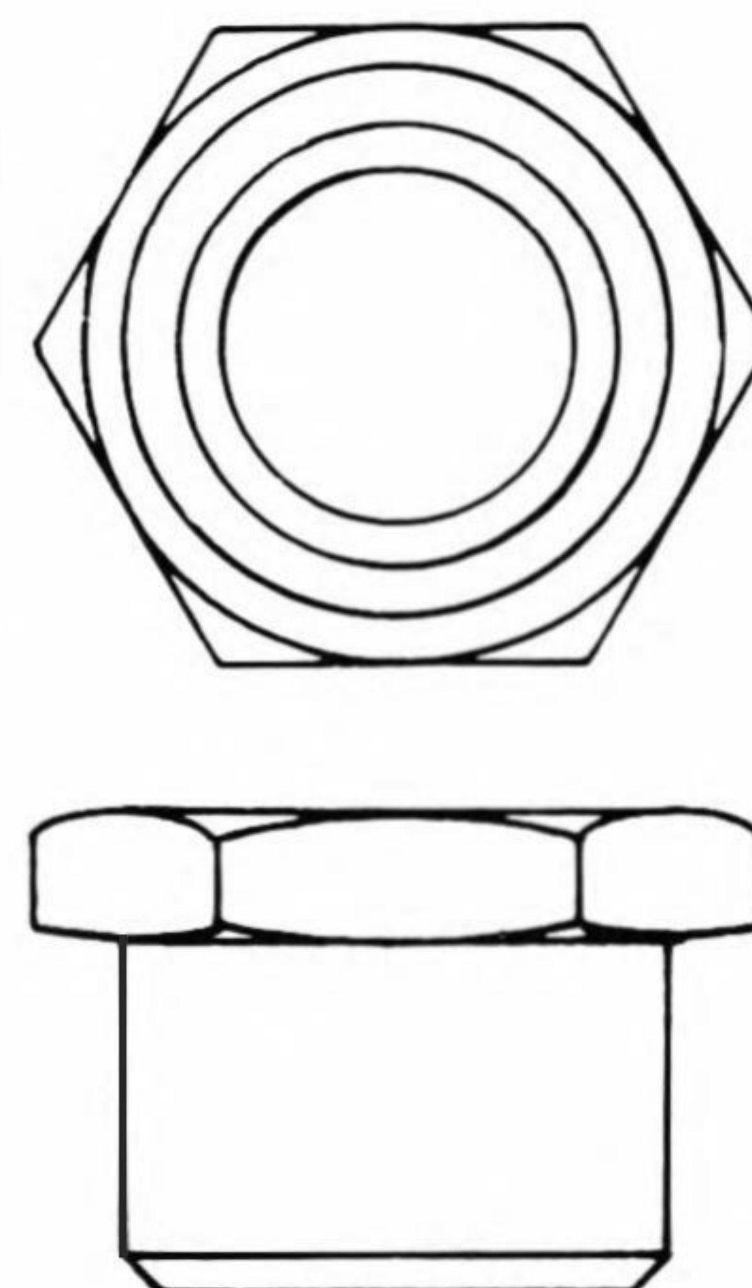
S-1342 .668-20 x 1-1/8 Extended Hex .845 Thk. Plain Finish
