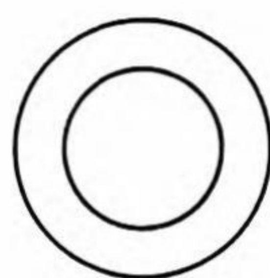
13112 3/8 I.D. 5/8 O.D. .030 Thk. Fiber
