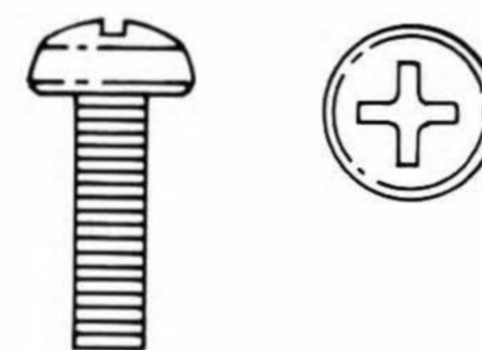
S-3975 M 5 x 0.8 x 15.7 mm Fillister Head, Phillips Zinc Plated
