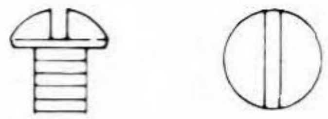
S-101 6-32 x 5/32 Slotted Round Head Zinc Plated
