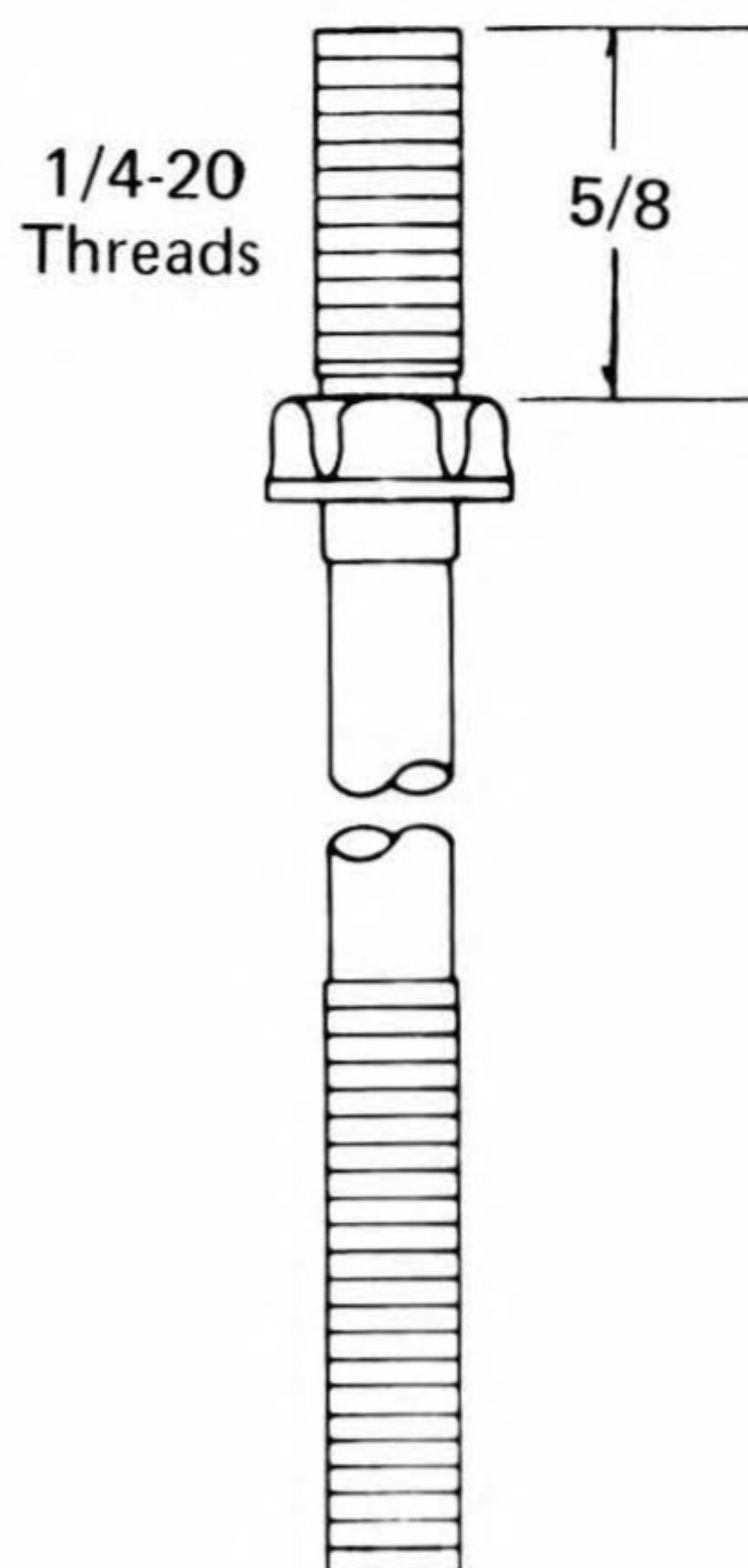
S-2051 1/4-20 x 5-7/8 Hex Washer Head Extension Bolt Plain Finish
