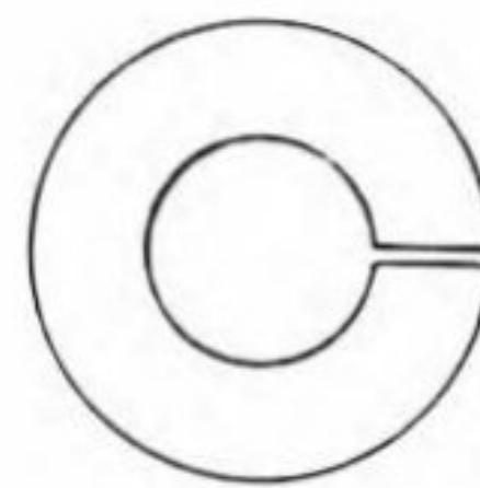
S-256 1/4 I.D. 1/2 O.D. .055 THK. Zinc Plates
