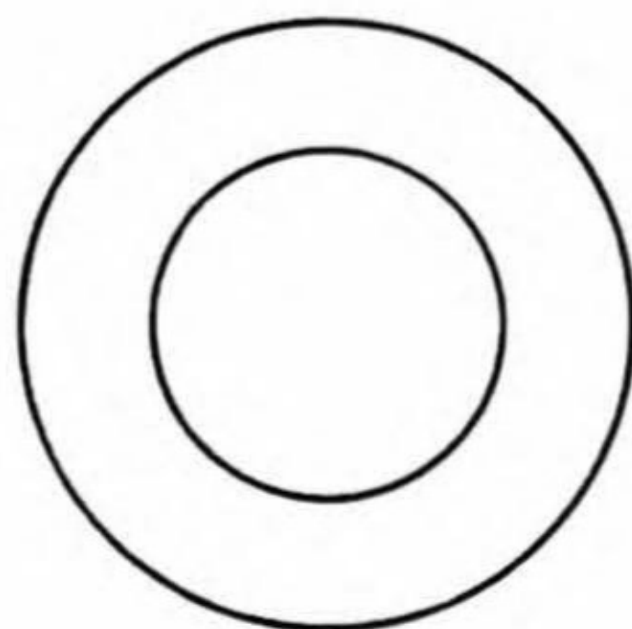
S-853 5/8 I.D. 1-1/16 O.D. .100 Thk. Zinc Plated
