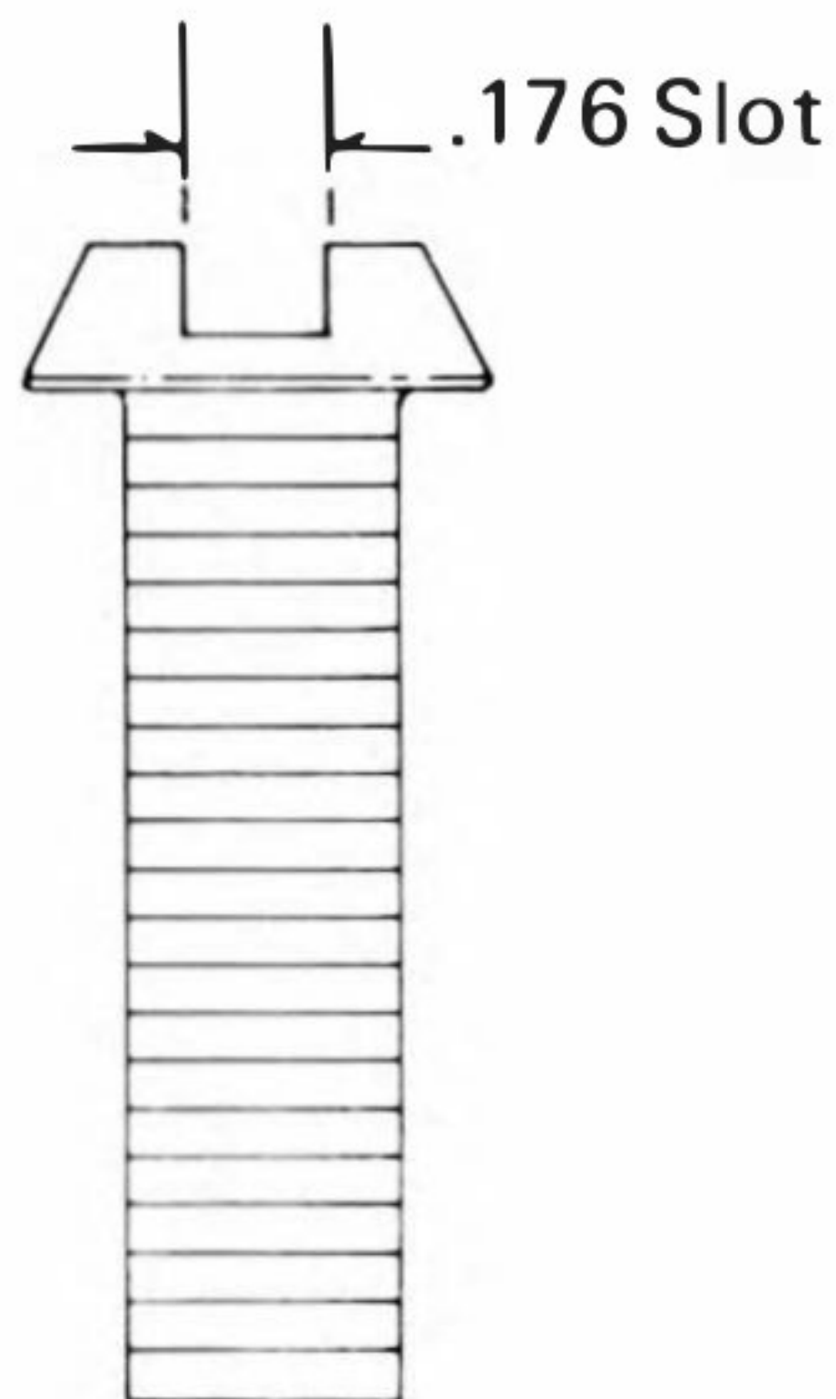
S-864 3/8-16 x 1-3/8 Tapered Pan Head Slotted Copper
