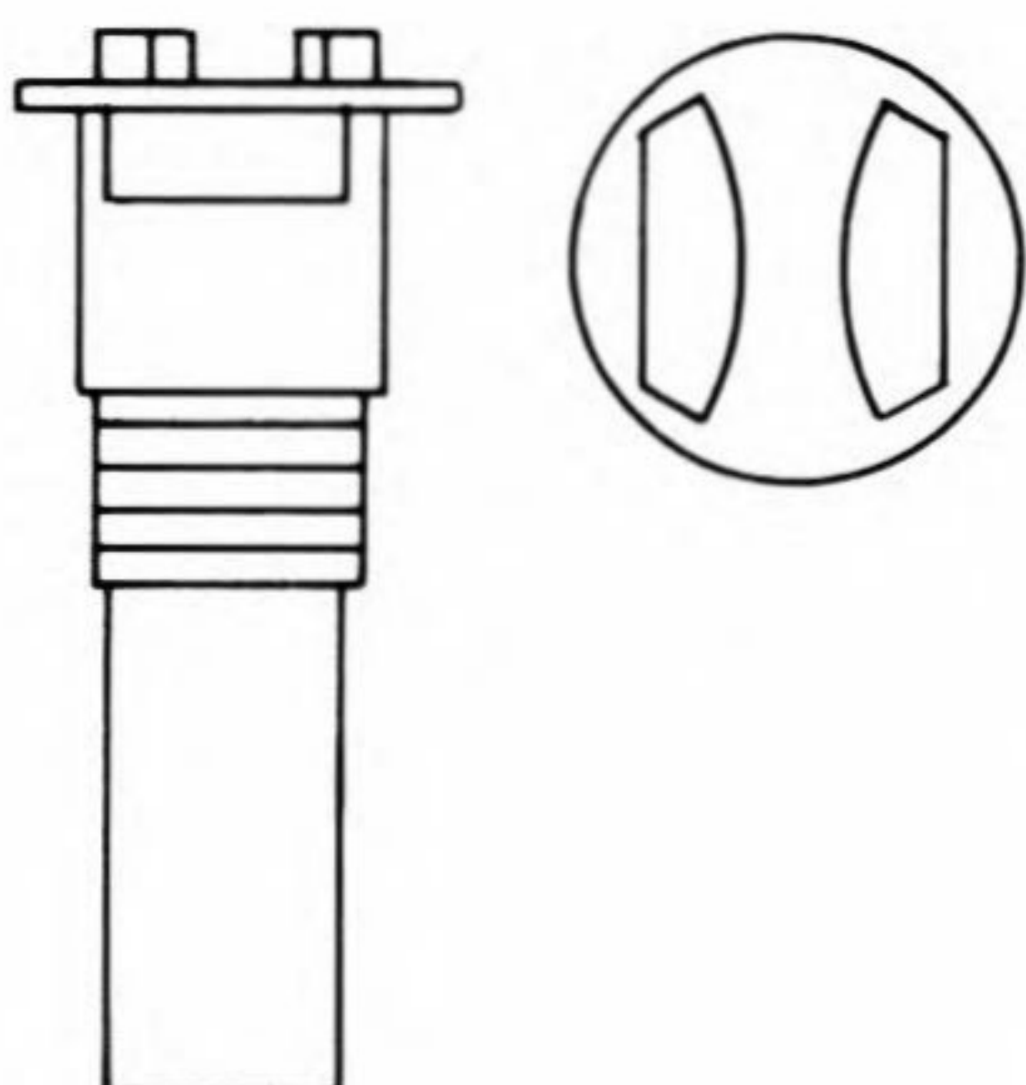
13140 3/8-16 x 1-9/32 Tapped 10-32 Shank Flat Slotted Extension Head Stepped Shoulder (Rectangular) Copper
