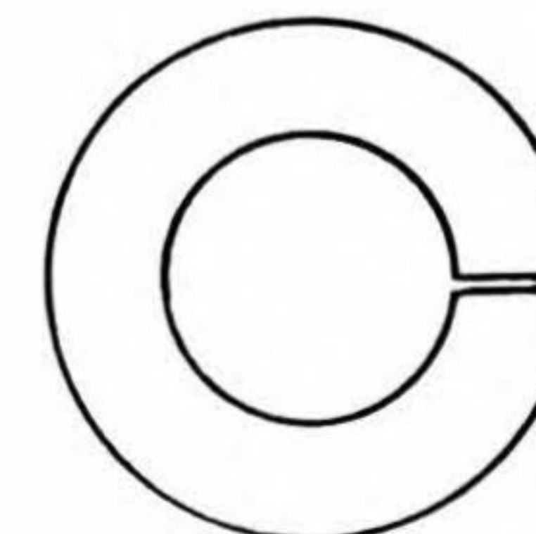
13181 1/2 I.D. 7/8 O.D. .103 THK. Zinc Plated
