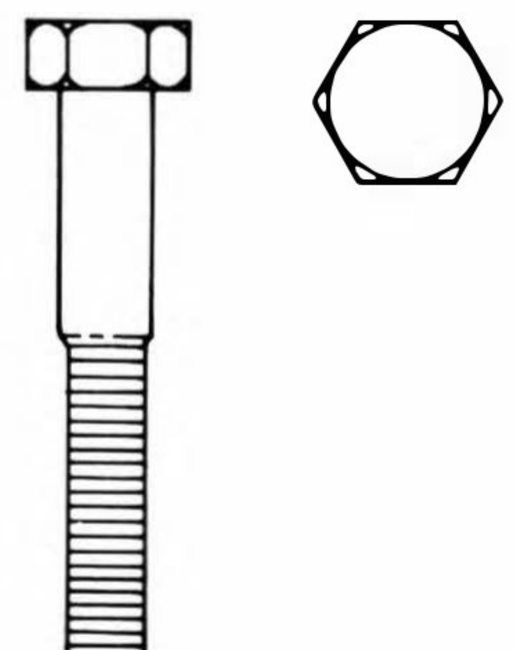
S-3871 M 6 x 1.0 x 35.0 mm Hex Head Zinc Plated
