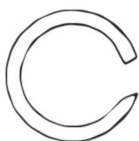
S-1857 .439 I.D. .557 O.D. .064 Thk. Plain Finish
