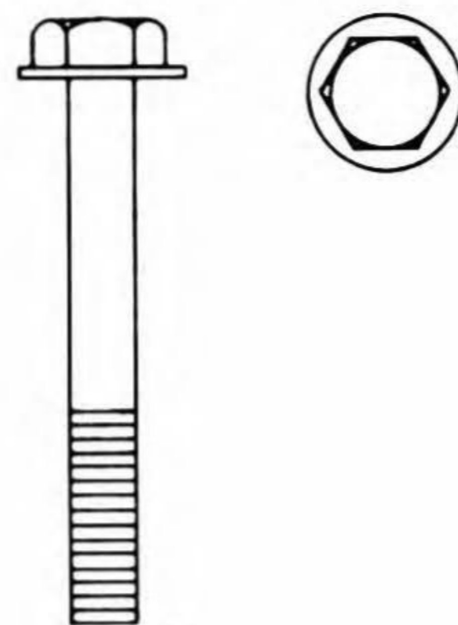
S-2346 10-24 x 1.312 Grade-5 Hex Washer Head Zinc Plated
