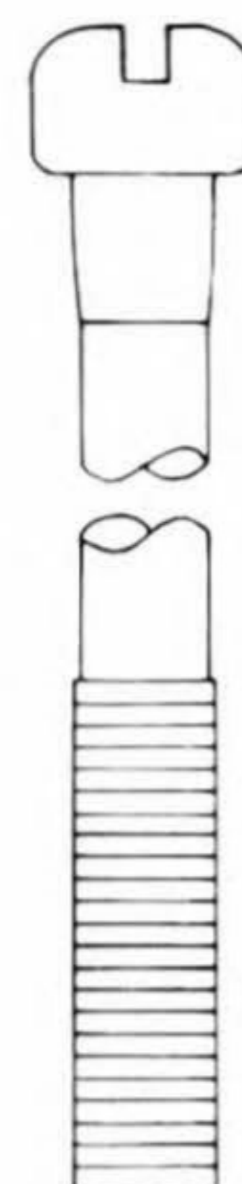
S-2656 1/4-26 x 6 Slotted Round Head Plain Finish
