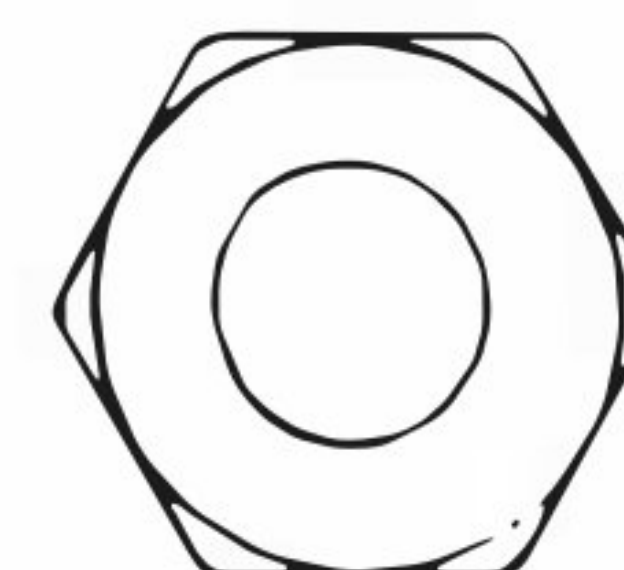
13113 3/8-16 x 5/8 Hex .160 Thk. Zinc Plated
