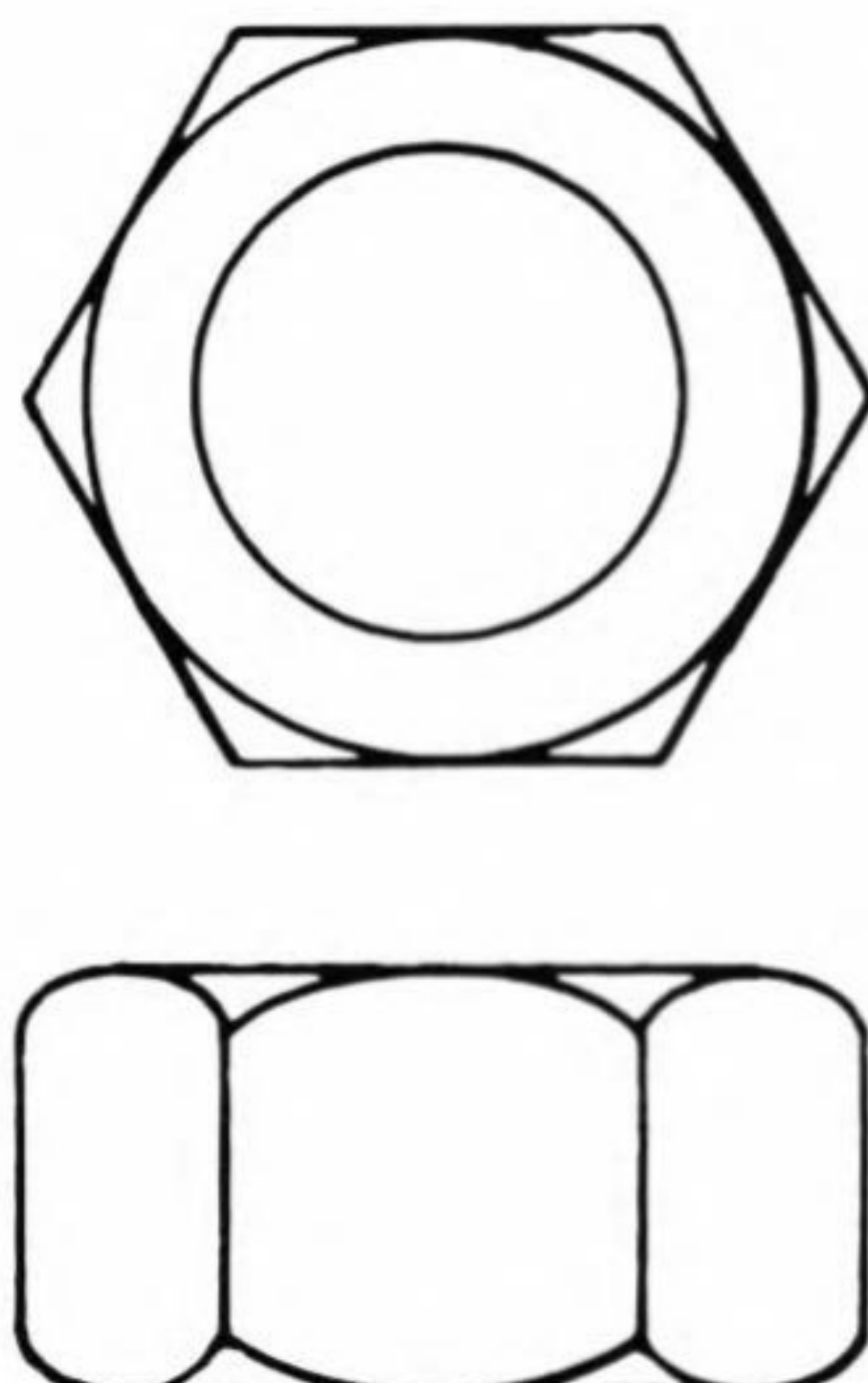
S-2020 5/8-18 x 15/16 Hex .549 Thk. Locknut Zinc Plated
