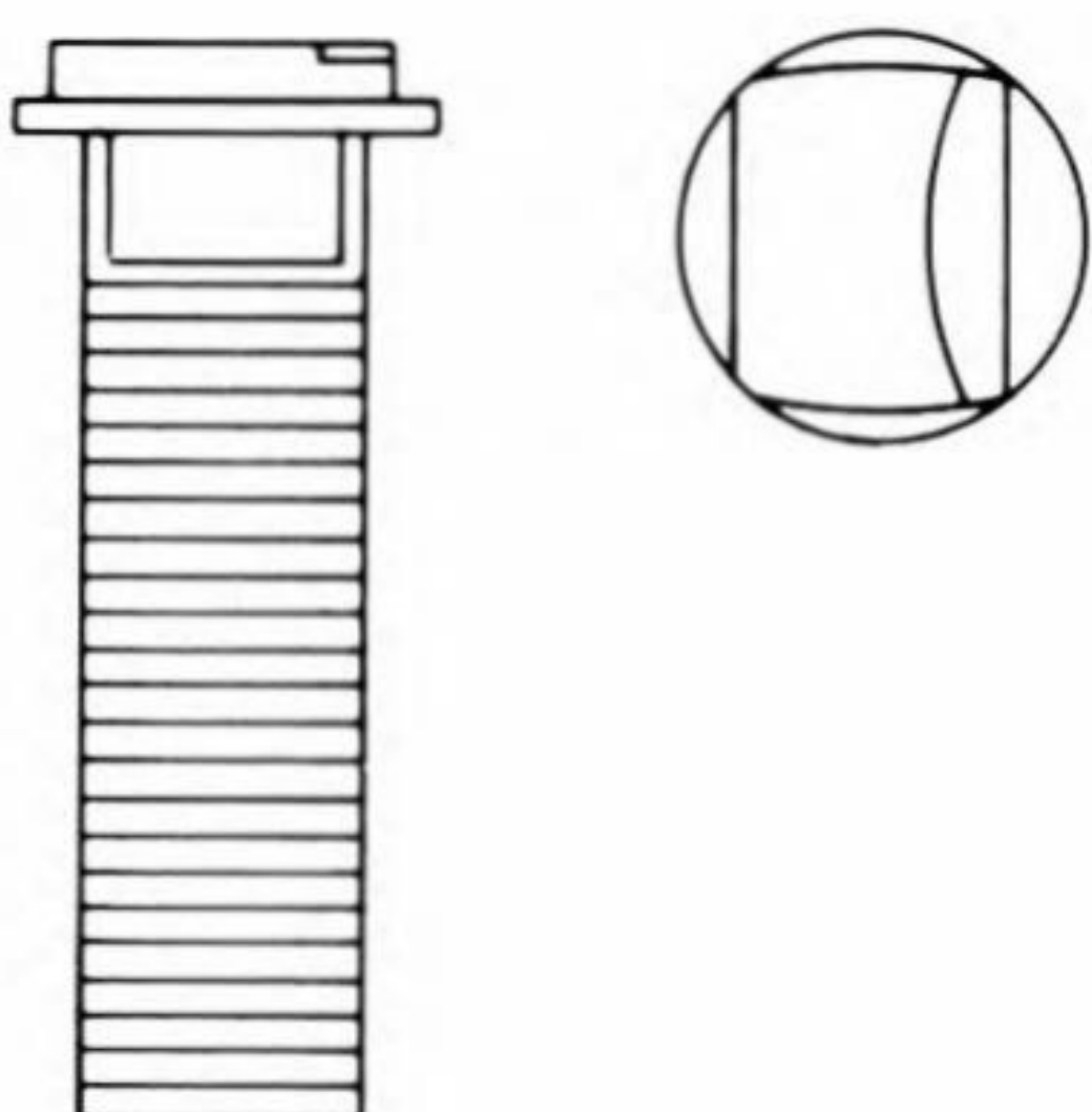
13246 3/8-16 x 1-3/16 Flat Head, Oval Crown Inlaid Silver Alloy Contact Stepped Shoulder (Rectangular) Copper
