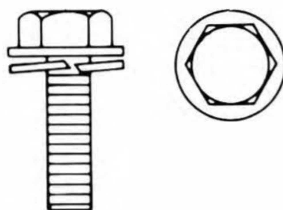
S-2324 10-24 x .750 Hex Washer Head Attached Lockwasher TAPTITE® Thread Zinc Plated
