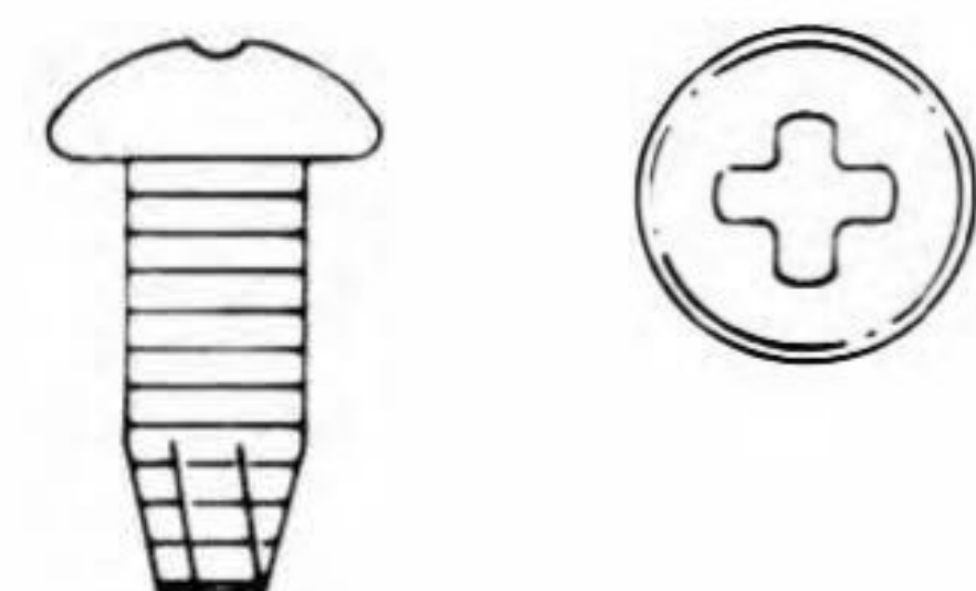
S-2547 10-24 x 5/8 Oval Phillips Head Thread Cutting Black Phosphate
