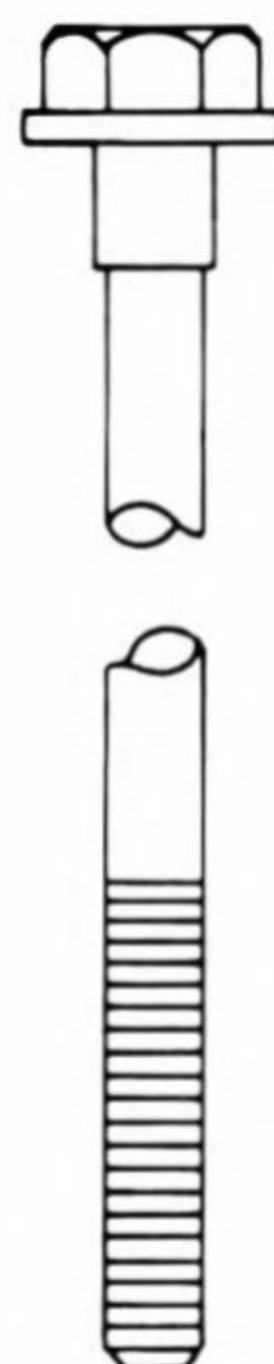
S-2312 10-24 x 5-7/8 Hex Washer Head Plain Finish
