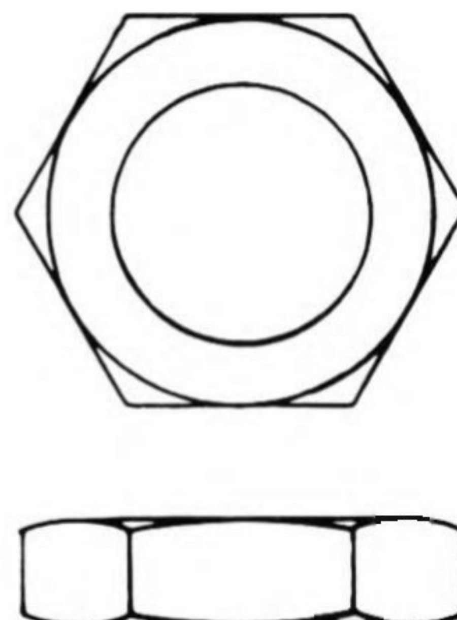
S-212 .668-20 x 15/16 Hex with Right Hand Threads .307 Thk. Zinc Plated
