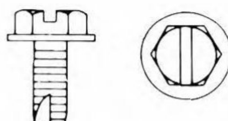
S-2426-H 8-32 x 3/8 Slotted Hex Washer Head Thread Cutting Zinc Plated
