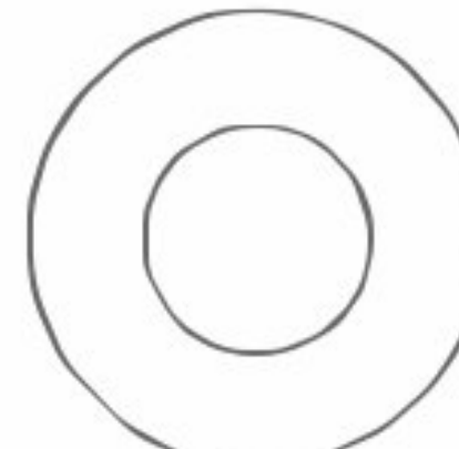
S-349 1/4 I.D. 1/2 O.D. .030 Thk. Zinc Plated
