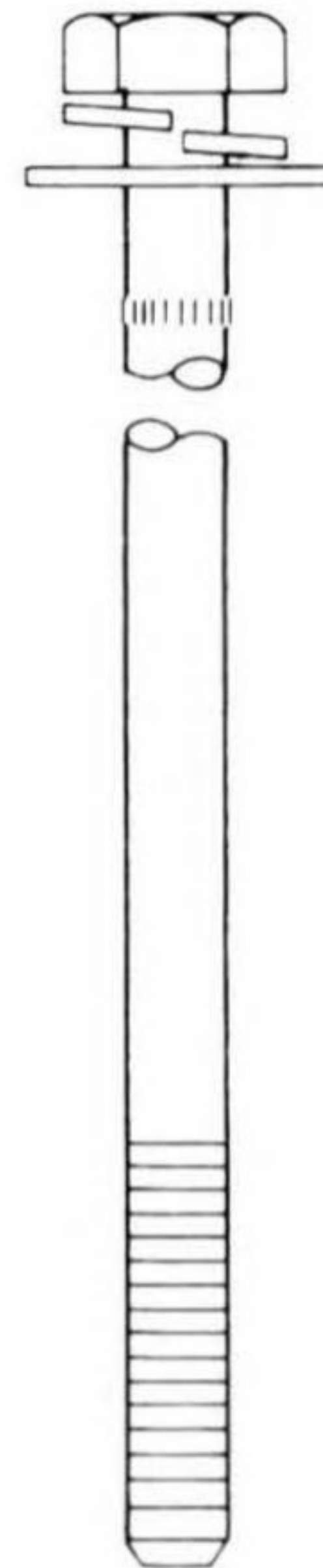
S-5144 M 6 x 1.0 x 139.0 mm Hex Head Attached Lock & Flat Washers Knurled Shoulder Zinc Plated
