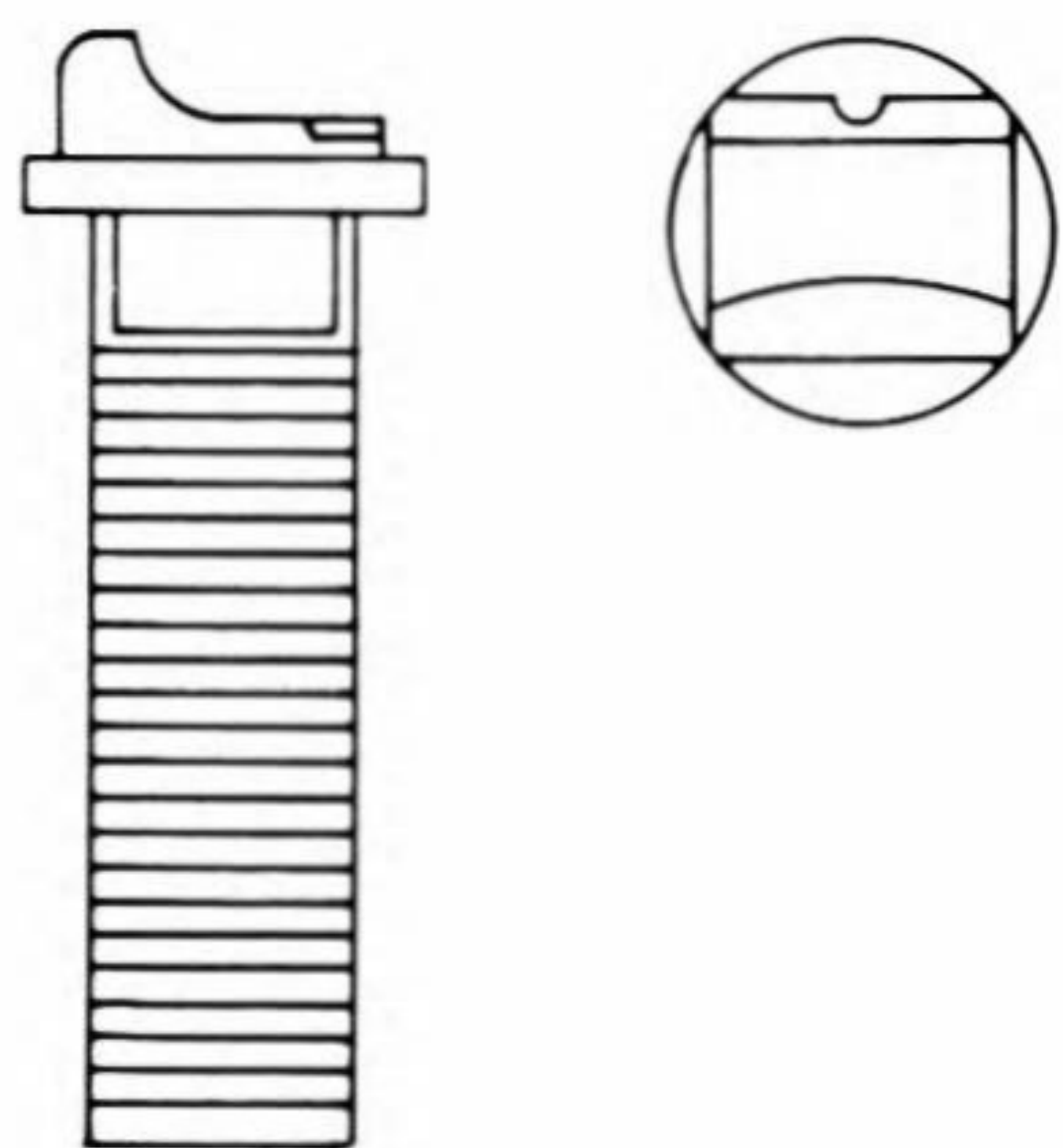
13245 3/8-16 x 1-3/16 Flat Head, Square Crown with Raised Side Inlaid Silver Alloy Contact Stepped Shoulder (Rectangular) Copper
