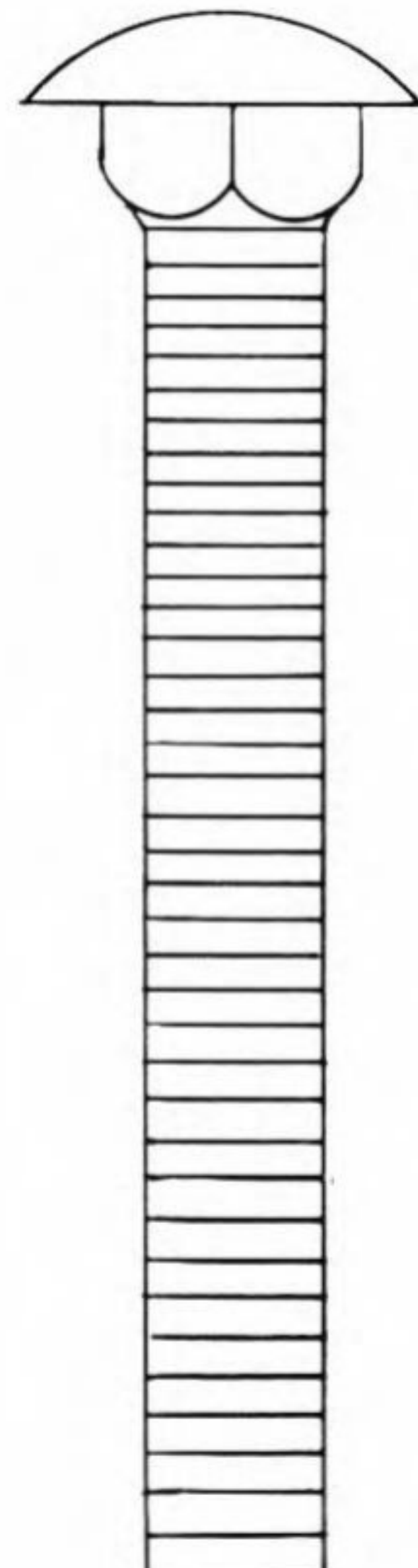
S-1432 5/16-18 x 2-1/2 Round Head Square Shoulder Zinc Plated
