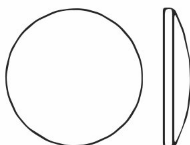
S-881 1 1/16" Dia. .049 Thk. Plain Finish
