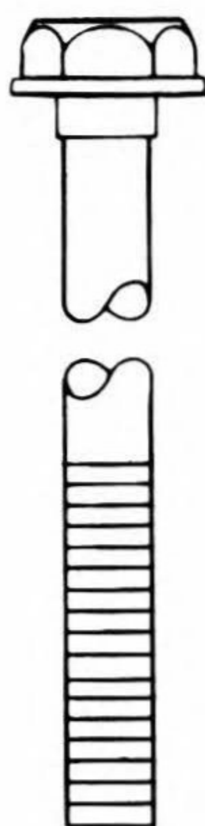
S-2470-L 1/4-20 x 5-27/64 Hex Washer Head Plain Finish
