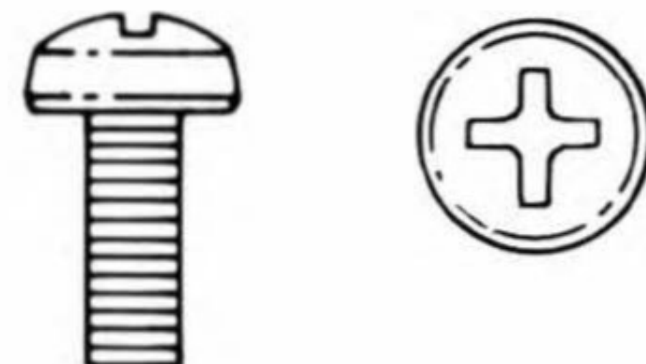
S-3974 M 5 x 0.8 x 12.0 mm Pan Head, Phillips Zinc Plated
