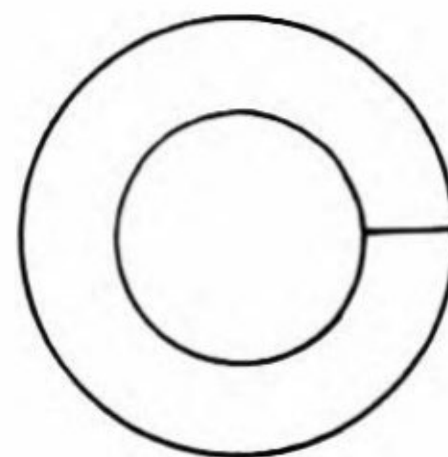
13277 5/16 I.D. 9/16 O.D. .060 THK. Zinc Plated
