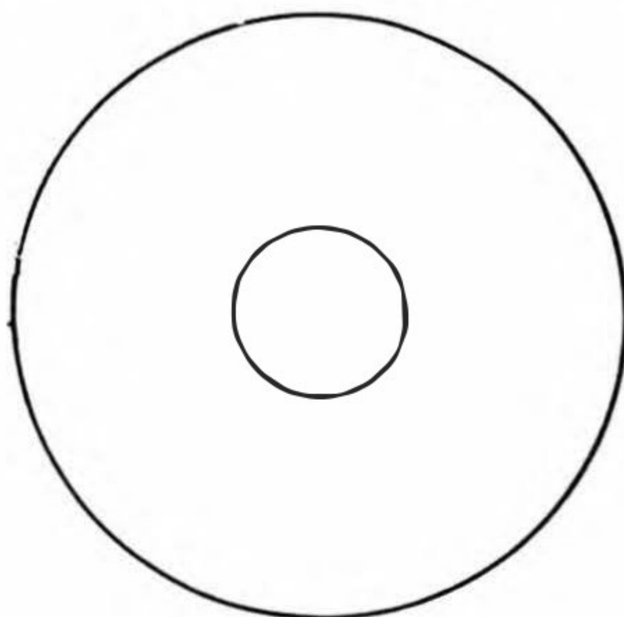
13204 1/2 I.D. 1-25/32 O.D. .095 Thk. Cadmium Plated Copper
