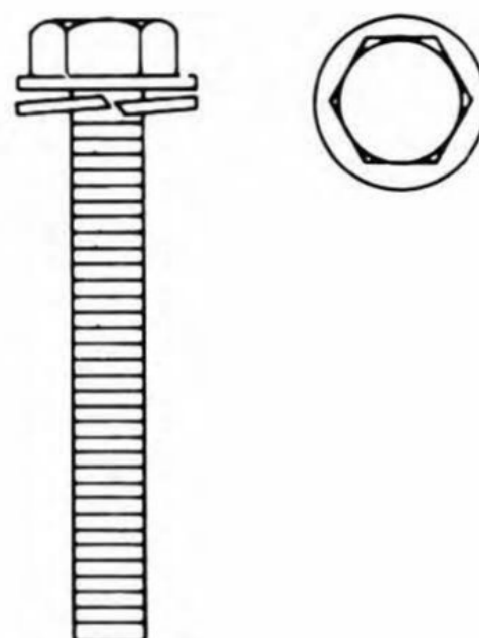
S-2325 10-24 x 1.375 Hex Washer Head Attached Lockwasher TAPTITE® Thread Zinc Plated
