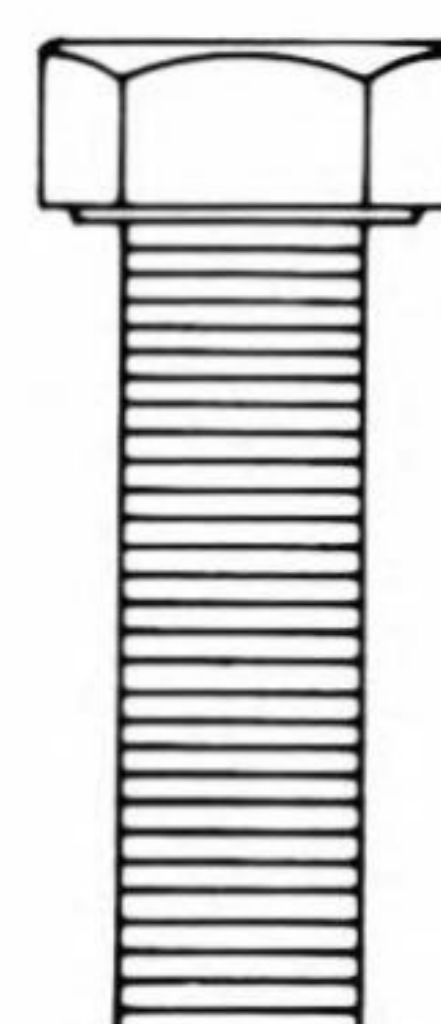
S-3978 M 8 x 1.25 x 24.5 mm Hex Head Black Oxide
