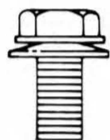
S-4201 10-24 x 3/8 Hex Washer Head Attached Conical Washer TAPTITE® Thread Black Phosphate
