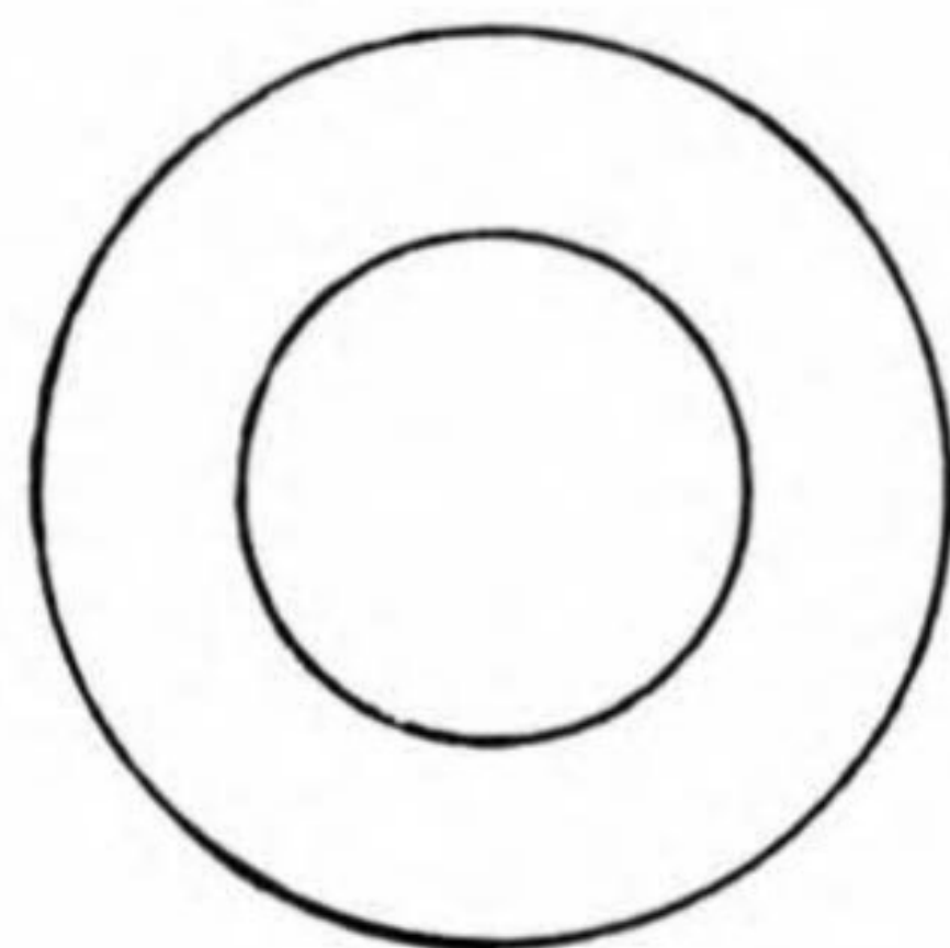
S-852 9/16 I.D. 1 O.D. .057 Thk. Black Oxide
