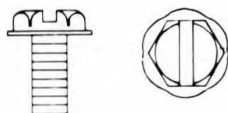
S-1262 10-24 x 3/8 Slotted Hex Washer Head Zinc Plated
