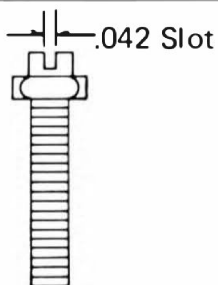
S-2490 8-32 x 3/4 Square Flat Head Cylindrical Crown Zinc Plated
