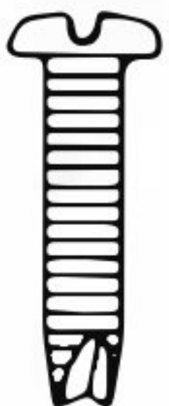
S-104 6-32 x 5/8 Slotted Pan Head Thread Cutting Zinc Plated
