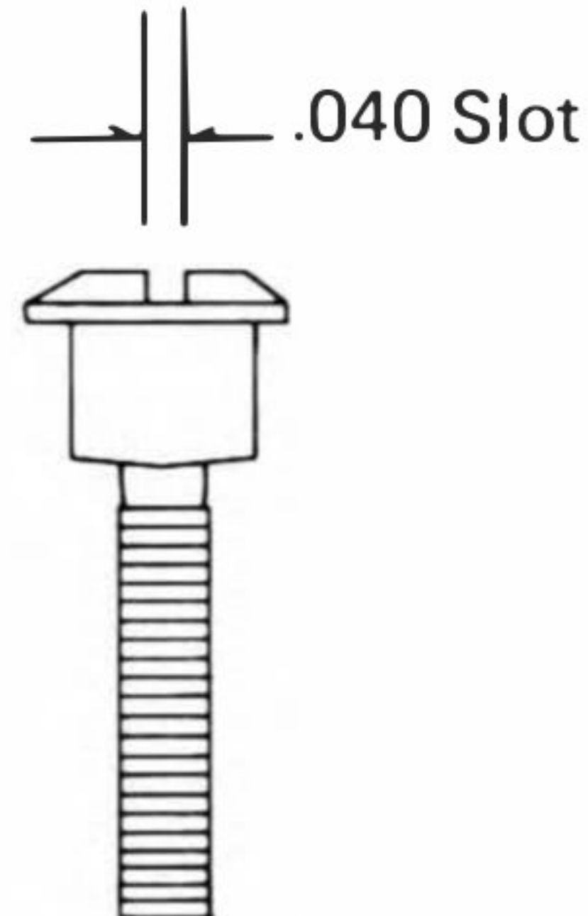
S-160 10-32 x 1 Pan Head Stepped Shoulder (Oval) Zinc Plated
