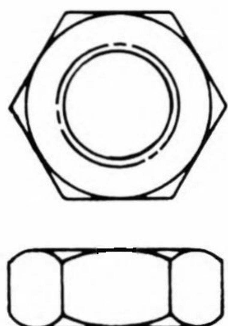
S-211 1/2-20 x 3/4 Hex .310 Thk. Zinc Plated
