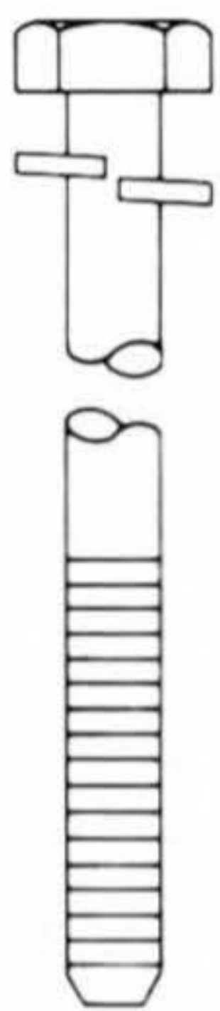
S-5086 M 5 x 0.8 x 151.5 mm Hex Head Attached Lockwasher Zinc Plated
