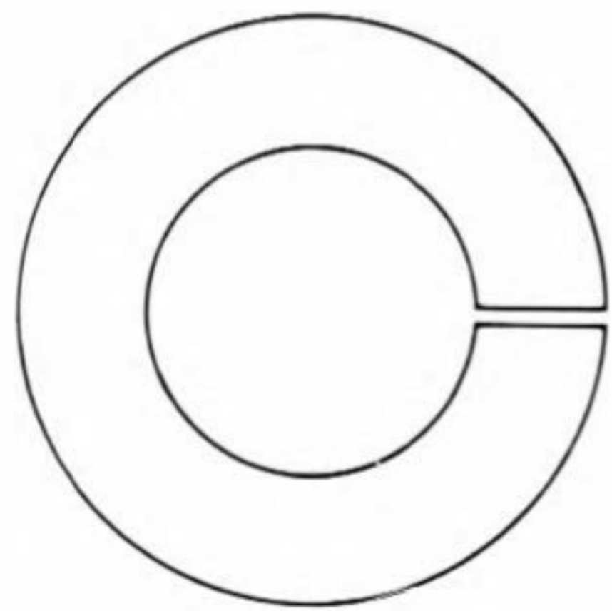
S-3990 9/16 I.D. 31/32 O.D. .113 Thk. Zinc Plated
