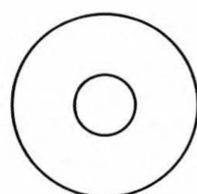
S-4991 1/4 I.D. 25/32 O.D. .029 Thk. Fiberglass
