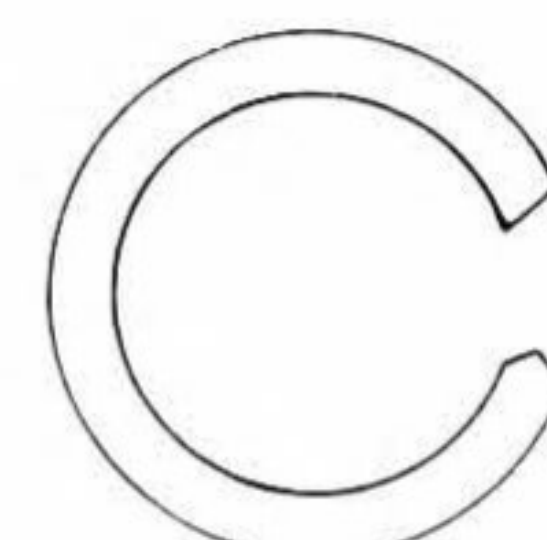
S-781 .505 I.D. .688 O.D. .096 Thk. Zinc Plated
