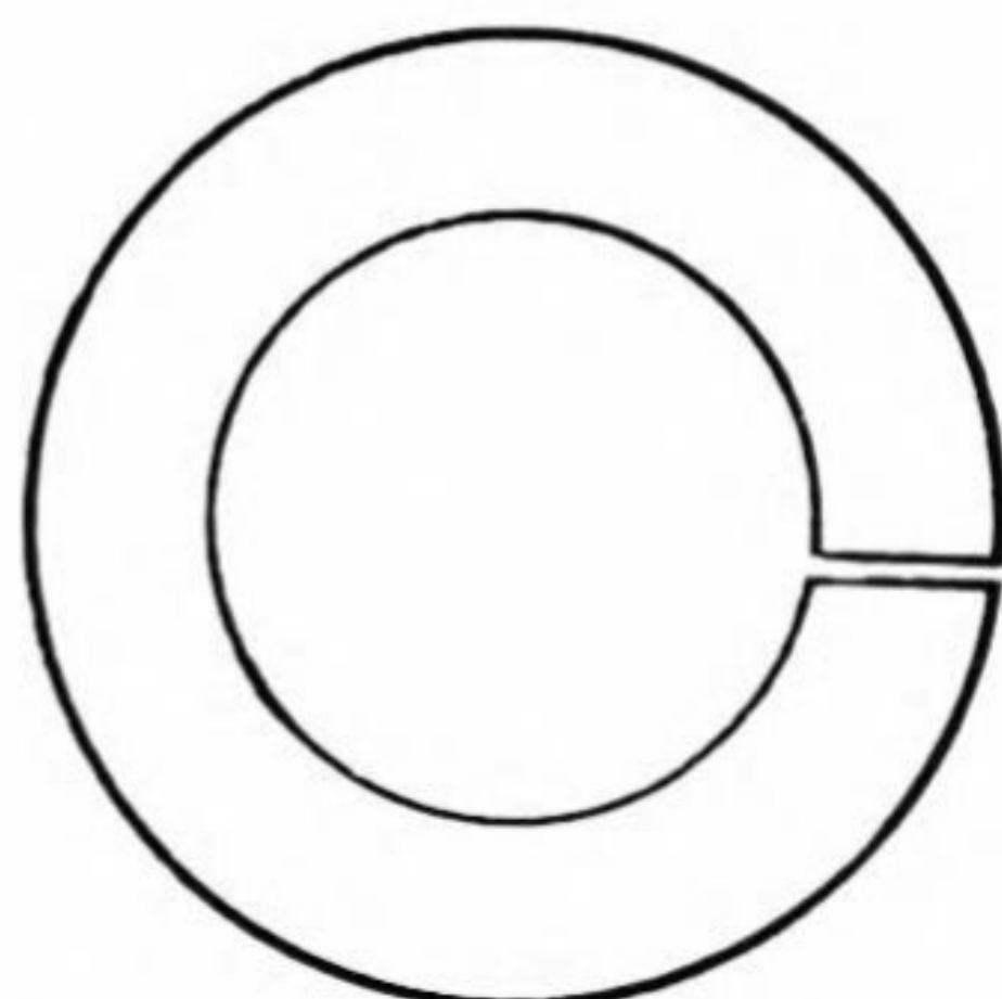
S-266 11/16 I.D. 1-1/16 O.D. .105 THK. Zinc Plated
