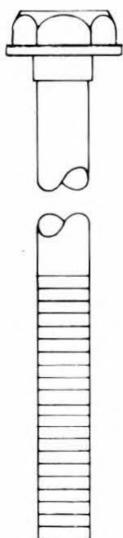
S-159 1/4-20 x 5-7/8 Hex Washer Head Plain Finish
