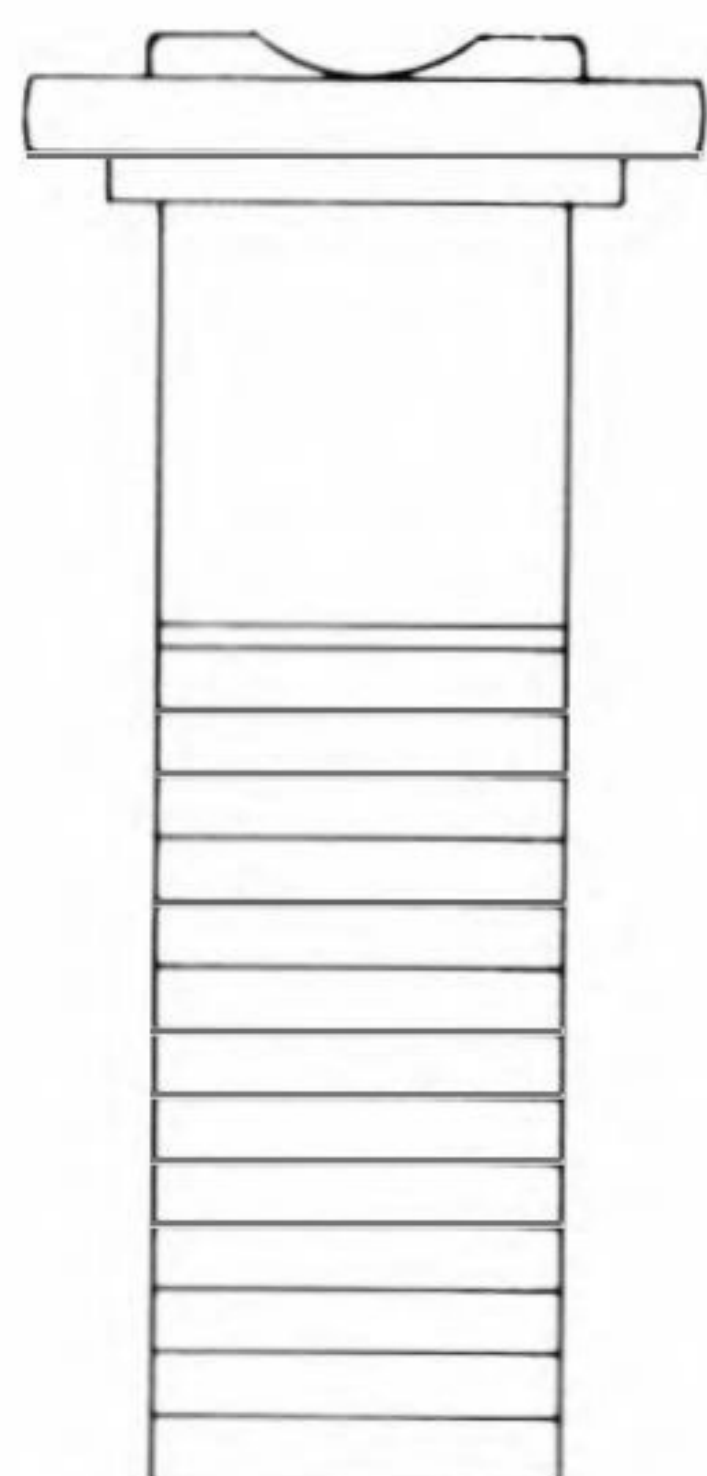
S-183 1/2-13 x 1-5/8 Flat Head Cylindrical Crown (Recessed) Stepped Shoulder (Oval) Copper
