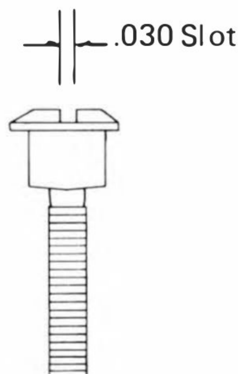
S-160-N 10-32 x 1 Pan Head Stepped Shoulder (Oval) Zinc Plated
