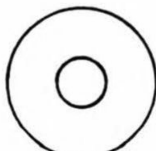
13128 7/32 I.D. 5/8 O.D. .063 Thk. Zinc Plated
