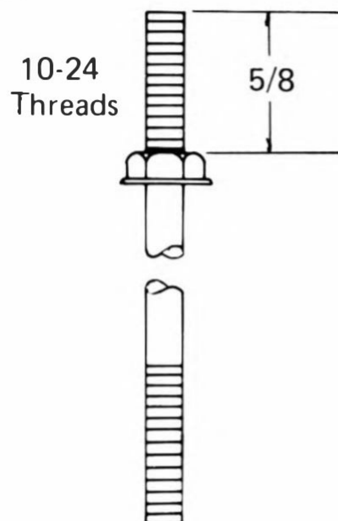
S-2306 10-24 x 5-7/8 Hex Washer Head Extension Bolt Plain Finish
