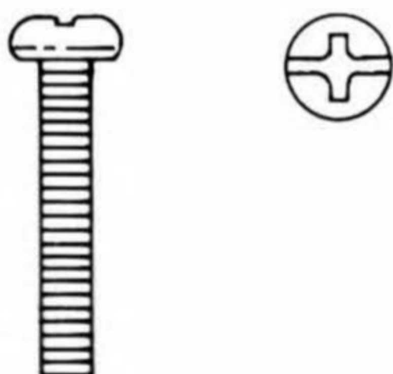
S-3856 M 4 x 0.7 x 19.0 mm Round Head Standard and Phillips Slot Zinc Plated
