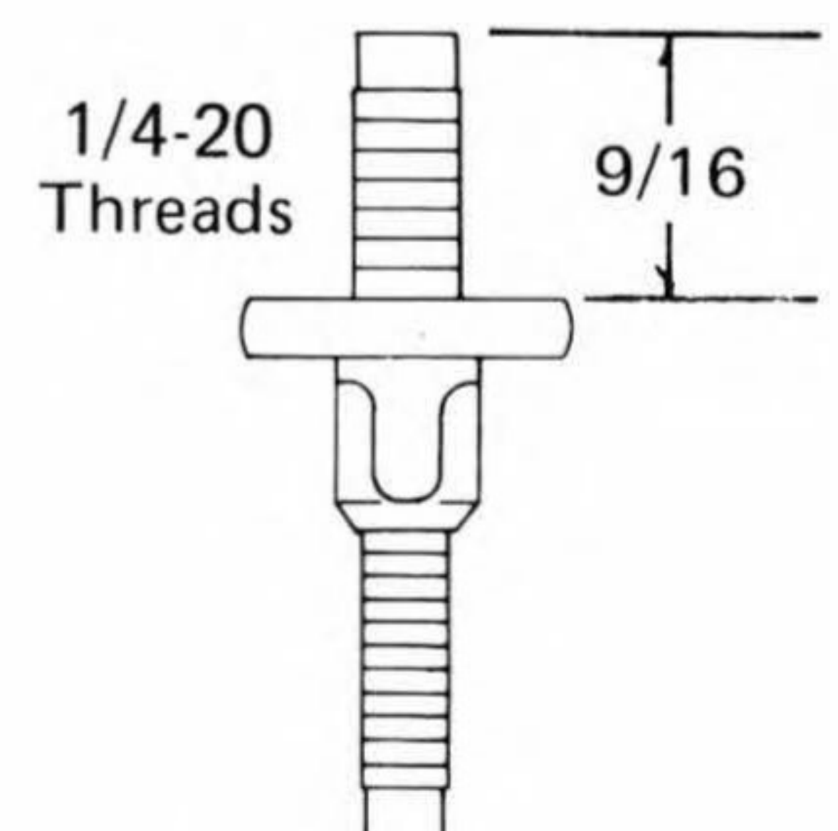
S-2541 10-24 x 7/8 Flat Extension Head Square Shoulder Dog Point Zinc Plated
