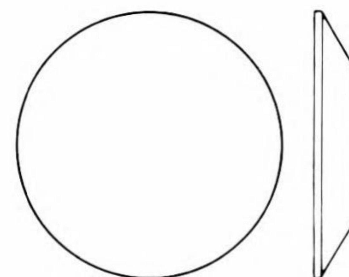
S-2003 1.035 Dia. .135 Depth .032 Thk. Plain Finish
