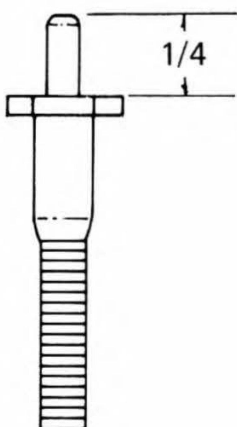
S-2236 8-32 x 31/32 Hex Extension Head Stepped Shoulder Zinc Plated
