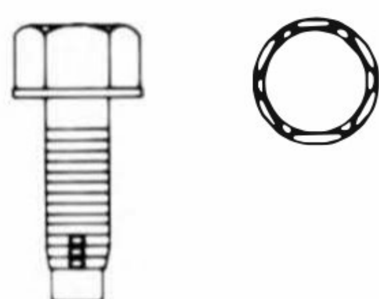
S-4254 10-32 x 5/8 Hex Washer Head Thread Forming Black Phosphate
