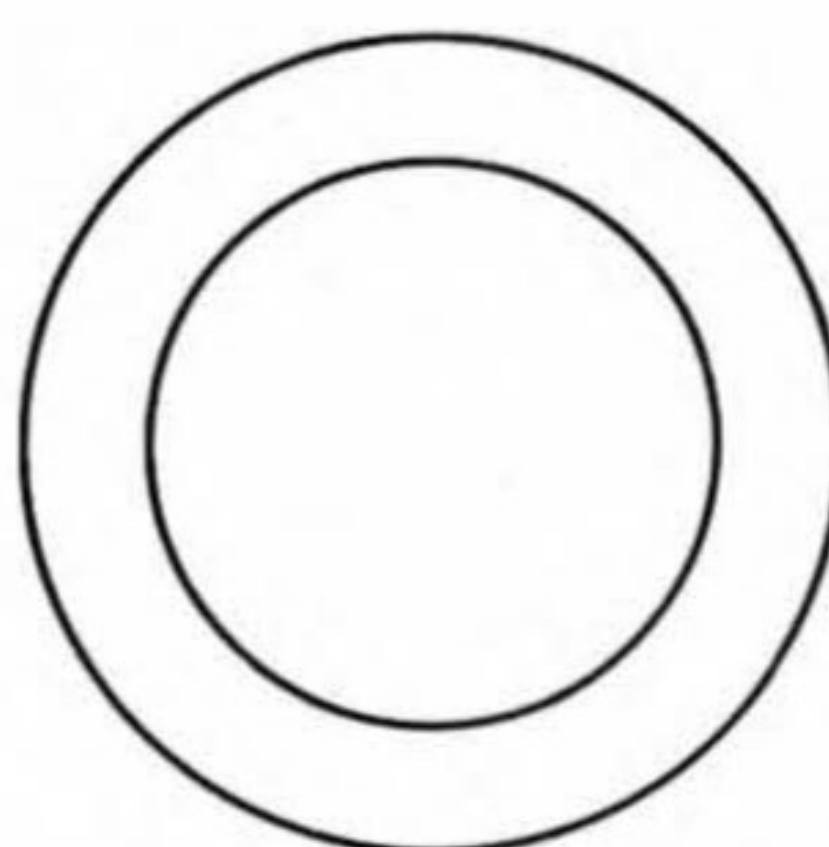
S-4511 11/16 I.D. 1 O.D. .063 Thk. Zinc Plated
