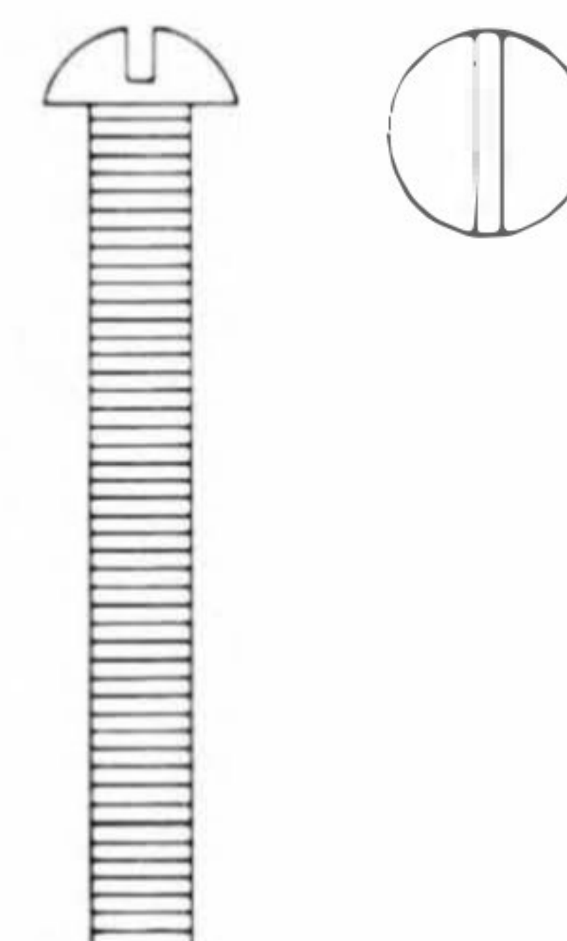
S-2563 10-32 x 1-1/2 Slotted Round Head Zinc Plated
