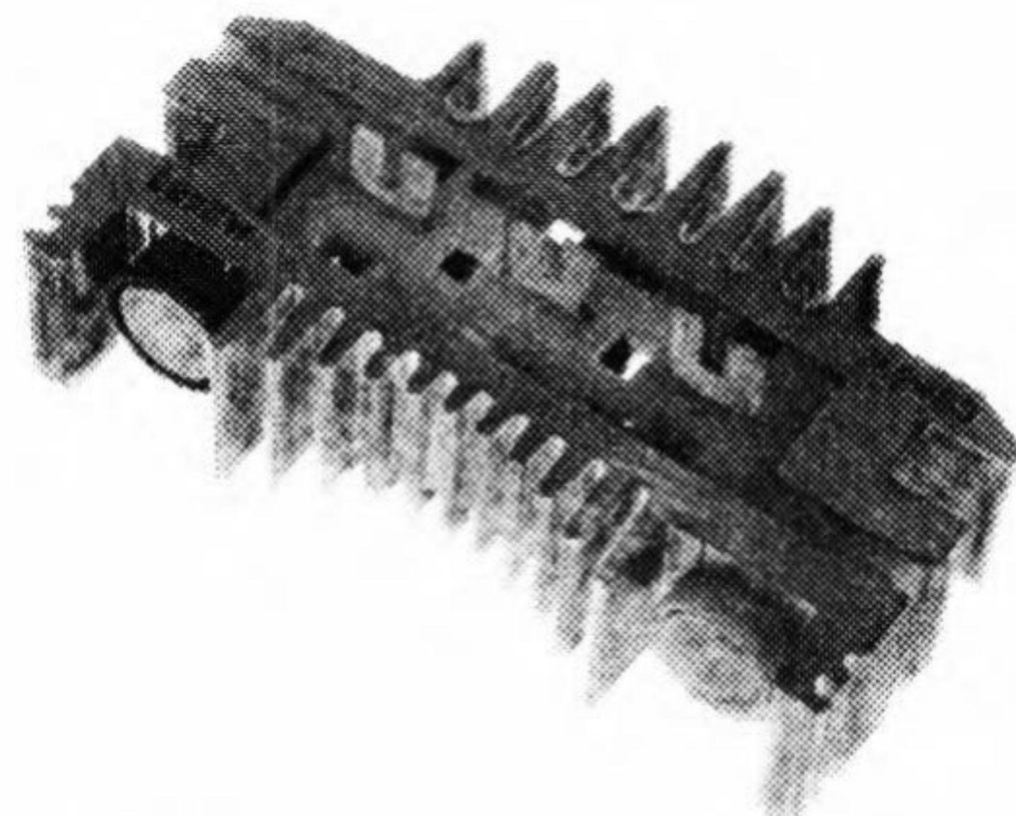
S-5379 Negative Ground for 50/60 amp Alternators REPLACES: 690971 APPLICATION: 1971-72 Peugeot 1969-83 Renault
