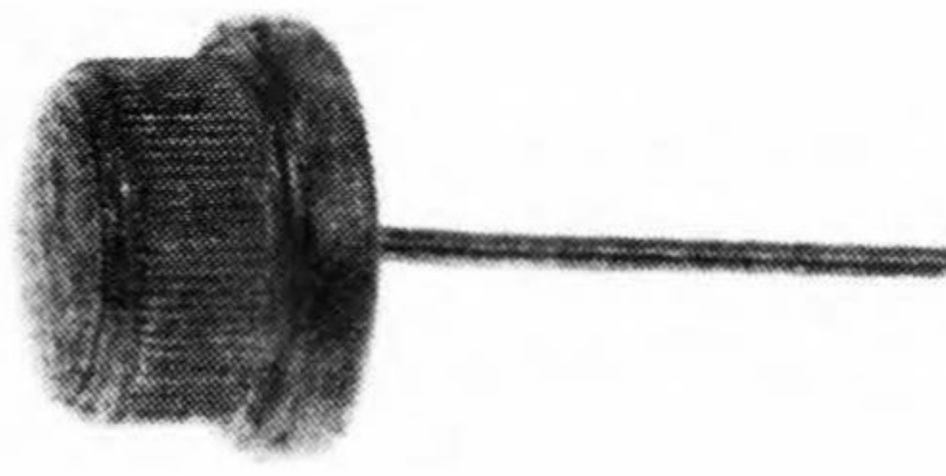
S-2403-P for CHRYSLER Positive; 25 amp; 50 volt 1/2" Can Type w/ Straight Stem w/ Eyelet REPLACES: 2098288
