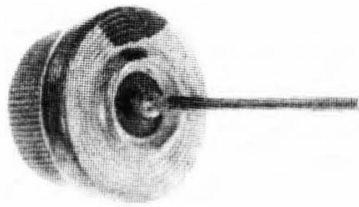
S-1430-N for AUTOMOTIVE Universal Diode Negative; 35 amp; 200 volt 1/2" Can Type w/ Straight Stem
