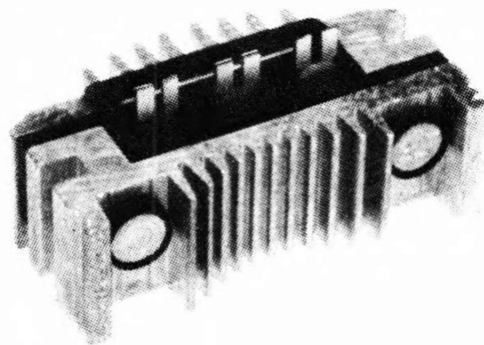
S-5380 for 70/75 amp Alternators REPLACES: 690972 APPLICATION: 1980-86 Renault/AMC
