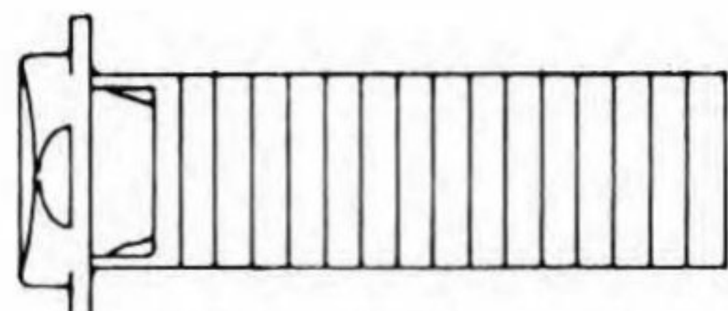
13111 3/8-16 x 1-3/16 Flat Oval Head Oval Crown Stepped Shoulder (Rectangular) Copper OEM No. 1927344
