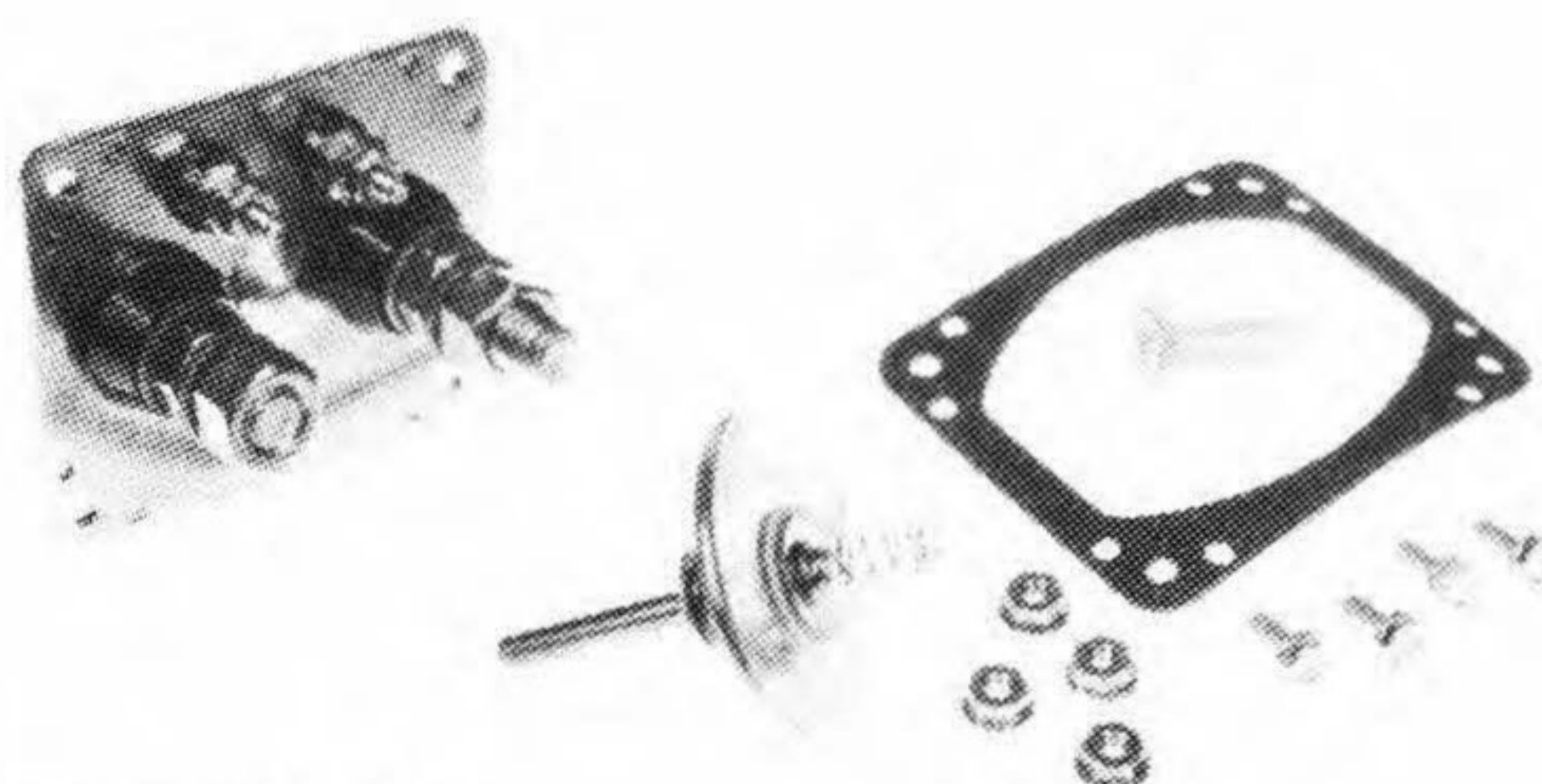
RK-5421 Repair Kit for Ace Solenoid Units 15556 12 Volt
