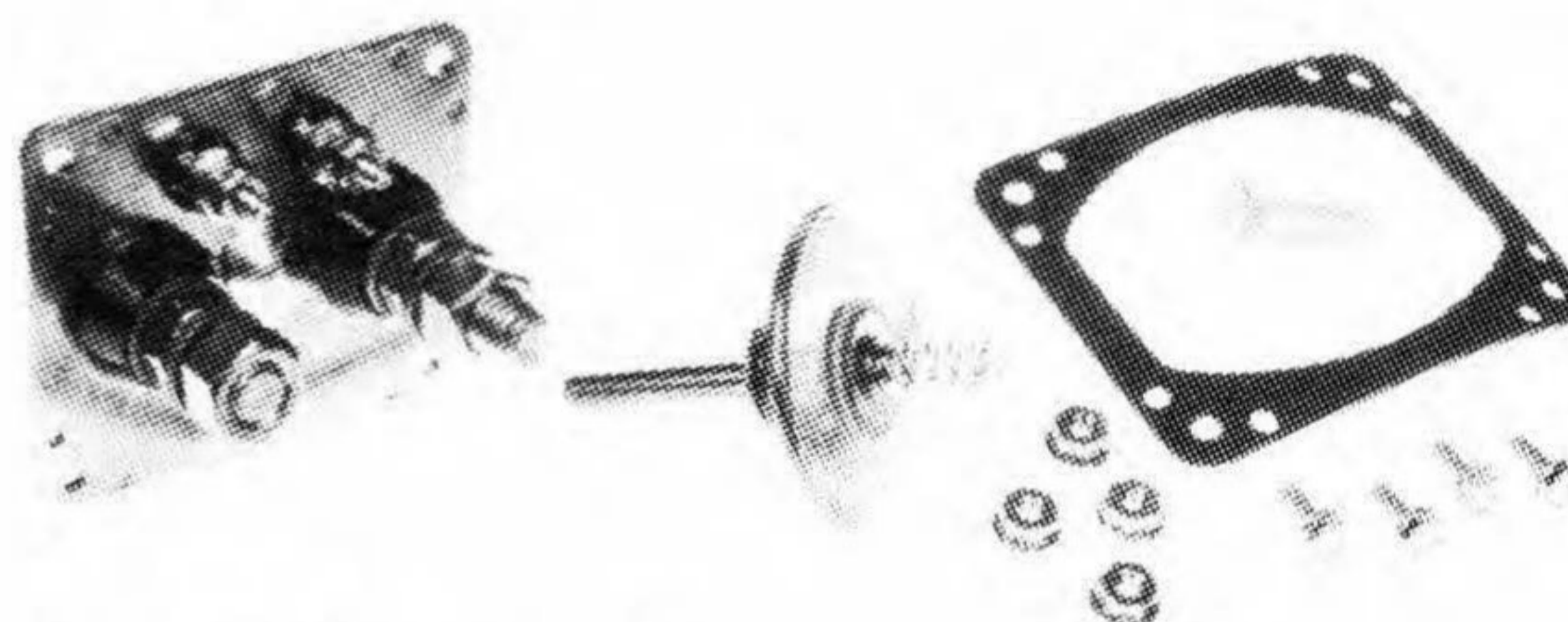
RK-5422 Repair Kit for Ace Solenoid Unit 15559 24 & 32 Volt can be used for OEM No. 1115558, 564 & 566
