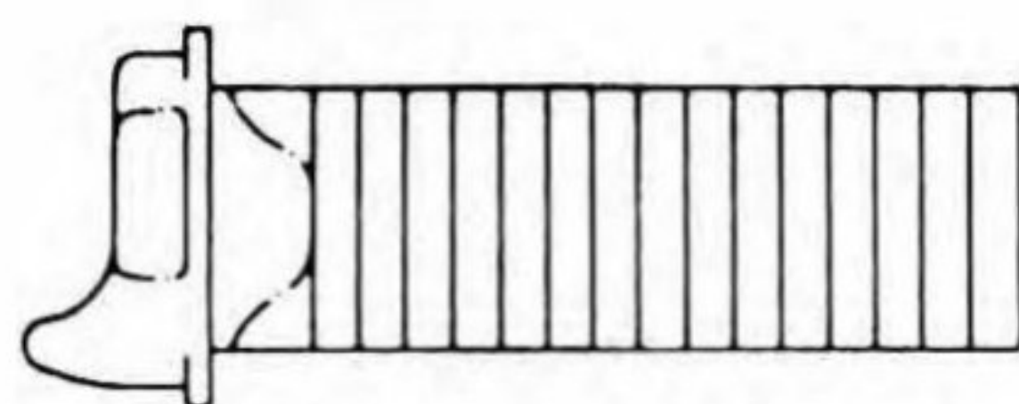
13242 3/8-16 x 1-1/8 Flat Oval Head Square Crown with Raised Side Stepped Shoulder (Rectangular) Copper
