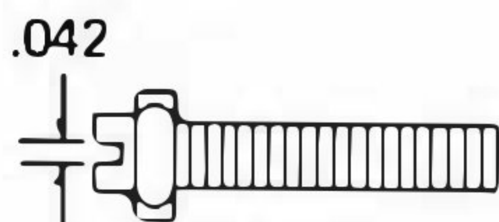
S-2490 8-32 x 3/4 Square Flat Head Cylindrical Crown Zinc Plated OEM No. 2098628
