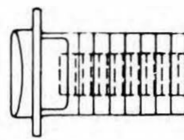
13132 3/8-16 x 5/8 Tapped 10-32 Shank Flat Oval Head Stepped Shoulder (Rectangular) Copper
