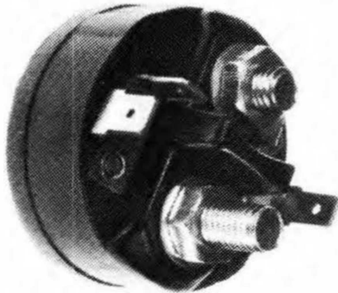
14211 Cap Assembly for Bosch Solenoid Units 0-331-302-004, 005, 008, 011, 021, 024, 025, 028, 030, 031, 032, 045, 074, 0-331-302-034, 071 Replaces: 1-330-516-001, 012, 015, 030, 033, 1-330-520-101, 161 6 & 12 Volt Starting Systems
