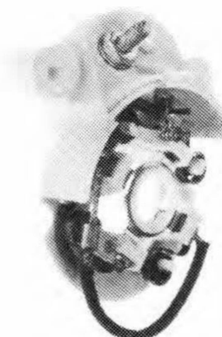
S-2532-C Brush Holder Assembly with Battery Terminal & Hardware
