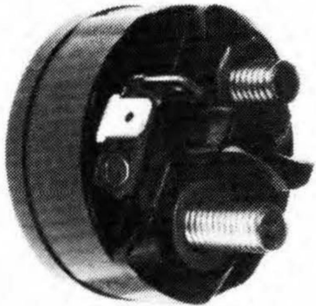
14201 Cap Assembly for ACE Solenoid Unit 14460 for Bosch Solenoid Units 0-331-302-034 & 071 Replaces: 1-330-516-001, 030 & 034 12 Volt Starting Systems
