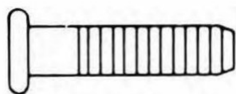
13182 M5 x 0.8 x 20.1 mm Circular Flat Head Square Shoulder Copper Plated
