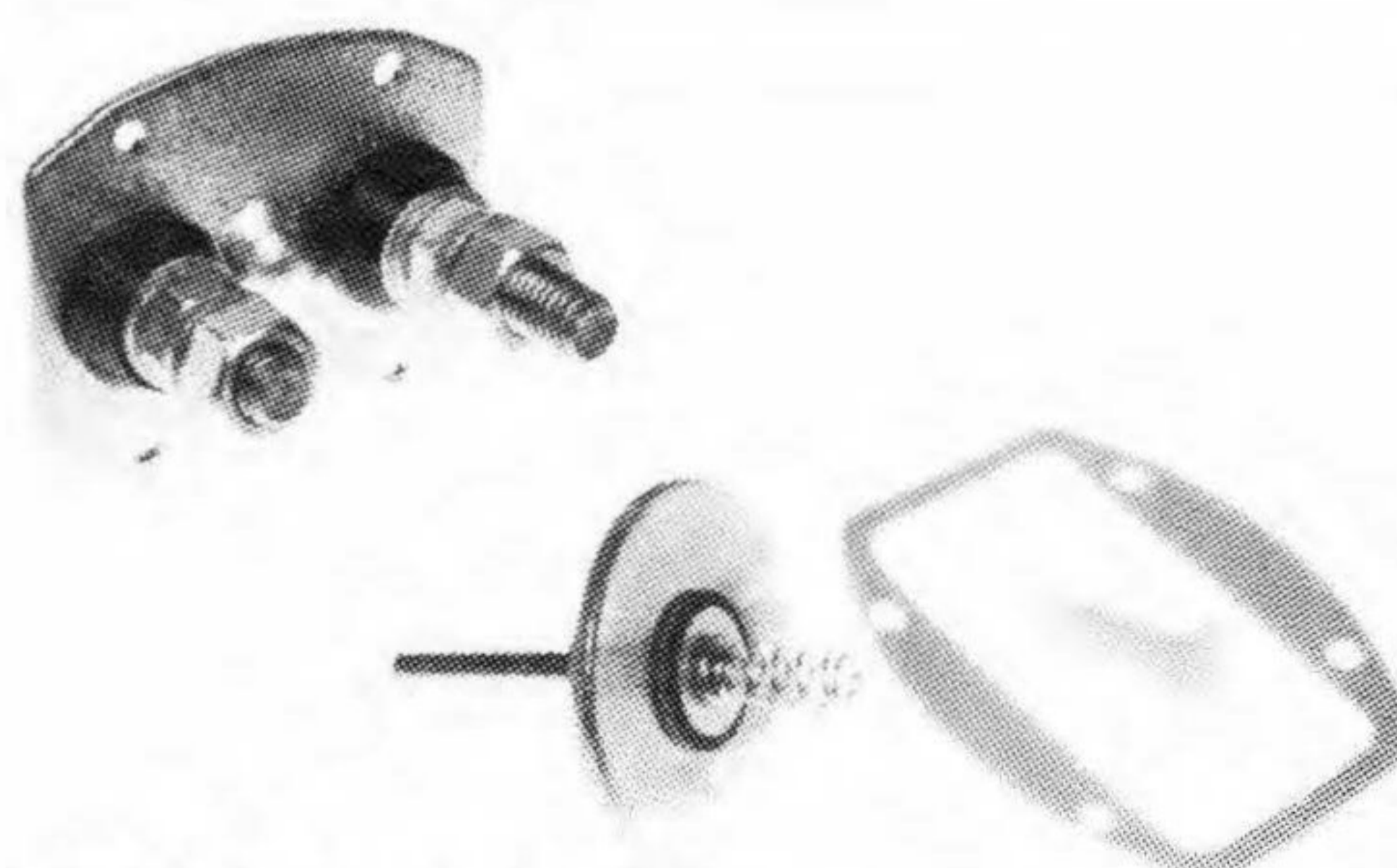
RK-5416 Repair Kit for Ace Solenoid Units 19851 & 19879
