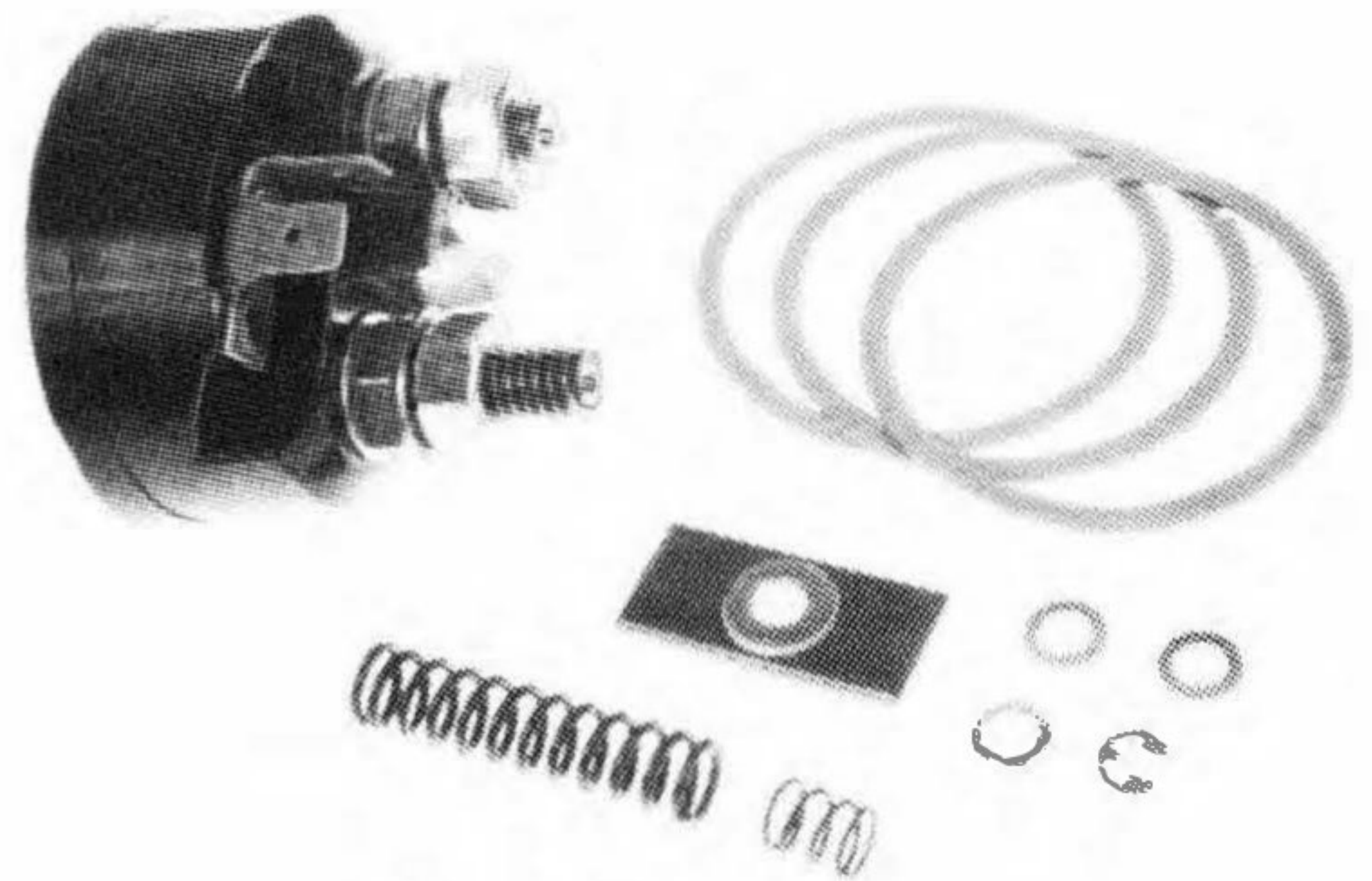
14203 Repair Kit for ACE Solenoid Unit 14459 for Bosch Solenoid Units 0-331-302-004, 005, 008, 011, 021, 025, 028, 030, 031 & 045 Replaces: 1-330-516-012, 015, 030, 033, 1-330-520-101 & 161 6 Volt Starting Systems
