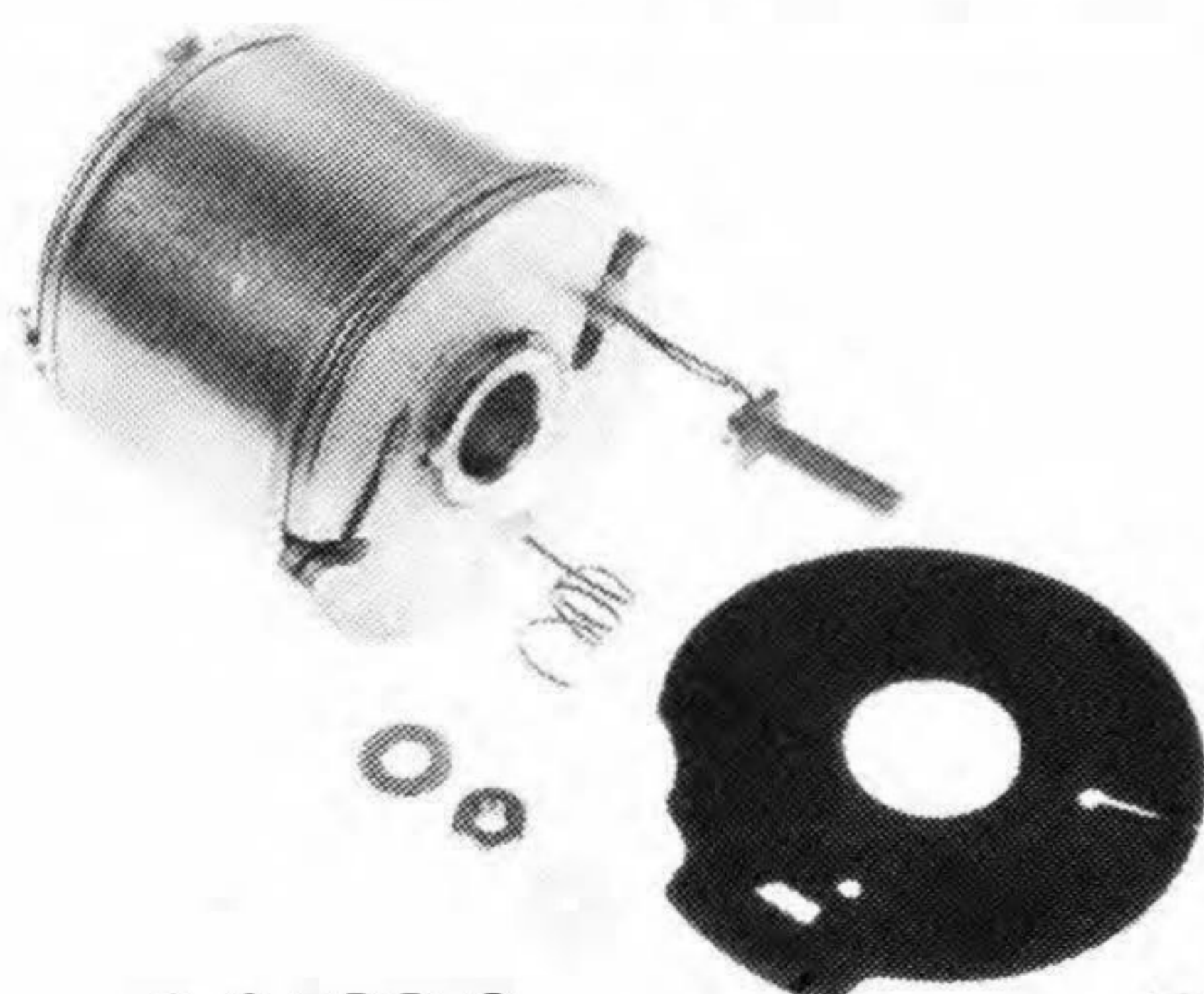
S-2488-C Coil Assembly with Switch Terminal, Hardware, & Gasket OEM No. 2275554
