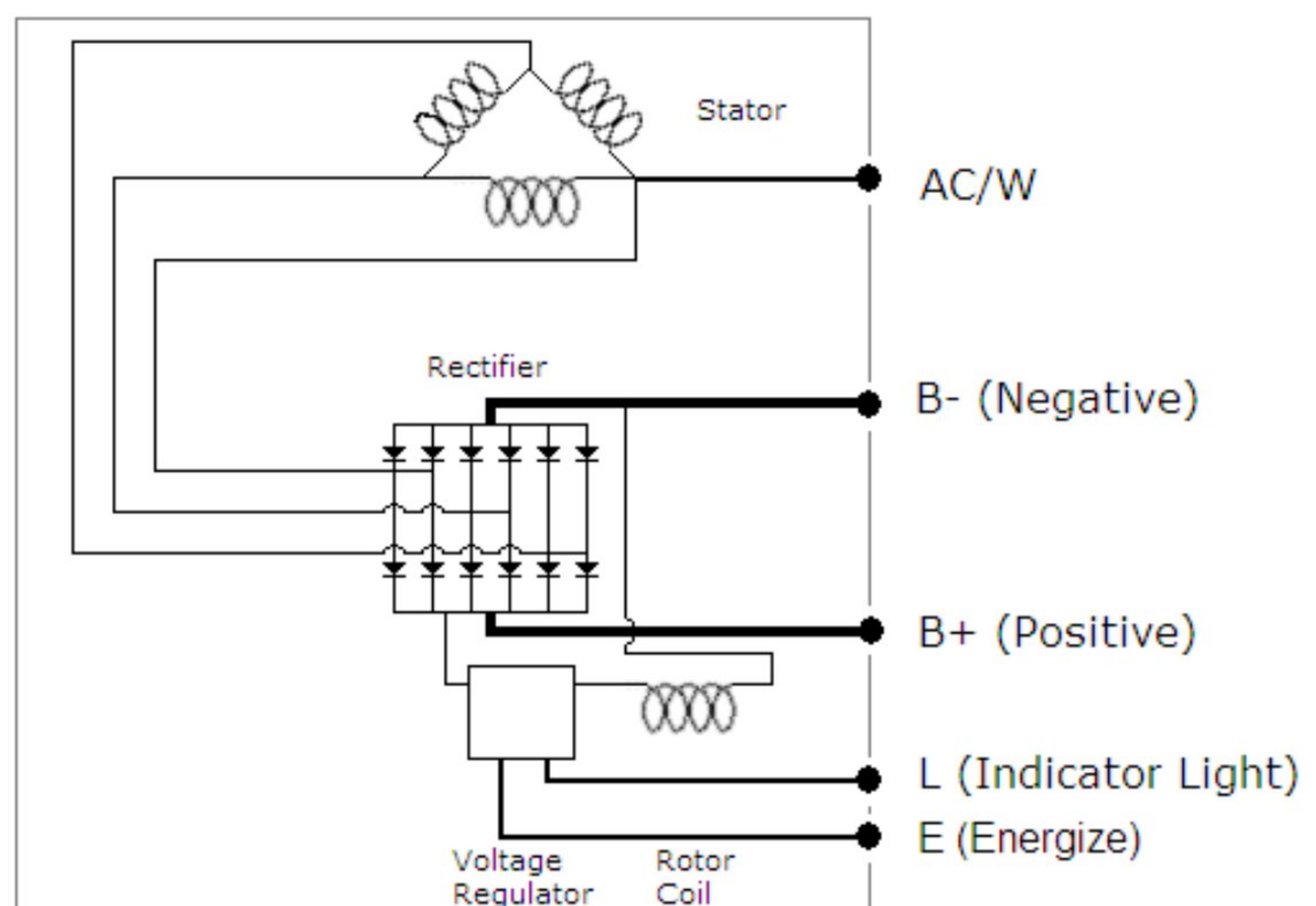
Alternator Schematic
